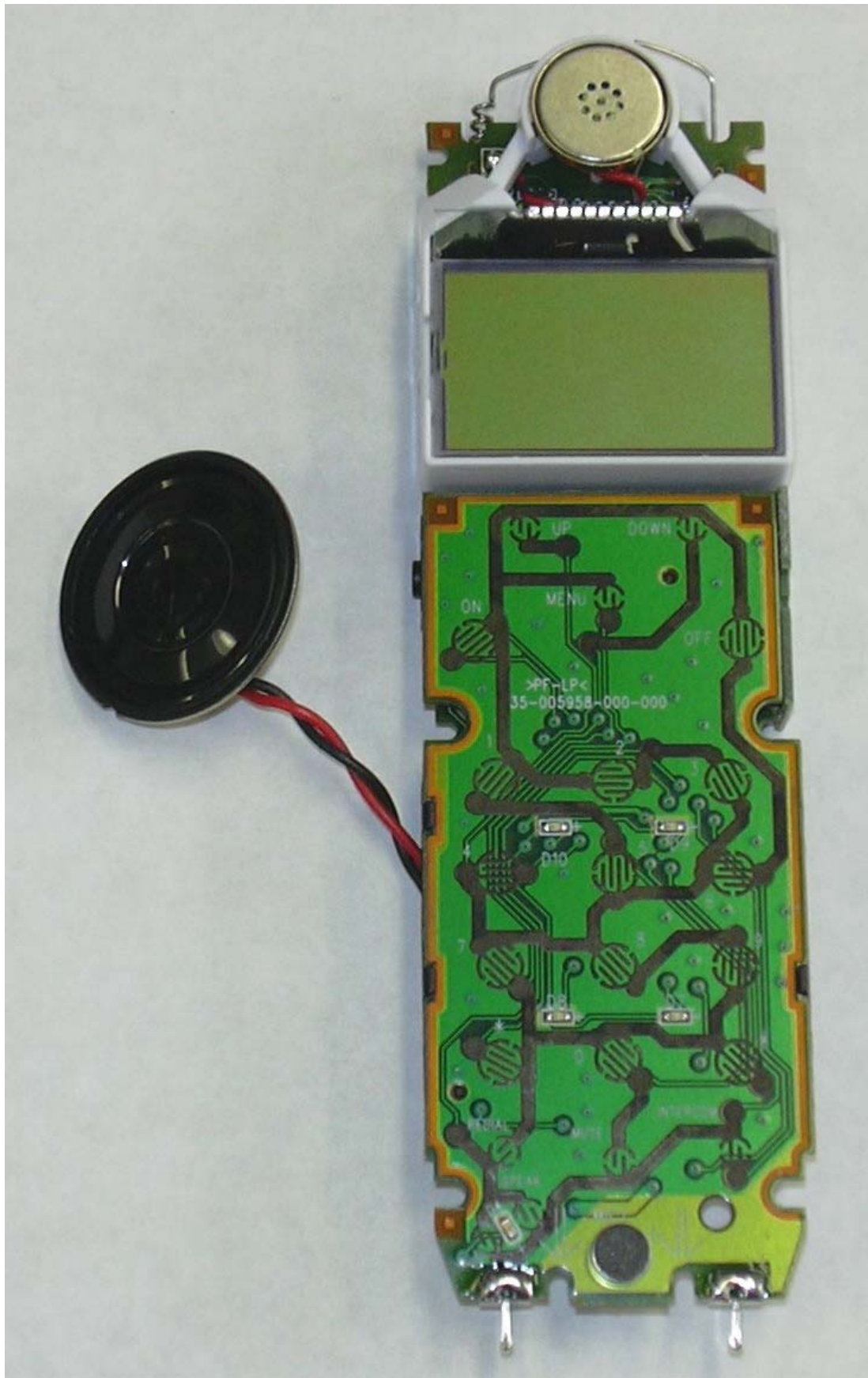
VTech I6765 Handset PCB
