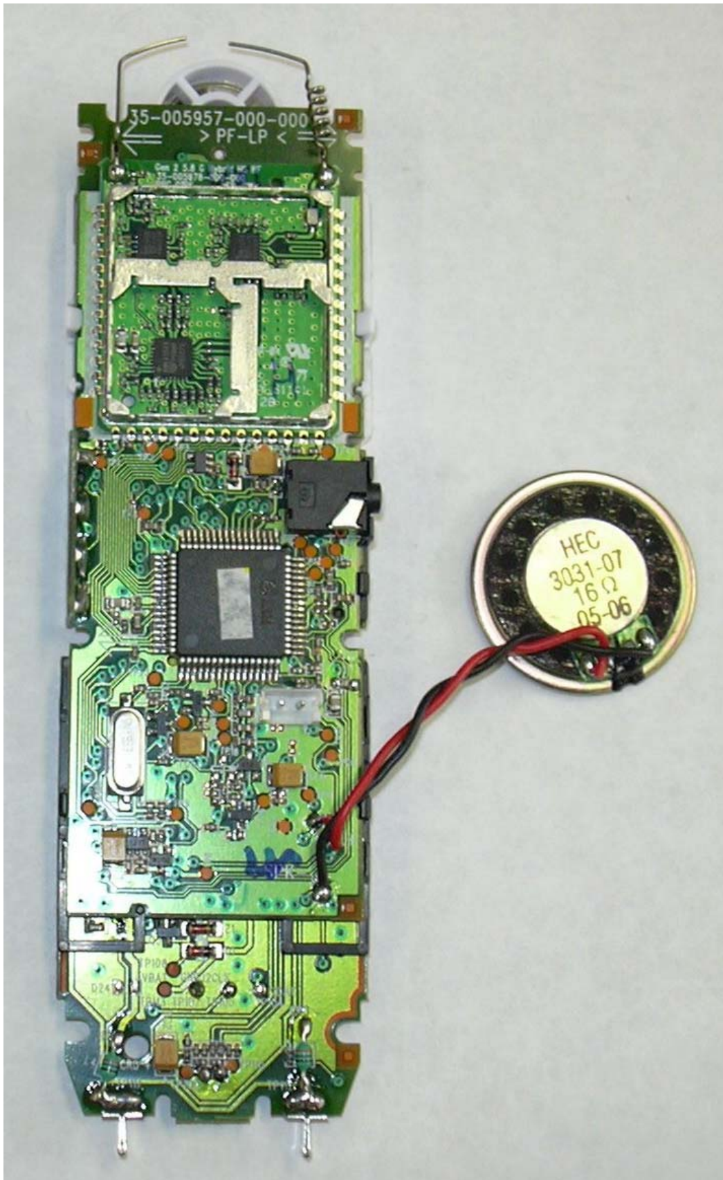
VTech i6765 Handset PCB
