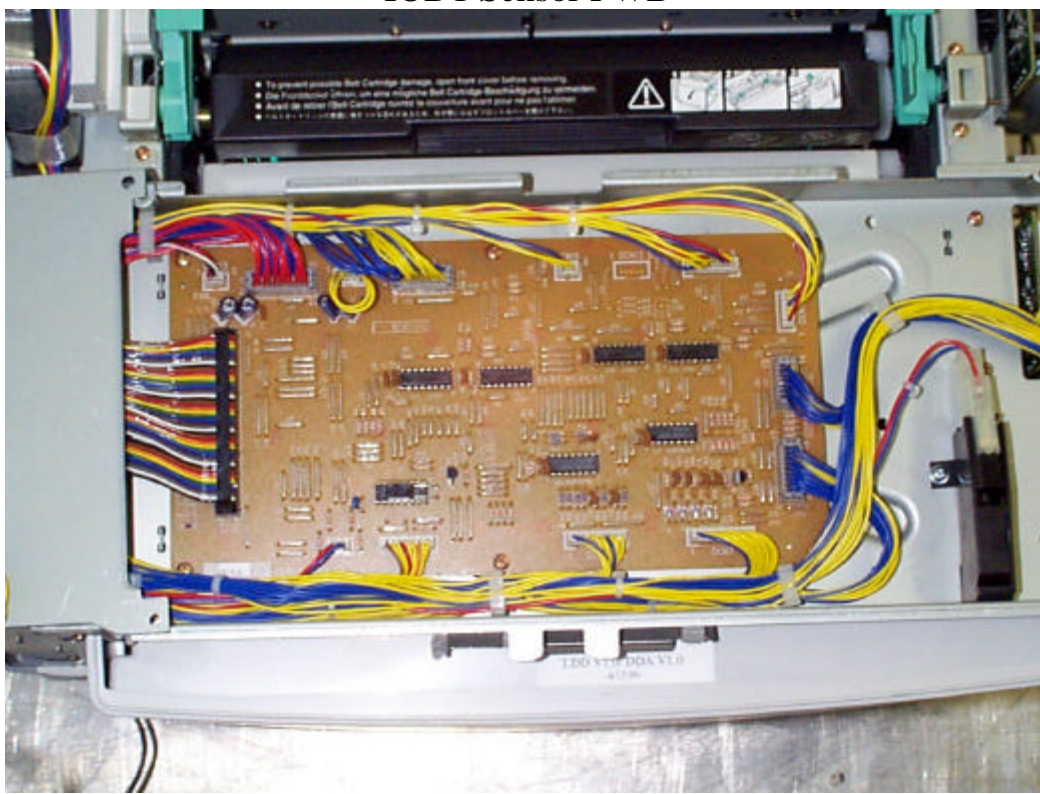
IOD1 Sensor PWB
