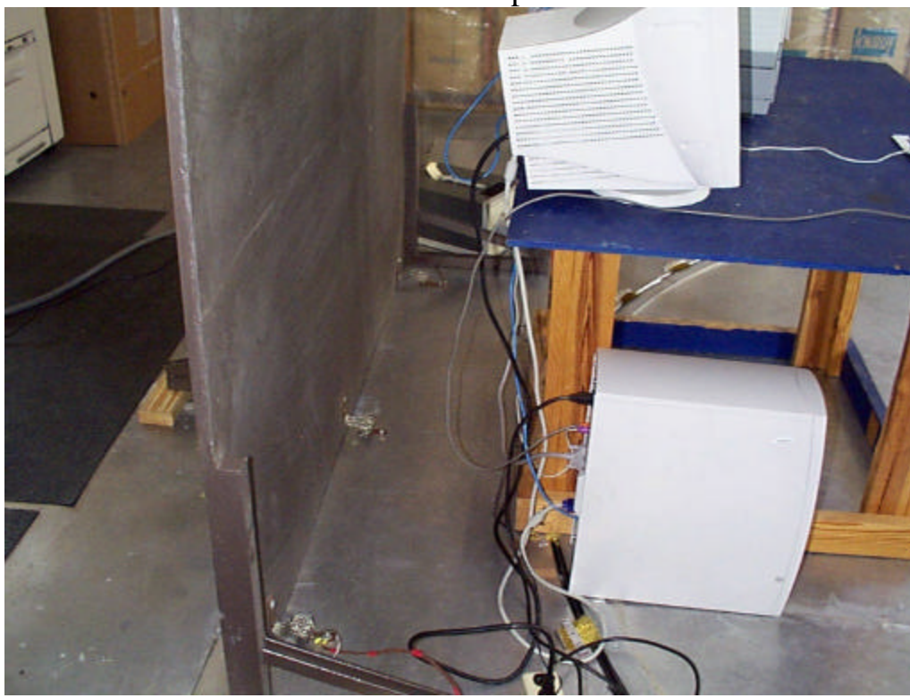
Conducted Test Setup - Left View
