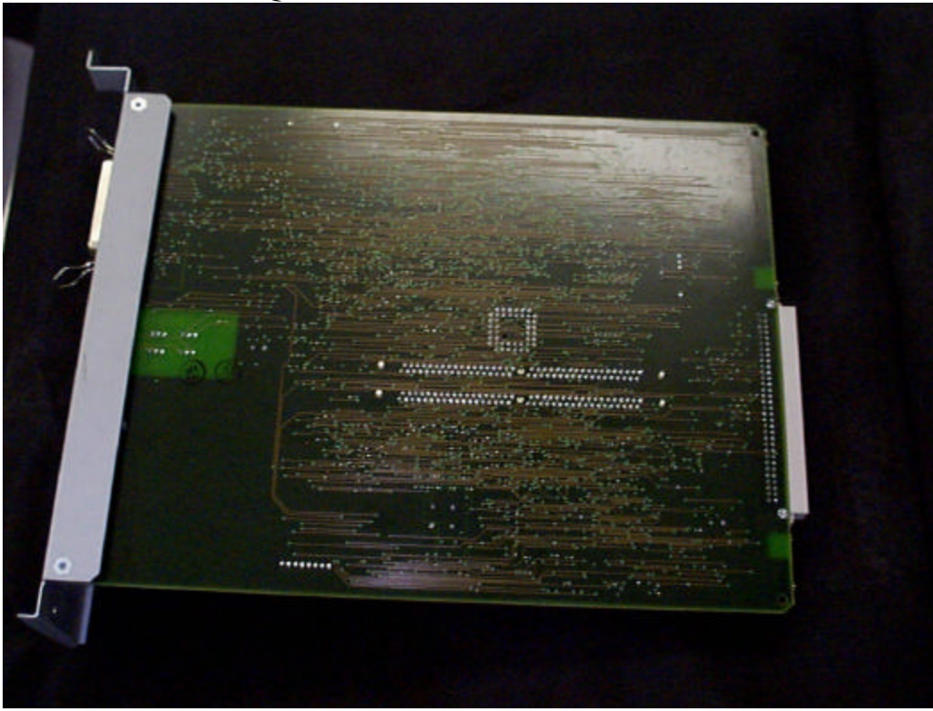
QMS Controller - Bottom View
