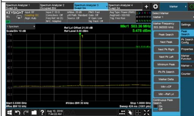
Mid CH-Spurious Emission-Low
