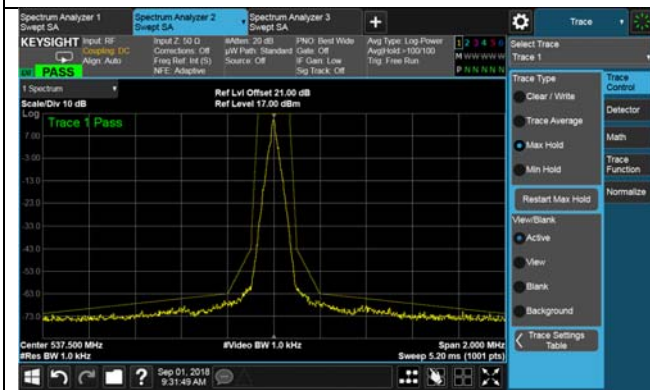
High Channel, Mask
