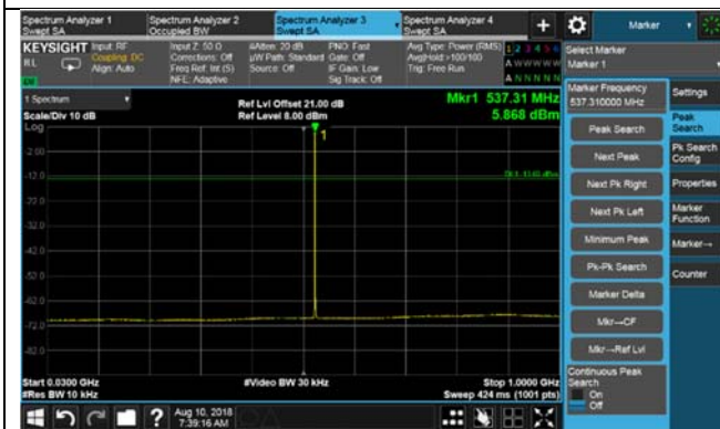
High CH-Spurious Emission-Low
