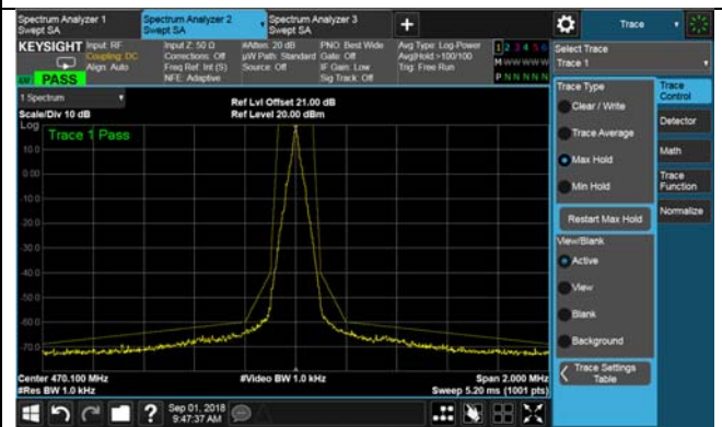
Low Channel, Mask
