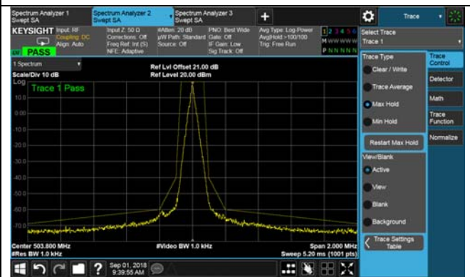
Middle Channel, Mask
