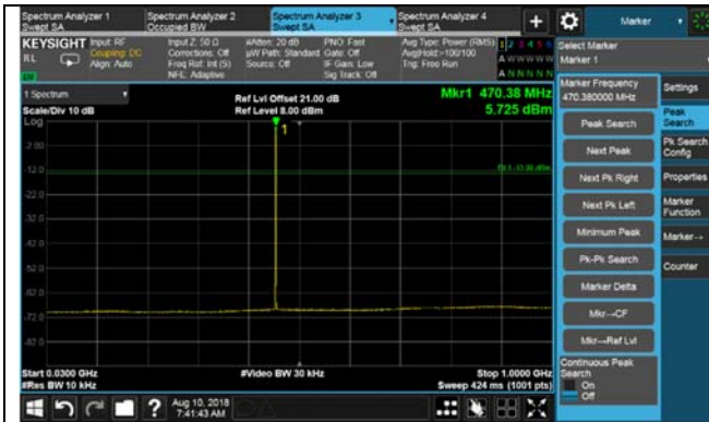
Low CH-Spurious Emission-Low
