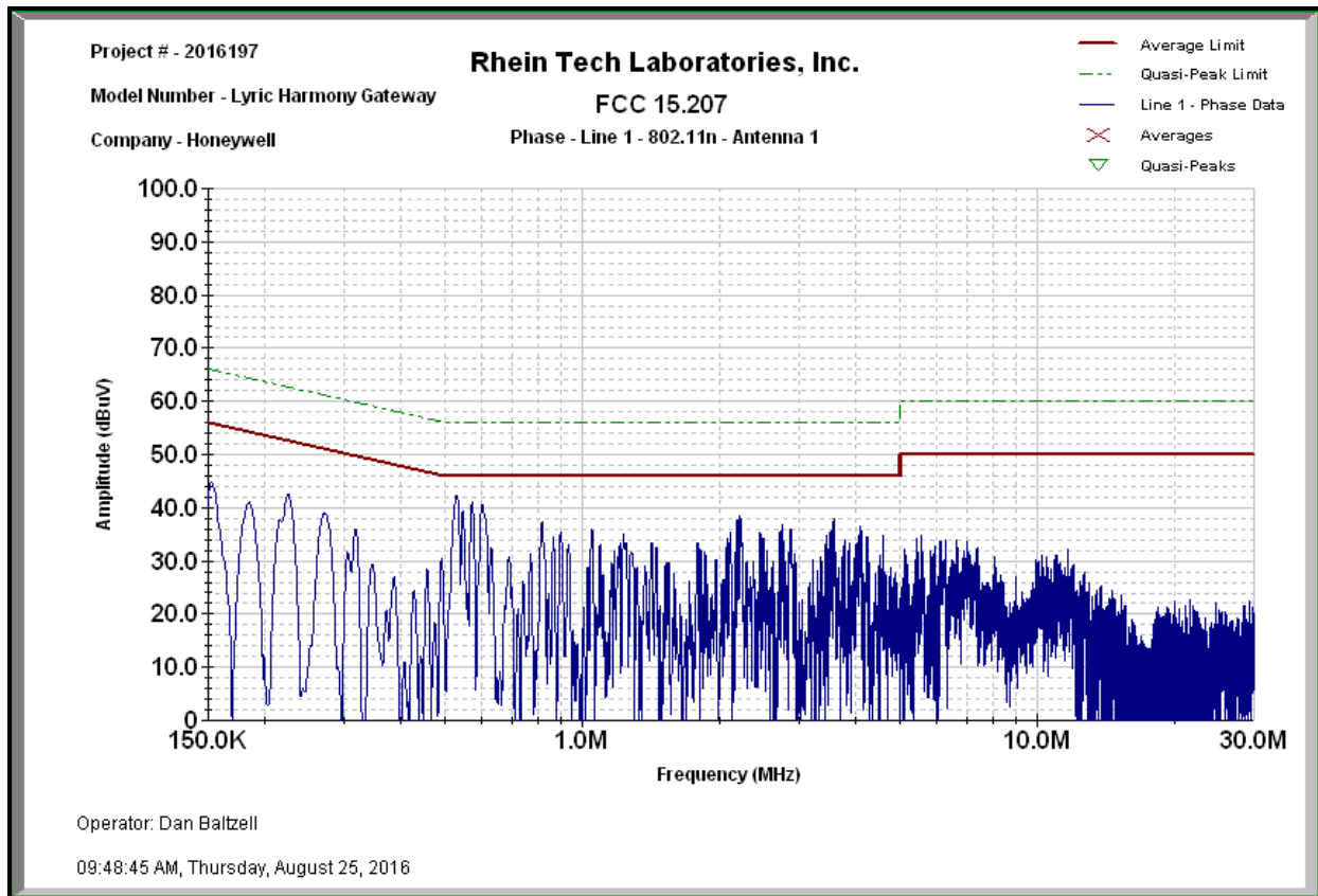
Plot 6-11: Conducted Emissions (Phase Side); Mode: Transmit - 802.11n (Antenna #1)
