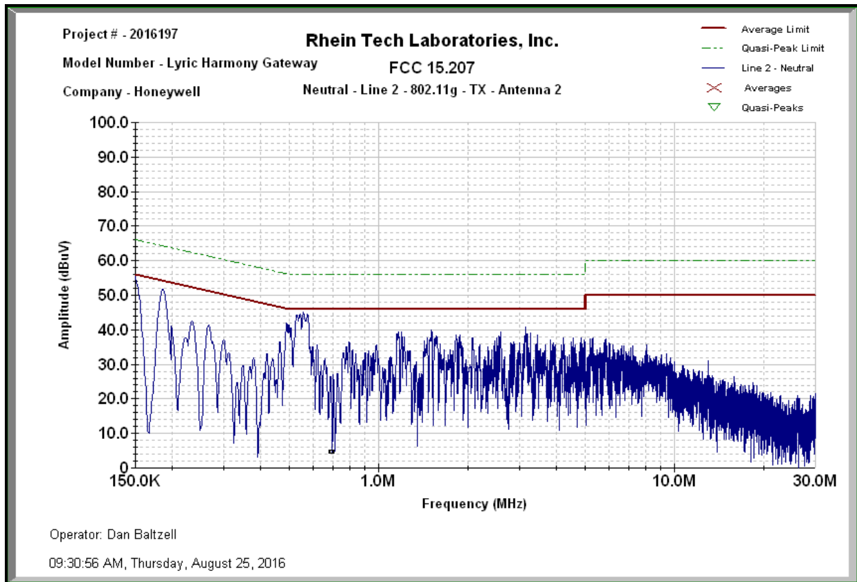
Plot 6-10: Conducted Emissions (Neutral Side); Mode: Transmit - 802.11g (Antenna #2)
