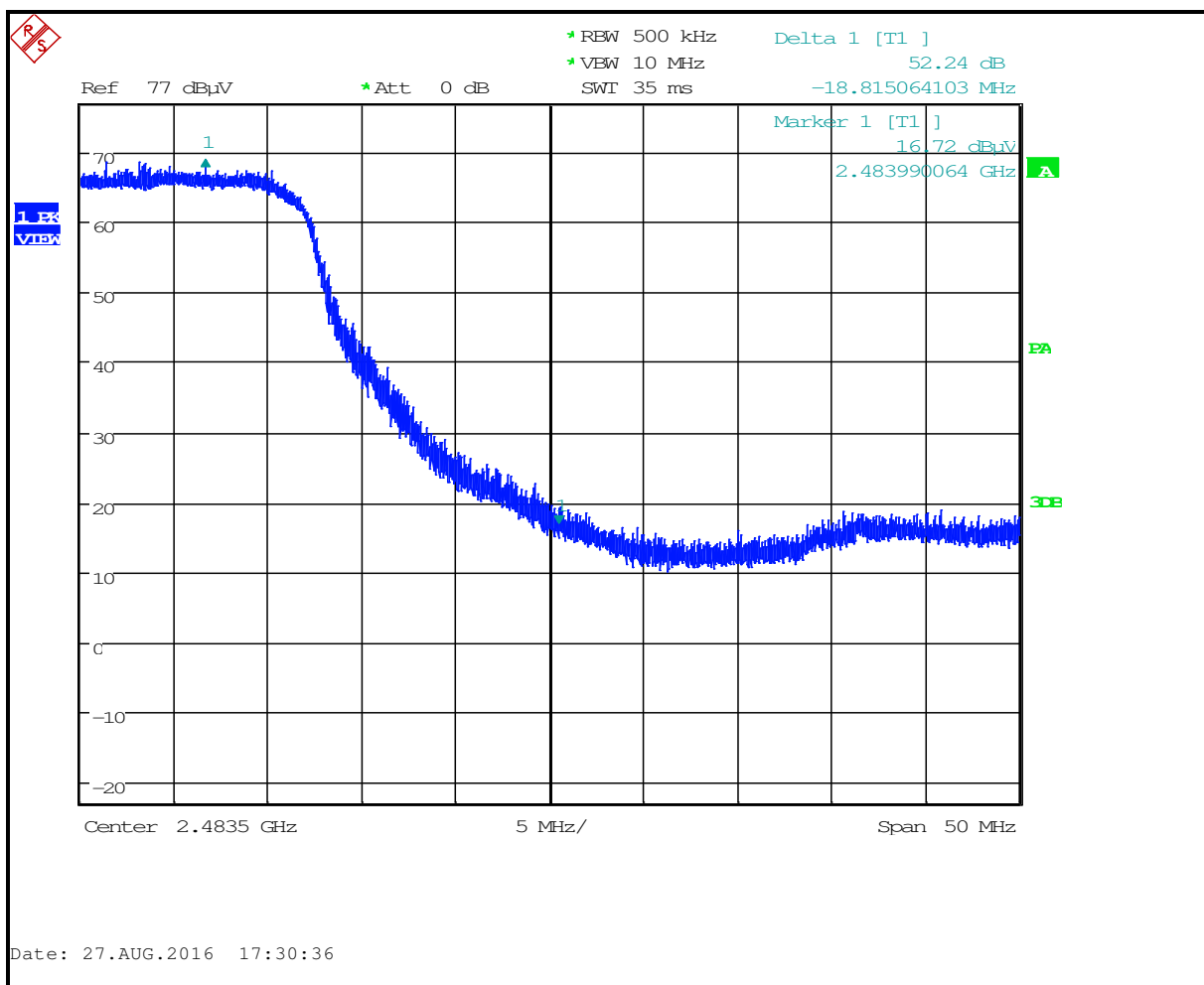
Plot 4-12: Upper Band Edge - 802.11n (Antenna #2)
