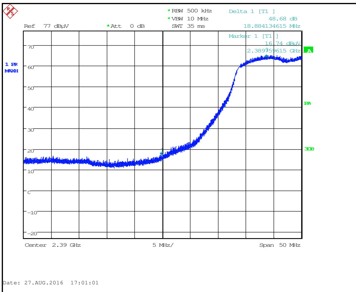
Plot 4-11: Lower Band Edge – 802.11n (Antenna #2)
