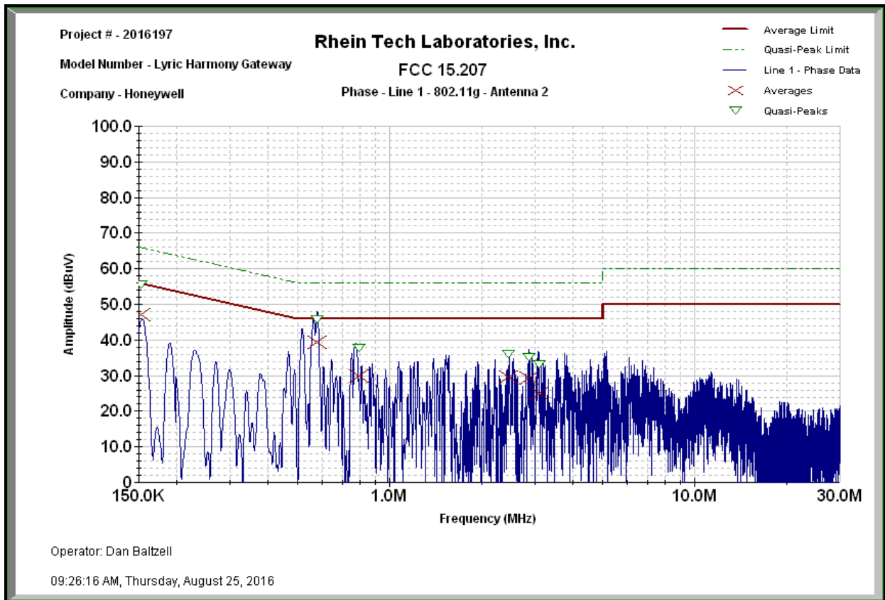
Plot 6-9: Conducted Emissions (Phase Side); Mode: Transmit - 802.11g (Antenna #2)
