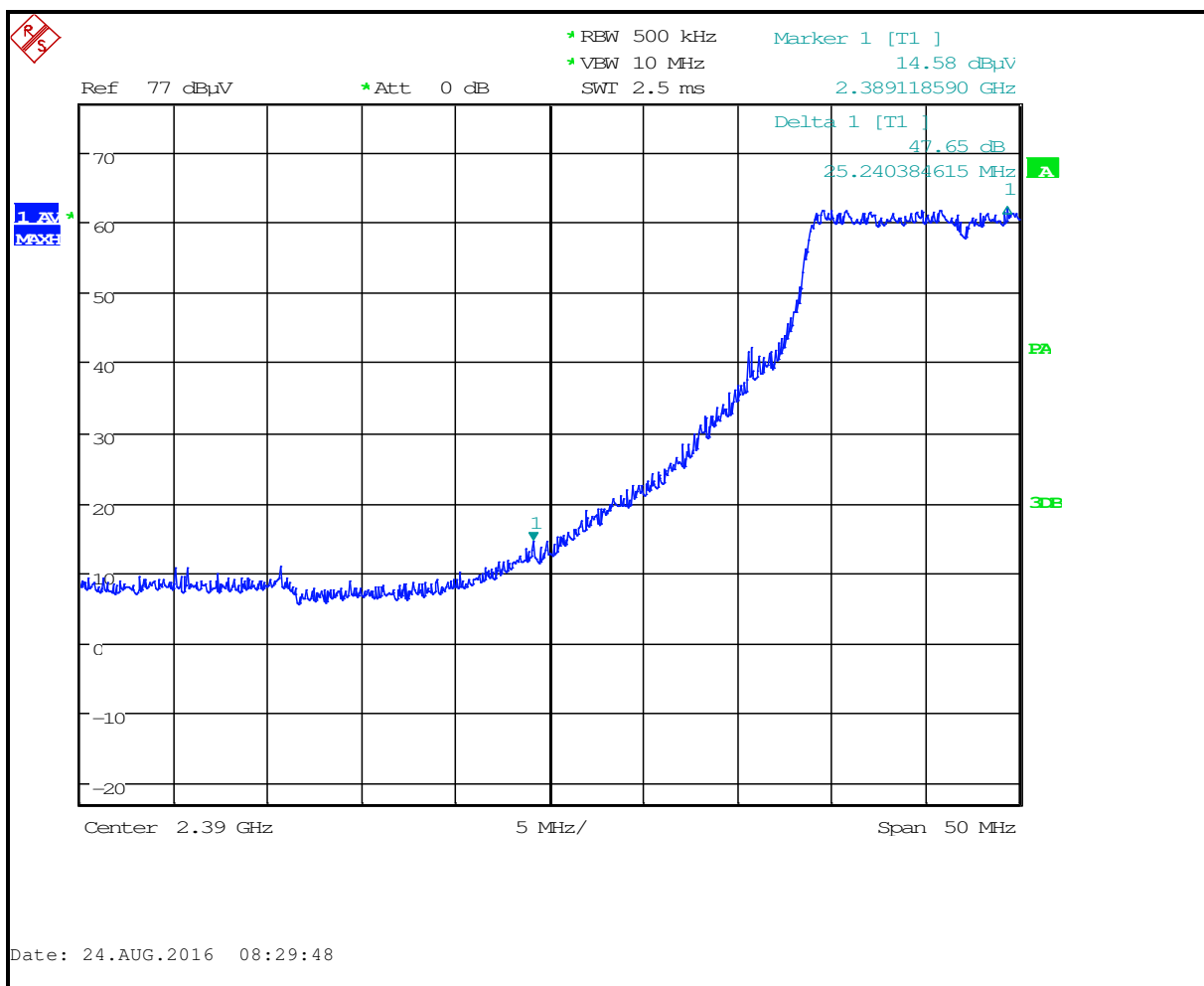
Plot 4-3: Lower Band Edge – 802.11g (Antenna #1)
