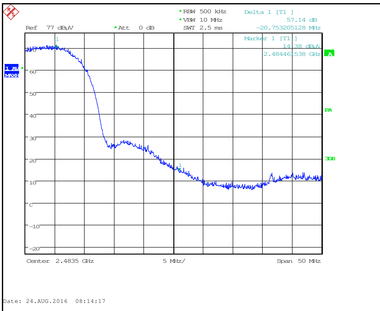
Plot 4-2: Upper Band Edge - 802.11b (Antenna #1)
