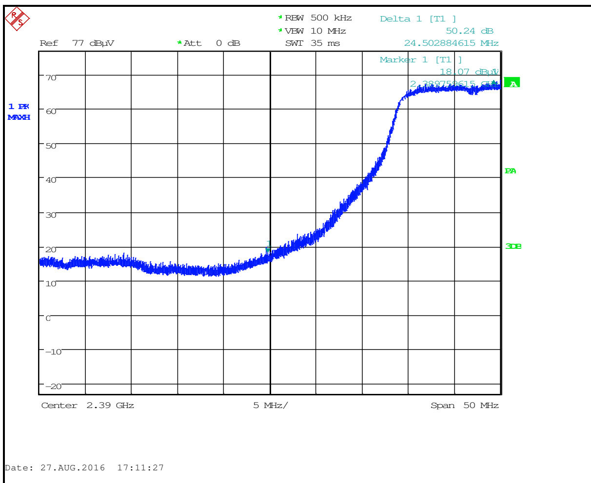
Plot 4-9: Lower Band Edge – 802.11g (Antenna #2)
