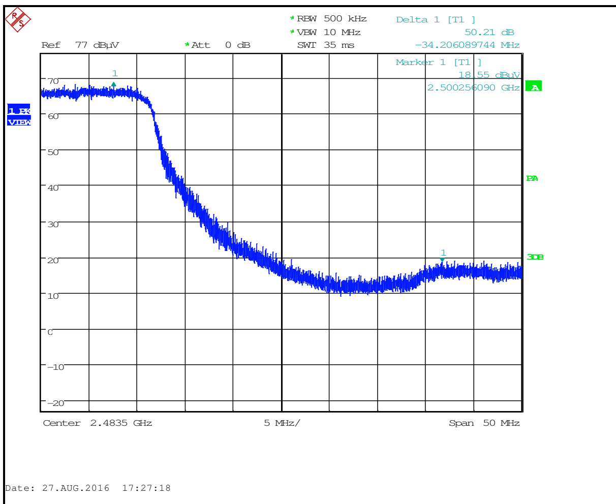
Plot 4-10: Upper Band Edge - 802.11g (Antenna #2)
