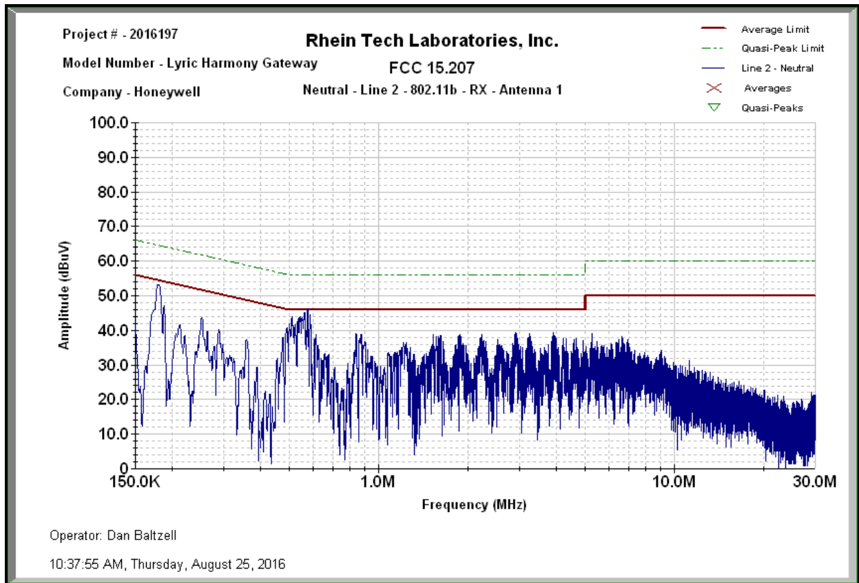
Plot 6-3: Conducted Emissions (Neutral Side); Mode: Receive - 802.11b (Antenna #1)
