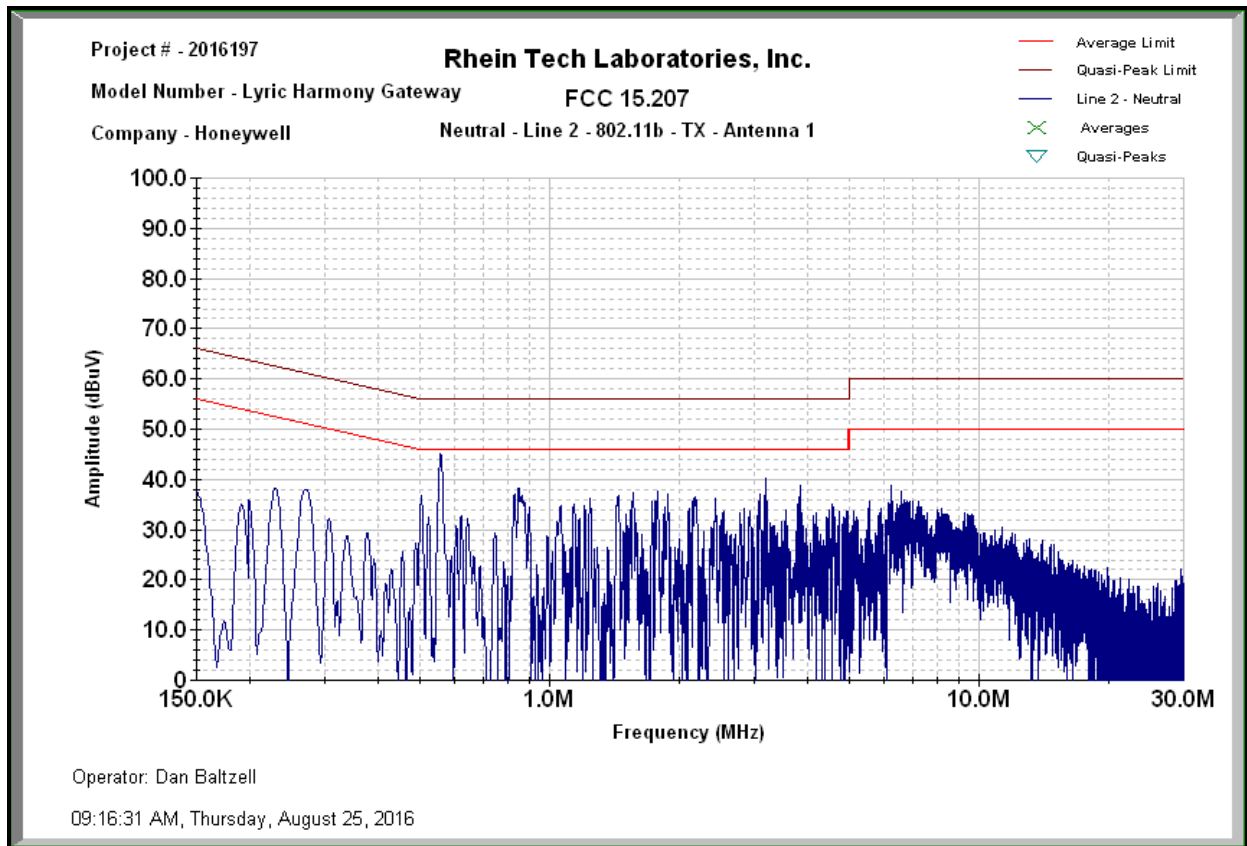
Plot 6-2: Conducted Emissions (Neutral Side); Mode: Transmit - 802.11b (Antenna #1)
