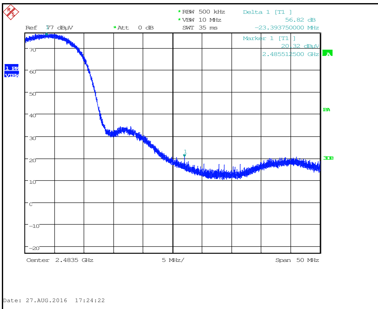
Plot 4-8: Upper Band Edge - 802.11b (Antenna #2)
