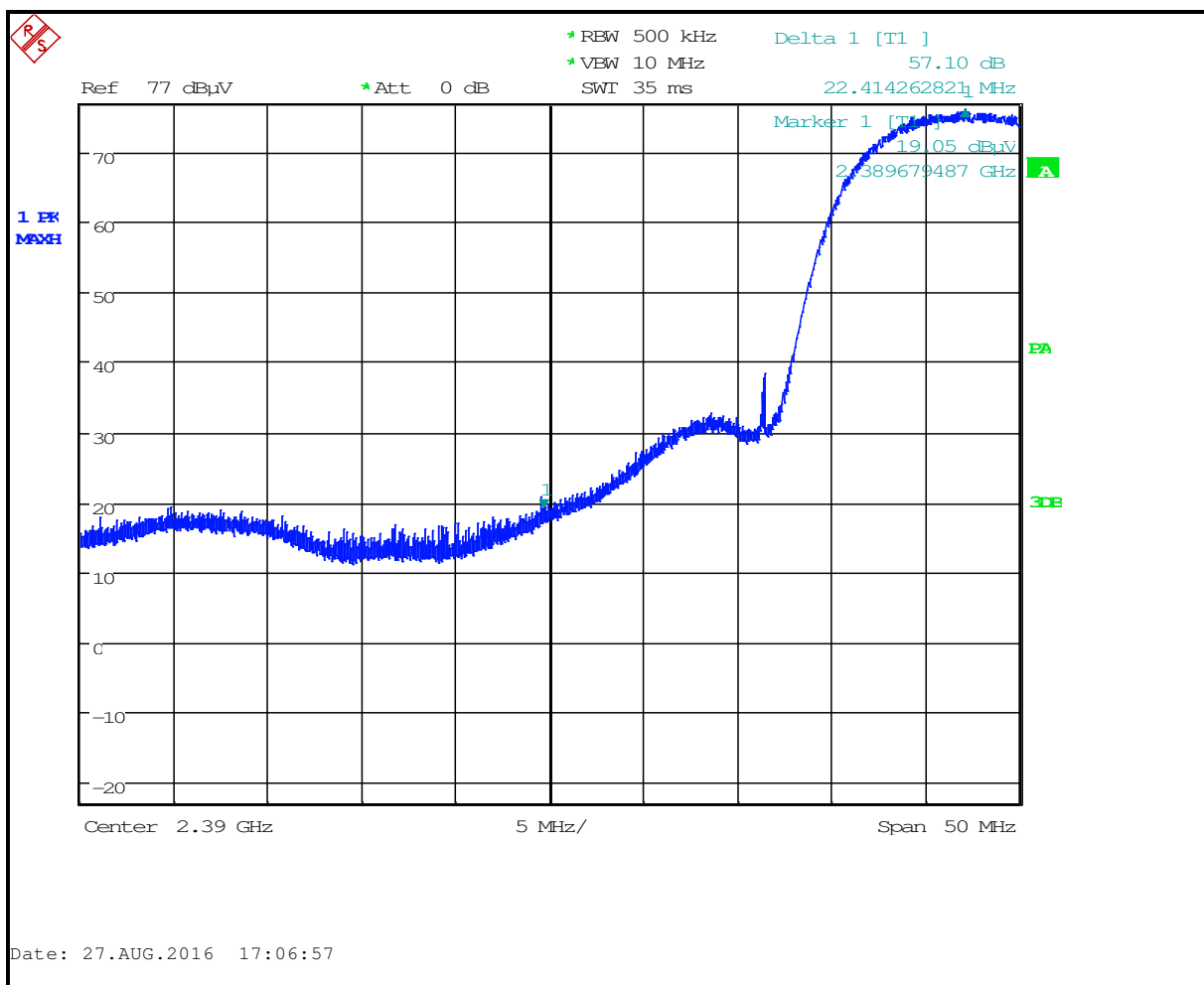
Plot 4-7: Lower Band Edge – 802.11b (Antenna #2)
