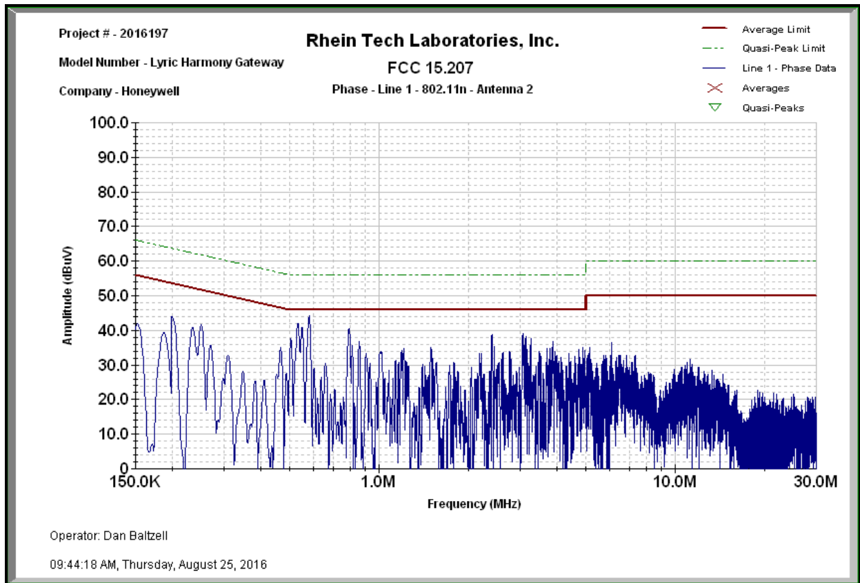
Plot 6-13: Conducted Emissions (Phase Side); Mode: Transmit - 802.11n (Antenna #2)
