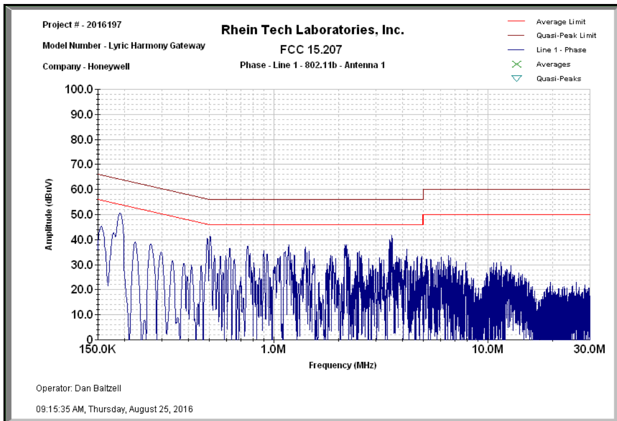
Plot 6-1: Conducted Emissions (Phase Side); Mode: Transmit - 802.11b (Antenna #1)
