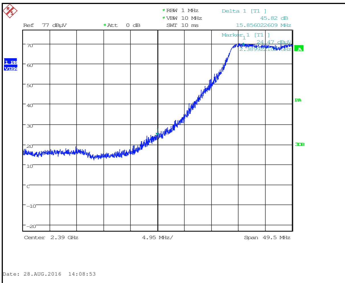
Plot 4-5: Lower Band Edge – 802.11n (Antenna #1)
