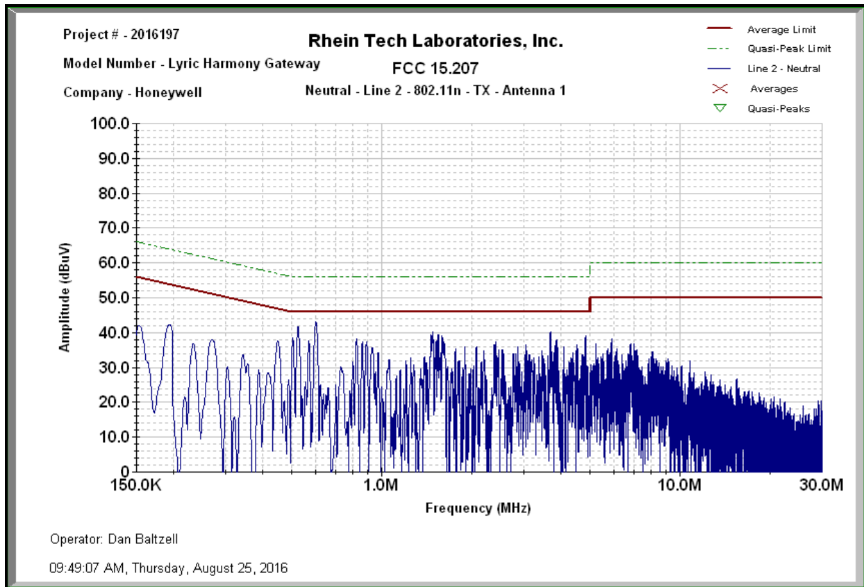
Plot 6-12: Conducted Emissions (Neutral Side); Mode: Transmit - 802.11n (Antenna #1)
