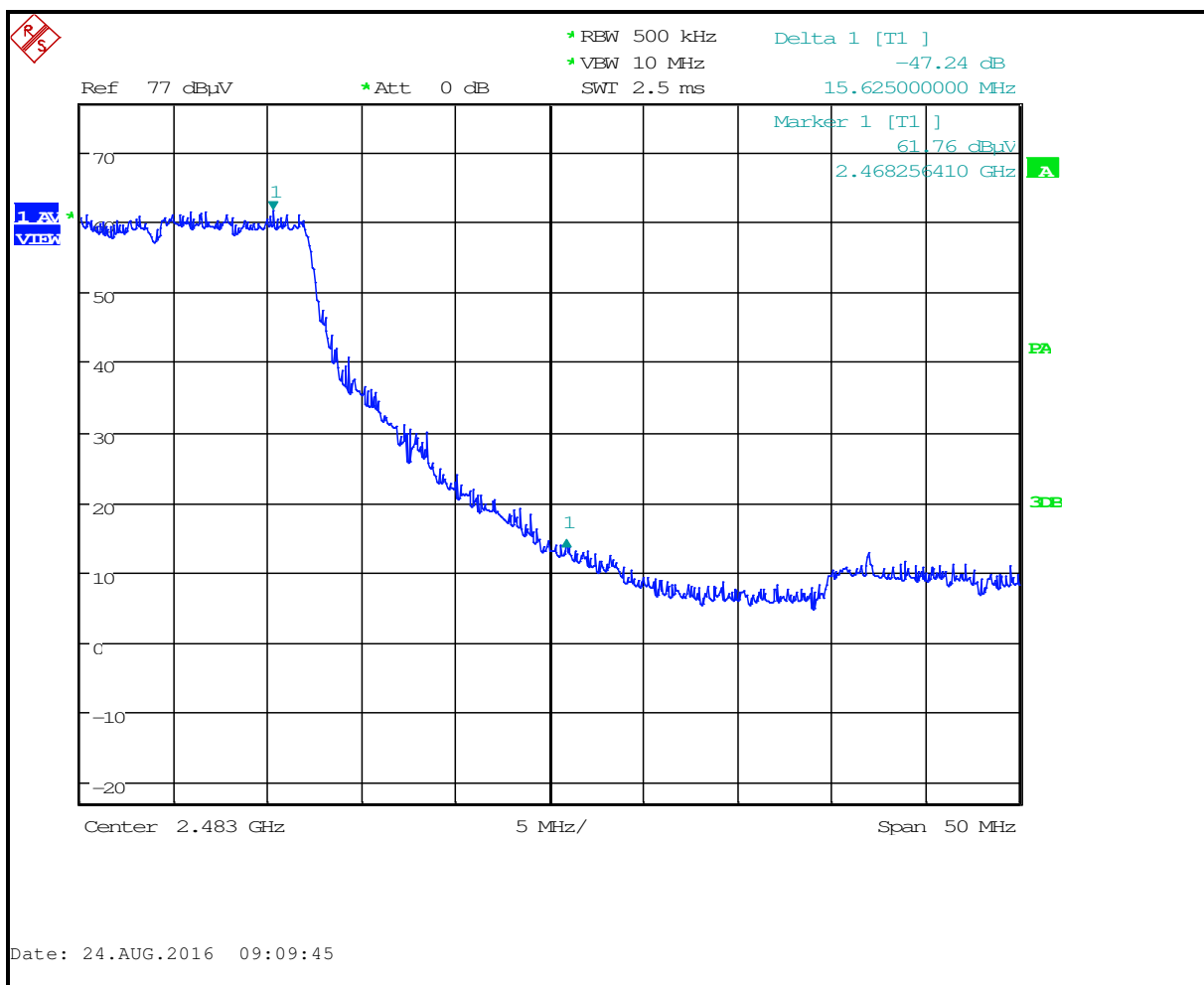
Plot 4-4: Upper Band Edge - 802.11g (Antenna #1)
