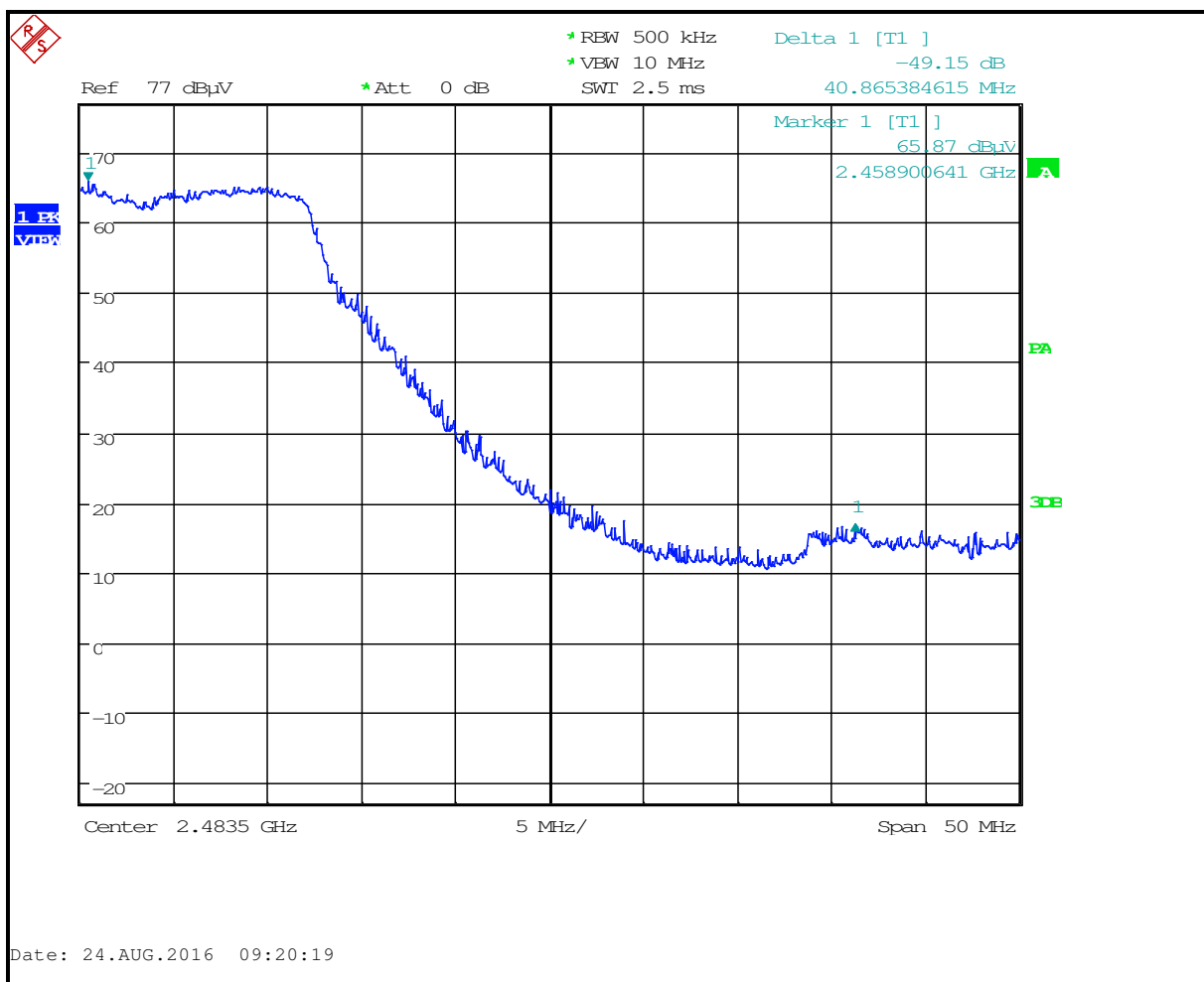
Plot 4-6: Upper Band Edge - 802.11n (Antenna #1)
