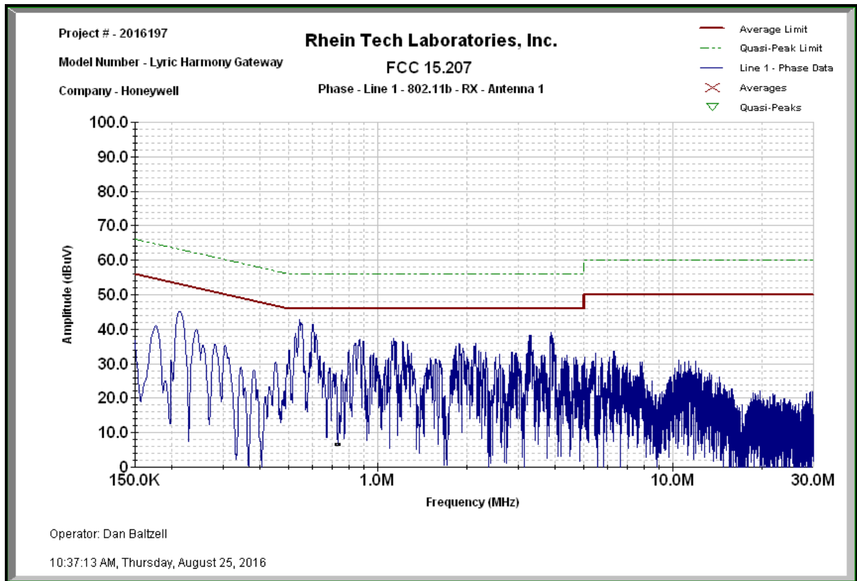
Plot 6-4: Conducted Emissions (Phase Side); Mode: Receive - 802.11b (Antenna #1)
