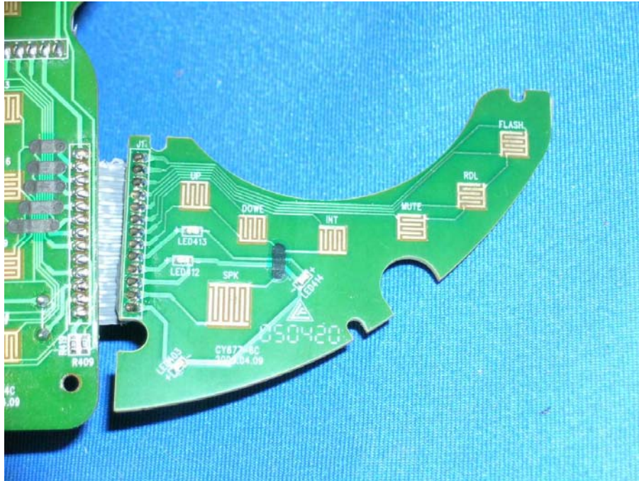
Base Keypad and LCD Display front side (View 2)
