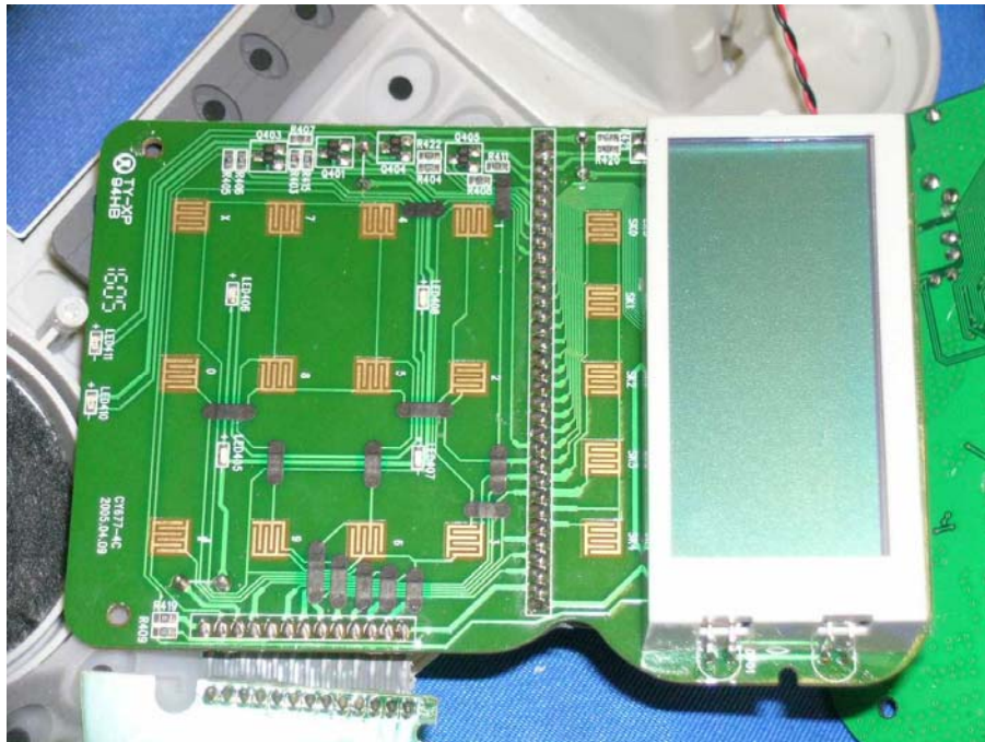
Base Keypad and LCD Display front side (View 1)
