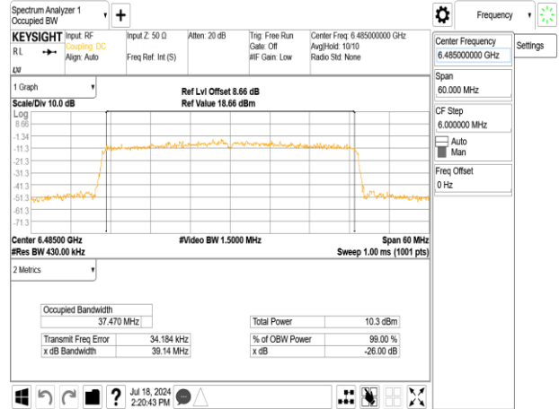
802.11ax_40MHz_Chain1_6485MHz_RU242_62
