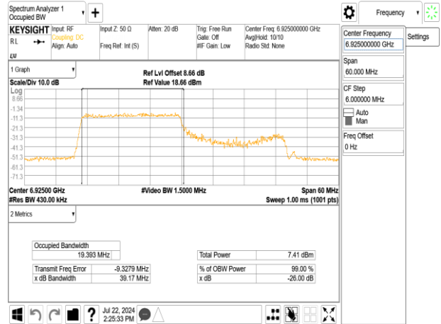
802.11ax_40MHz_Chain0_6925MHz_RU242_61
