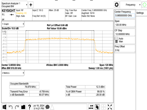
802.11ax_80MHz_Chain0_5985MHz_RU484_65
