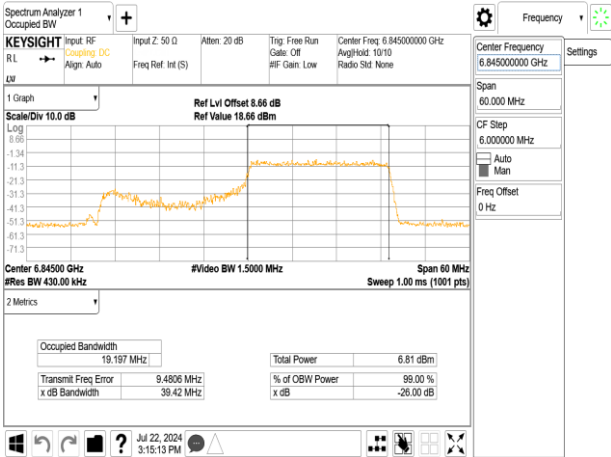
802.11ax_40MHz_Chain0_6845MHz_RU242_62
