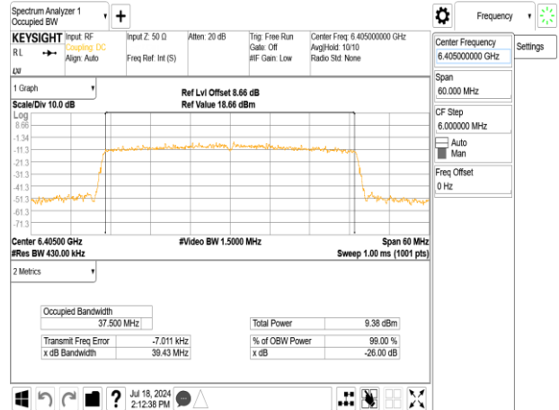
802.11ax_40MHz_Chain0_6405MHz_RU242_62
