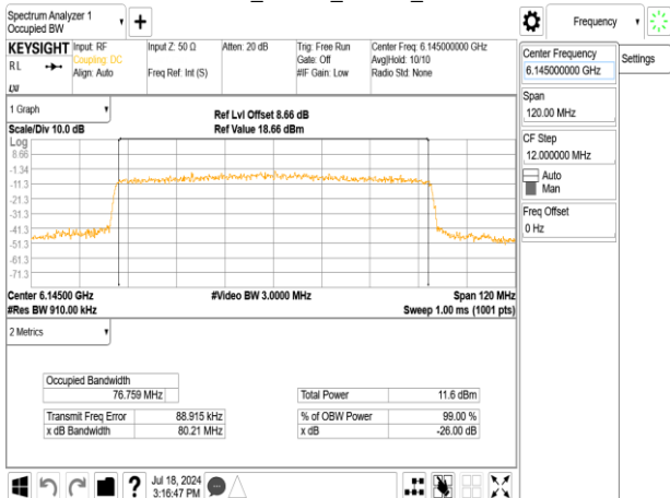
802.11ax_80MHz_Chain0_6145MHz
