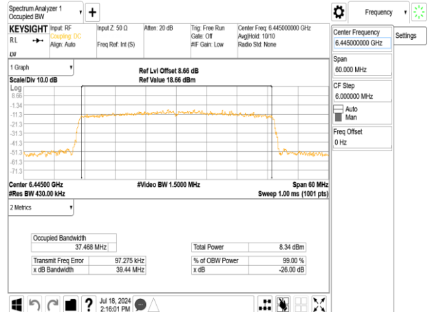
802.11ax_40MHz_Chain0_6445MHz
