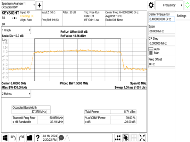
802.11ax_40MHz_Chain0_6485MHz_RU242_62
