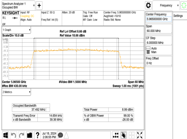
802.11ax_40MHz_Chain0_5965MHz_RU242_61
