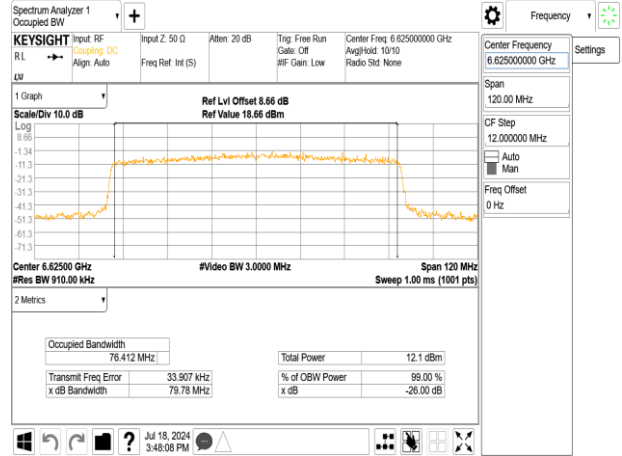
802.11ax_80MHz_Chain0_6625MHz_RU484_65
