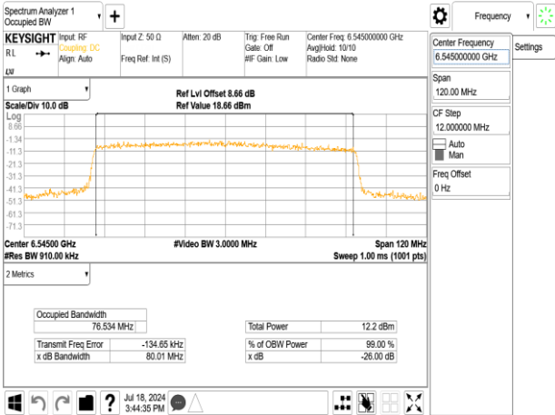
802.11ax_80MHz_Chain0_6545MHz
