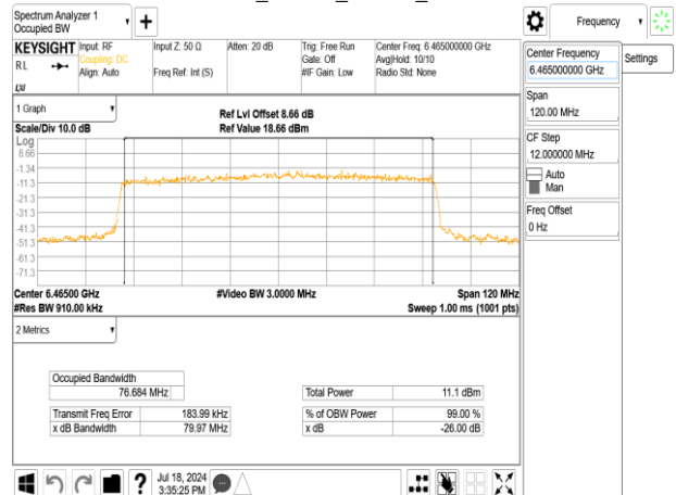
802.11ax_80MHz_Chain0_6465MHz
