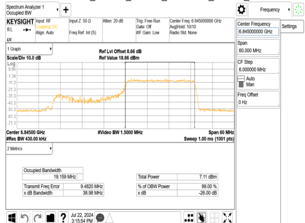
802.11ax_40MHz_Chain1_6845MHz_RU242_62
