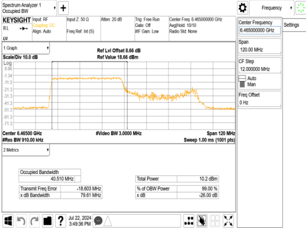
802.11ax_80MHz_Chain0_6465MHz_RU484_66
