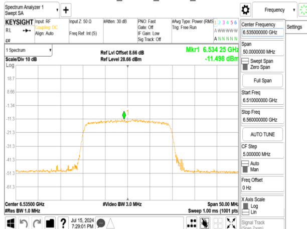
802.11ax_20MHz_Chain0_6535MHz_RU106_53
