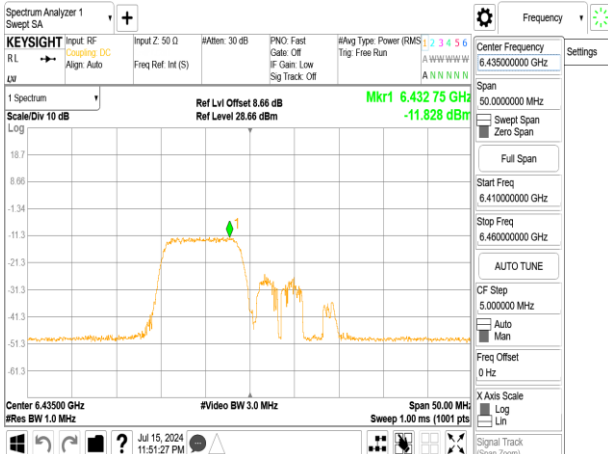
802.11ax_20MHz_Chain0_6435MHz_RU106_53
