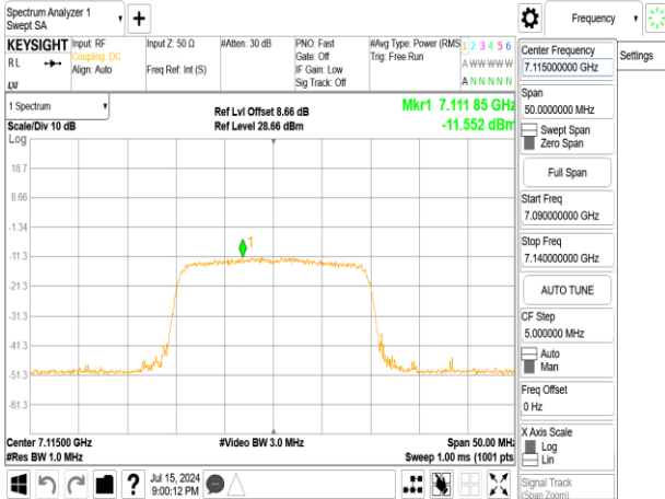
802.11ax_20MHz_Chain0_7115MHz_RU106_54PNG
