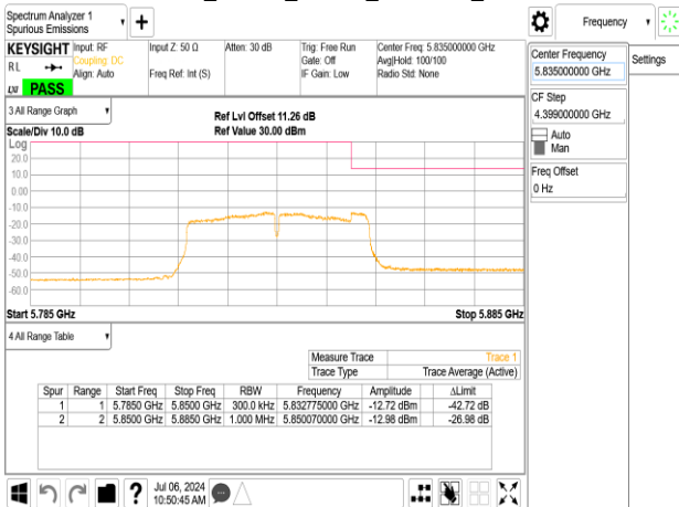
802.11n_40MHz_Chain1_5835MHz_UNII 2C
