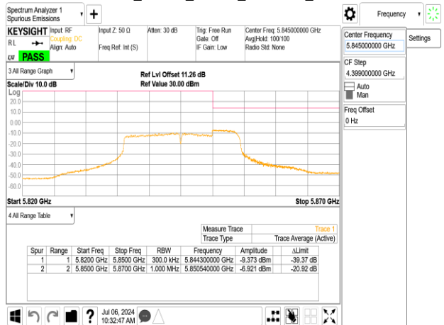
802.11n_20MHz_Chain1_5845MHz_UNII 2C
