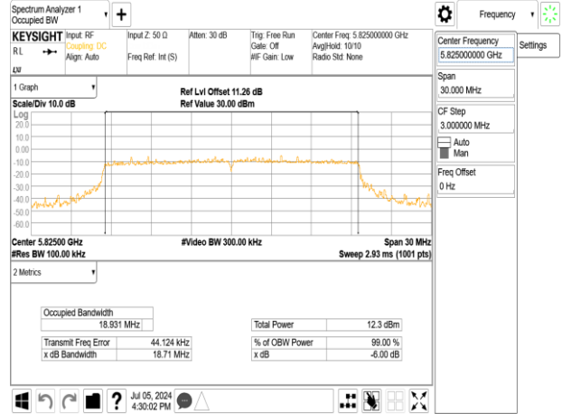
802.11ax_20MHz_Chain0_5825MHz_RU106_54
