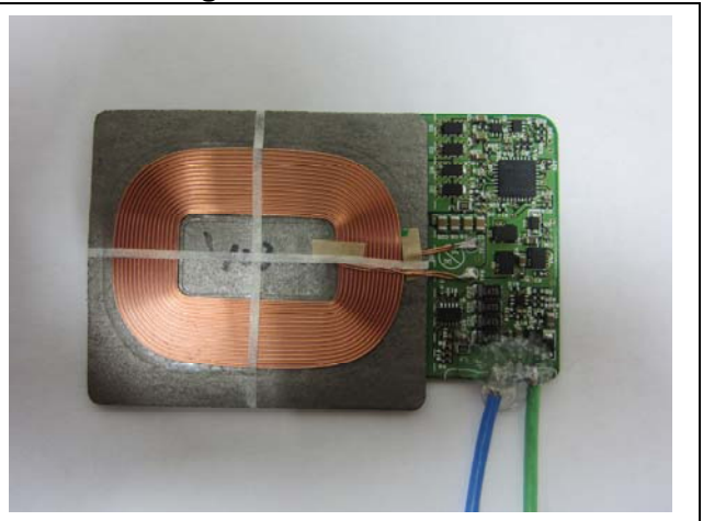
Jig Board for TM-A
