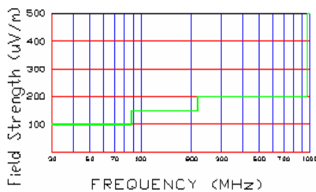
Figure A-6. Radiated limits at 3 meters.
