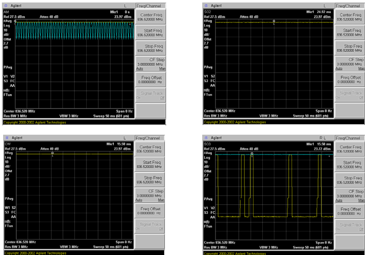
Figure 25 Zero-Span Plots
