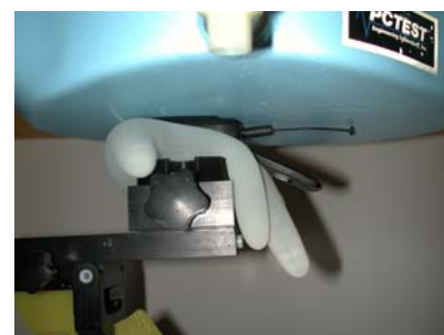
Figure 25. Hand SAR Test Setup
