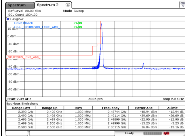
CP-OFDM QPSK - IC Low Channel - 1 RB
