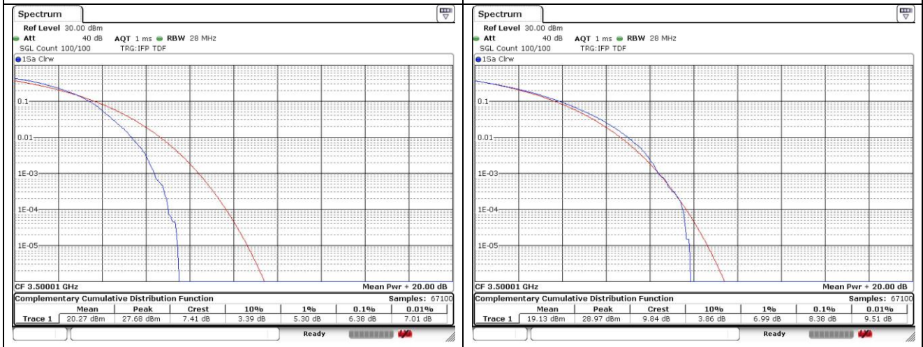
50 MHz Middle Channel - Full RB - DFT-S-OFDM
