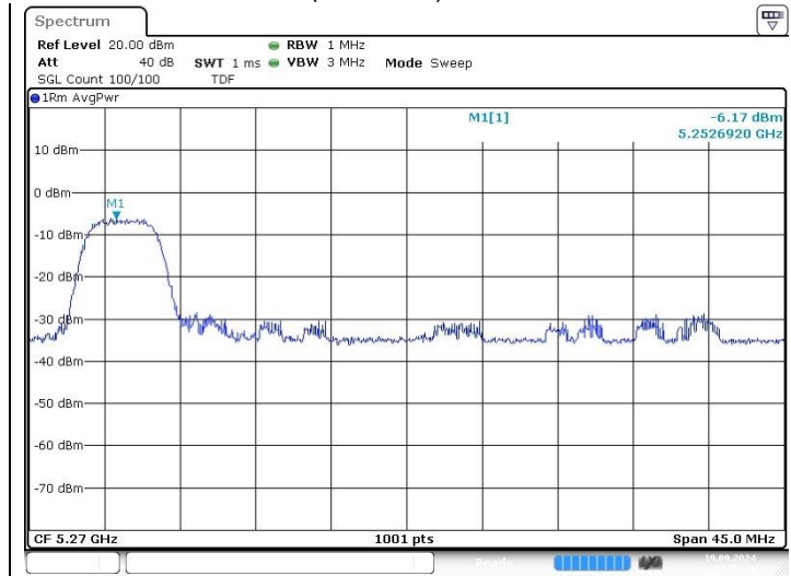
Low Channel (5 270 MHz)
