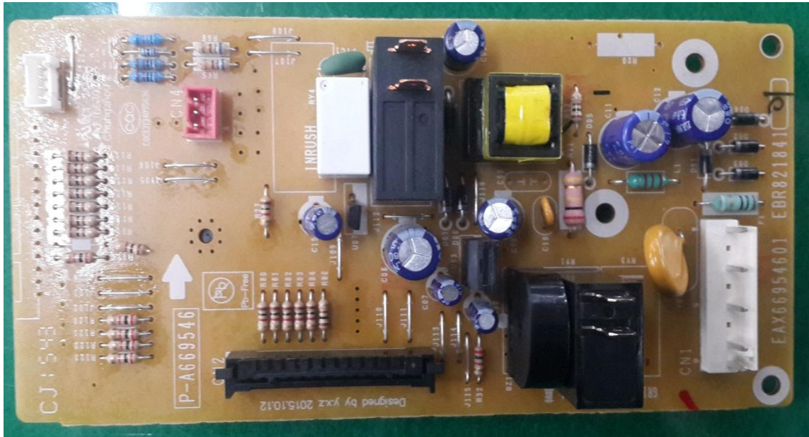
<PCB – Top of Main board>
