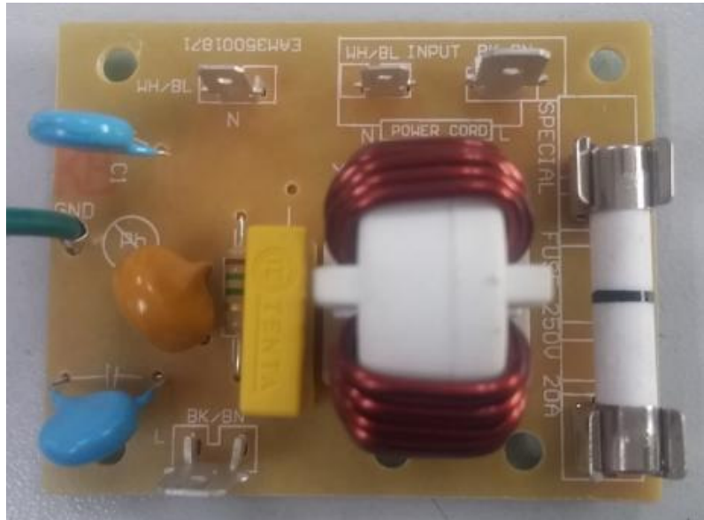
<Top of Noise filter>
