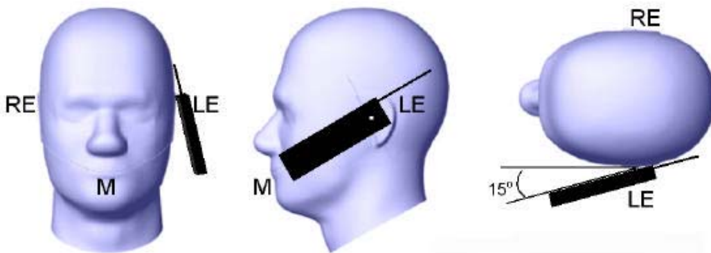
Fig. 6.4 “Tilted” Position.
