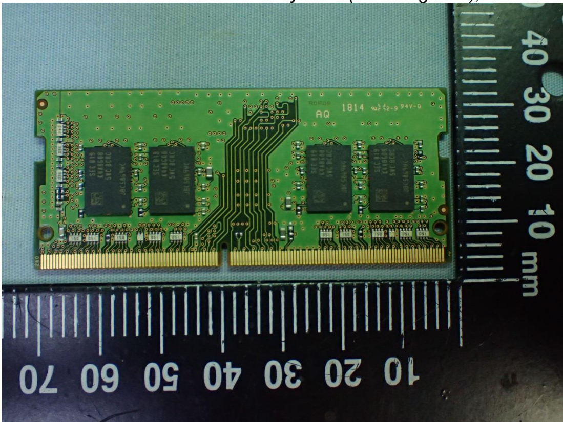
Figure 57 Memory Card (Samsung 8GB), Back View
