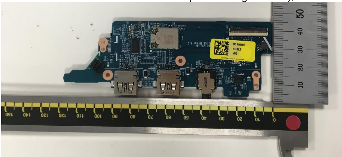
Figure 41 SUB Board (Without Finger Printer), Front View
