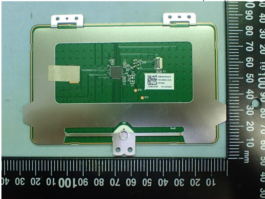
Figure 59 Touch Pad (White), Back View
