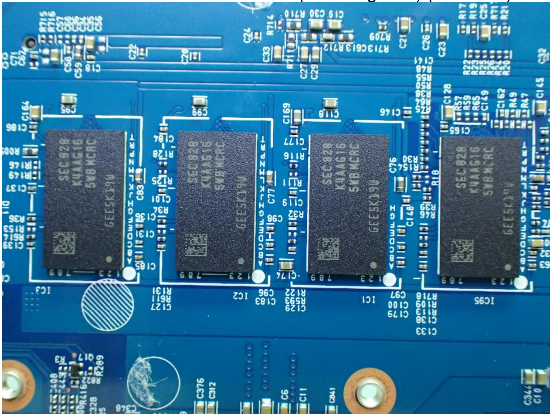
Figure 55 RAM (Samsung 8GB) (On Board) View
