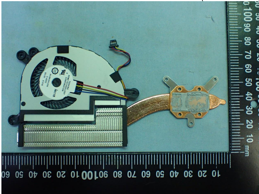
Figure 28 Internal View (CPU Heat Sink)
