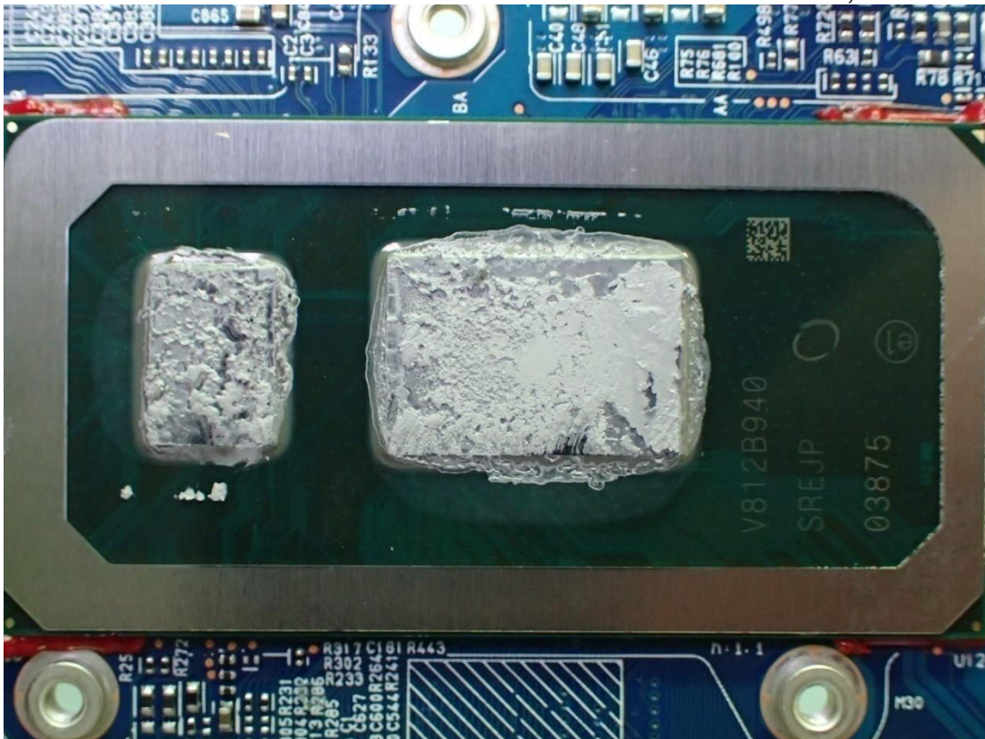
Figure 46 i7-8565U, CPU View
