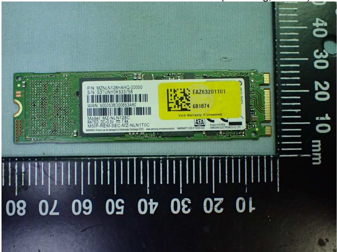
Figure 51 SSD (Samsung, 128GB) View
