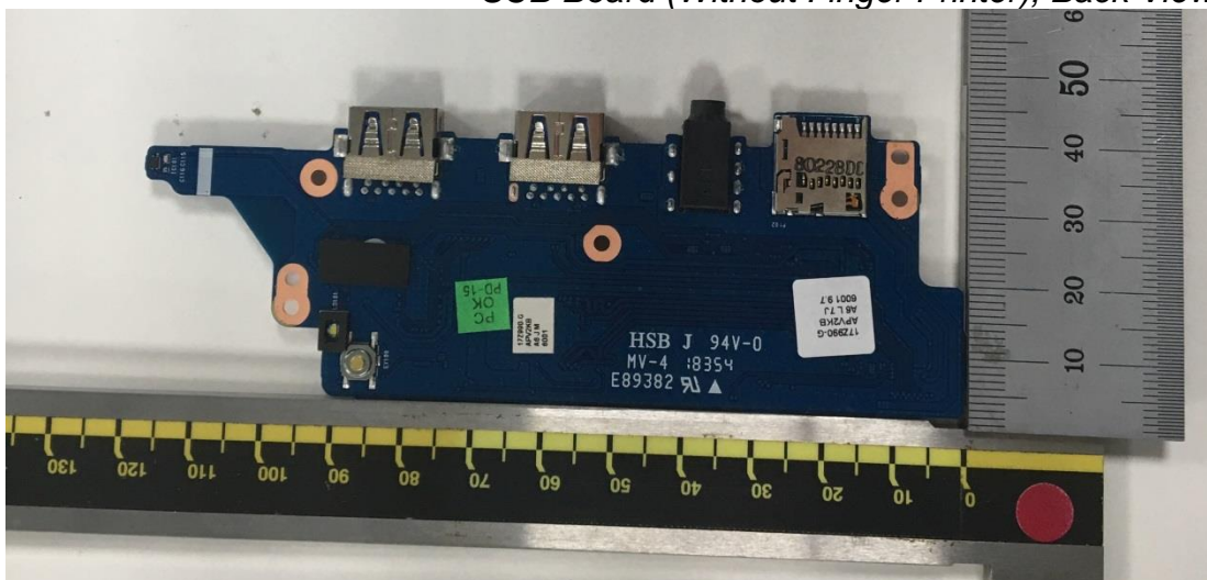
Figure 42 SUB Board (Without Finger Printer), Back View
