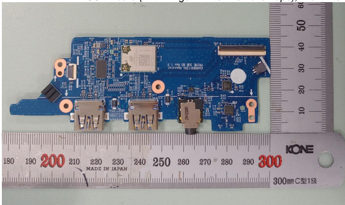
Figure 39 SUB Board (With Finger Printer-Remove Tape), Front View
