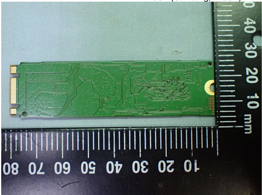
Figure 52 SSD (Samsung, 128GB) View
