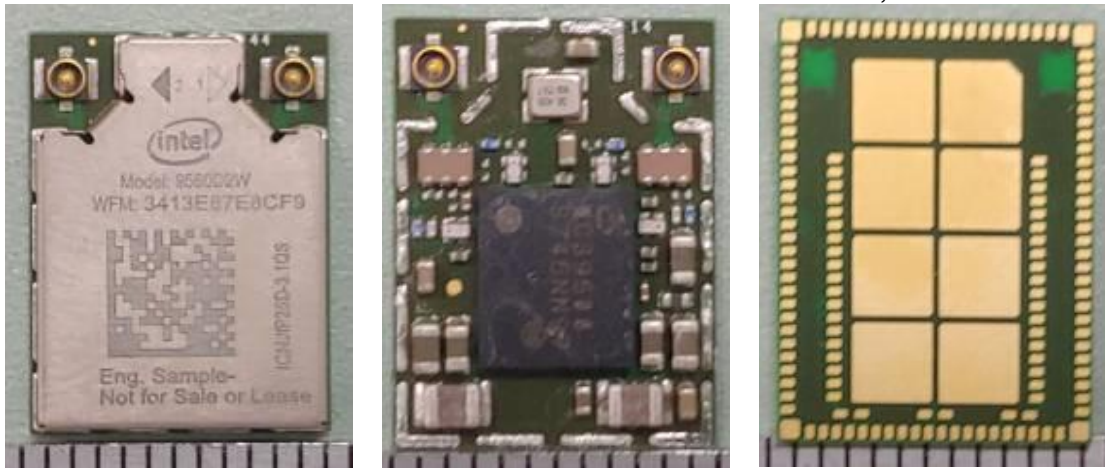
Figure 44 WLAN Combo Card, Remove Cover
