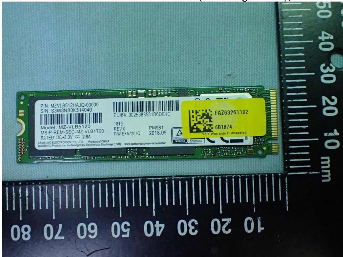
Figure 53 SSD (Samsung 512GB), Front View
