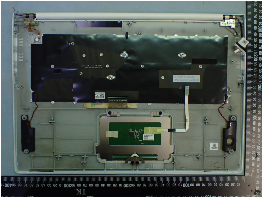
Figure 29 Internal View
