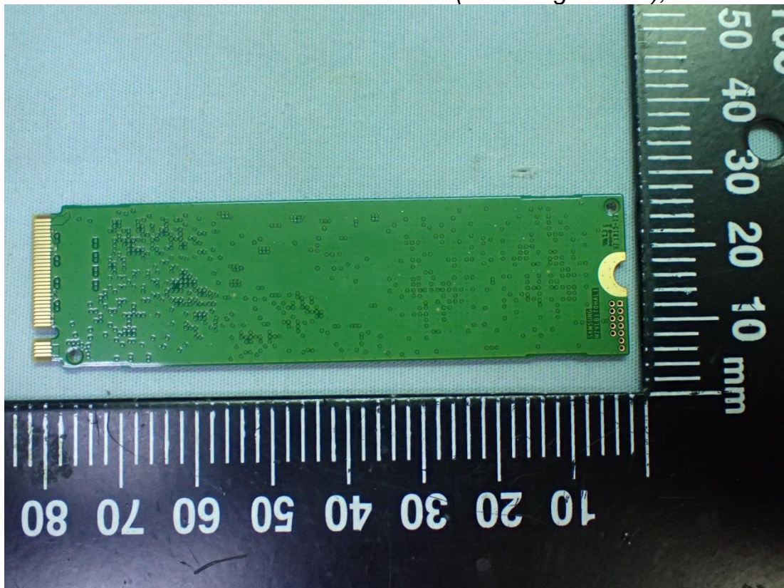
Figure 54 SSD (Samsung 512GB), Front View
