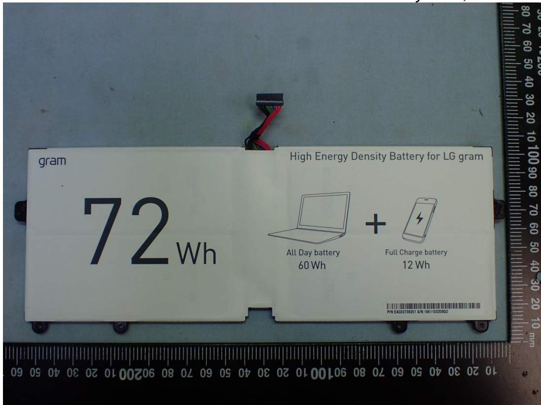
Figure 49 Battery Pack, Front View
