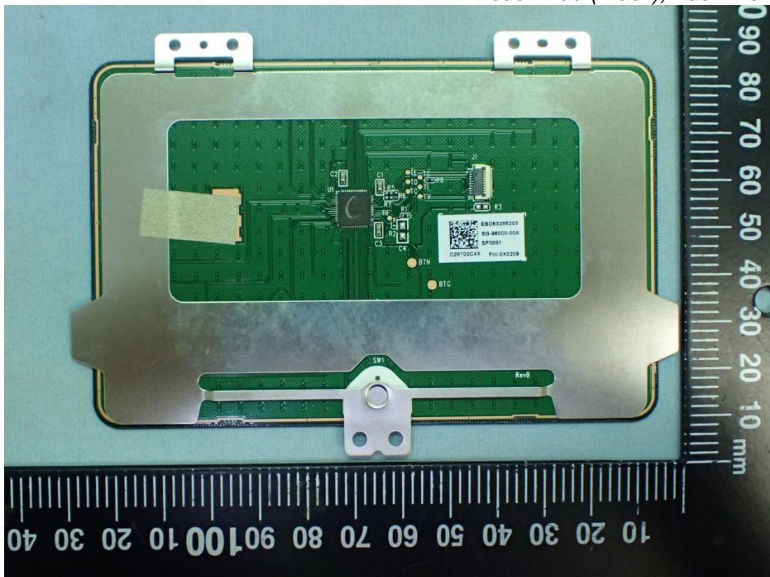
Figure 61 Touch Pad (Black), Back View
