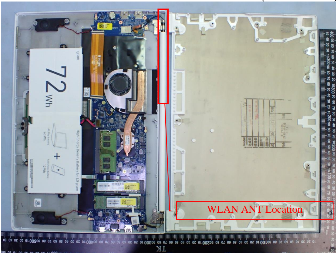
Figure 26 Internal View (Removed Cover)
