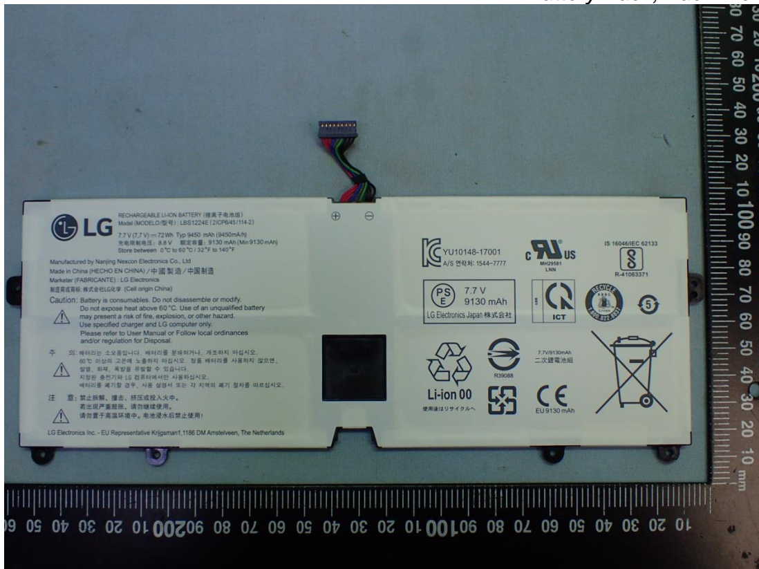
Figure 50 Battery Pack, Back View
