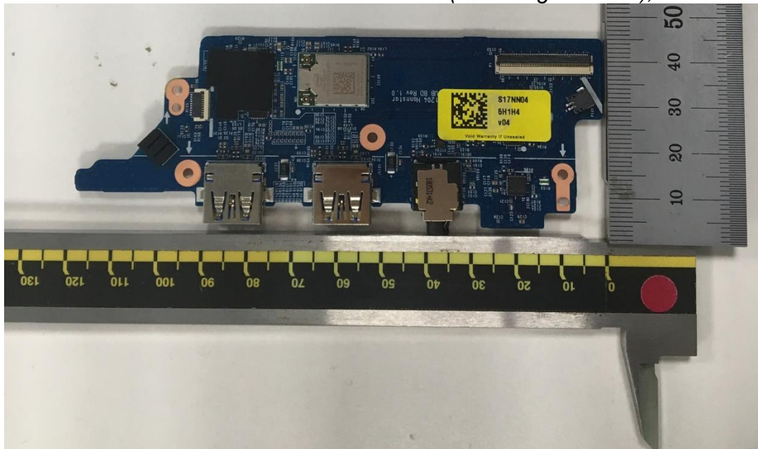
Figure 38 SUB Board (With Finger Printer), Front View
