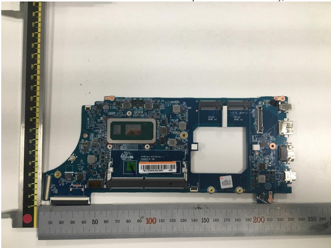
Figure 36 Main Board (without Thunderbolt), Front View
