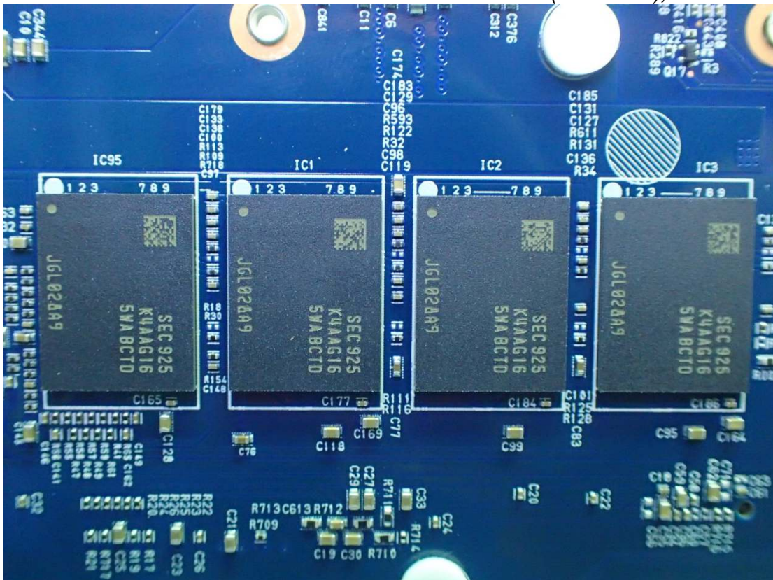
Figure 26 RAM (On Board), Back View
