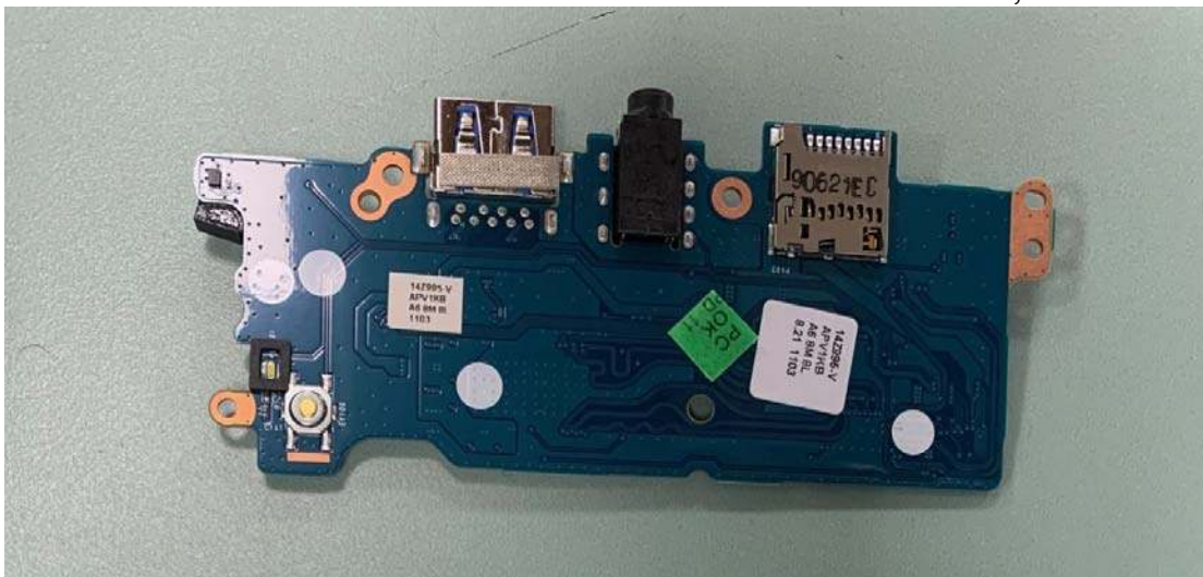
Figure 18 SUB Board, Back View
