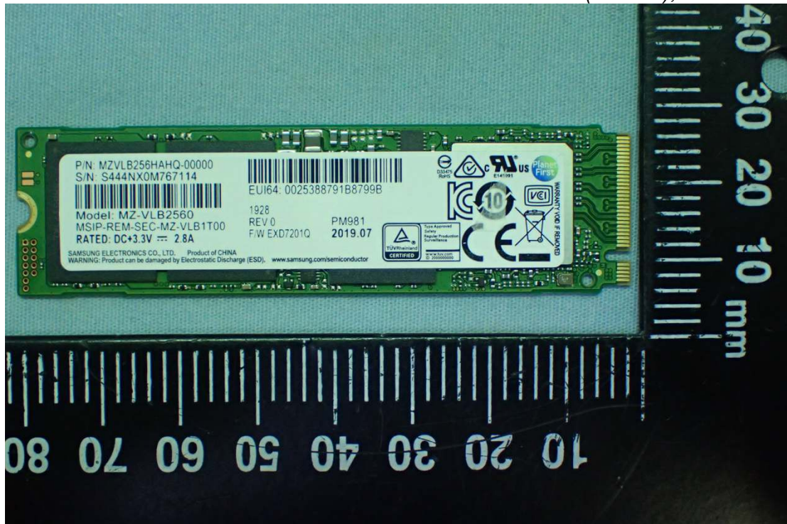
Figure 23 SSD (256GB), Front View
