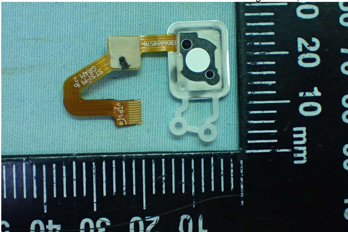
Figure 32 Finger Print , Back View
