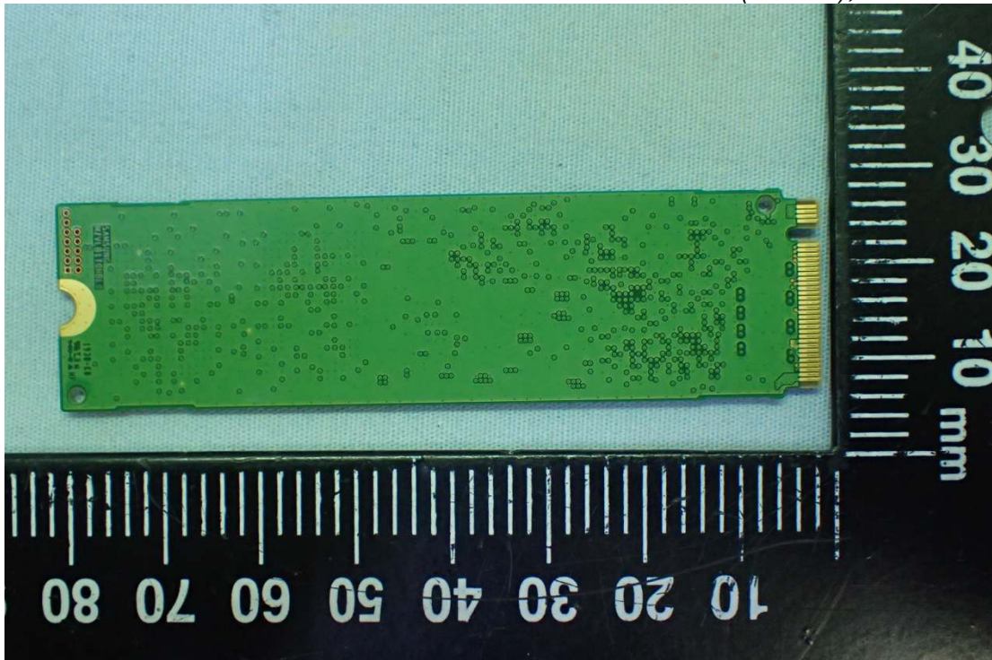
Figure 22 SSD (512GB), Back View
