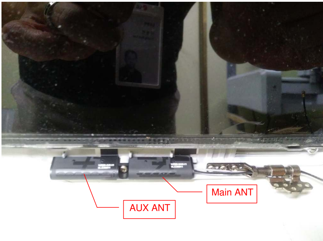
Figure 14 WLAN Combo Antenna Position
