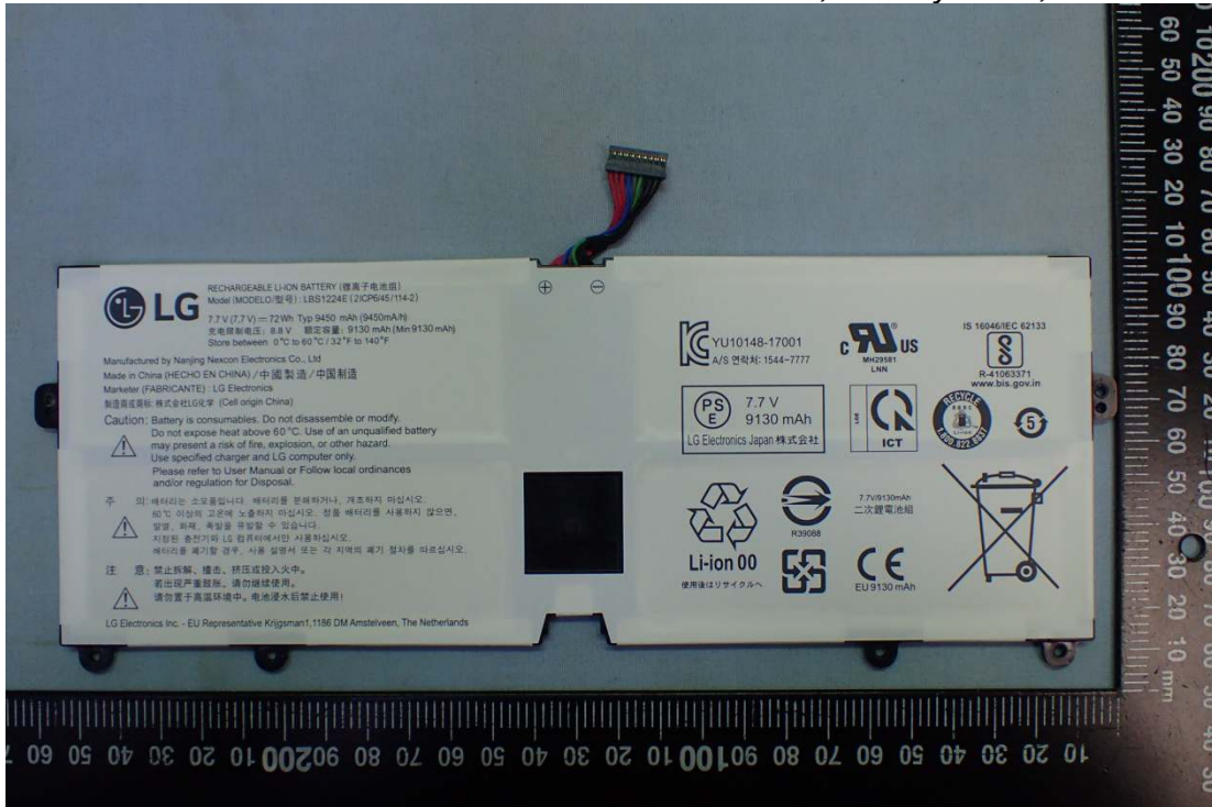
Figure 10 M/N: LBS1224E, Battery Pack, Back View
