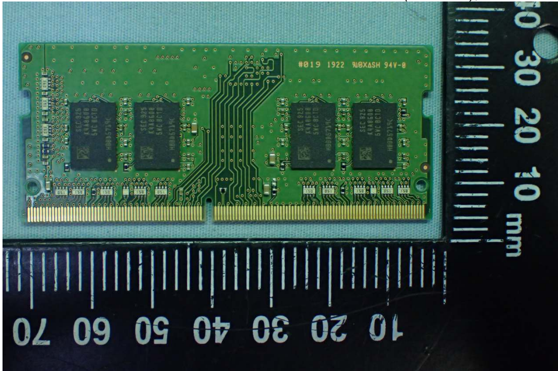
Figure 27 RAM (On Card), Front View
