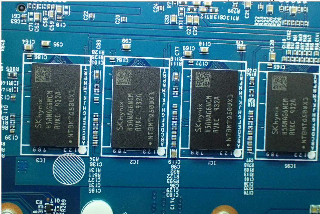
Figure 25 RAM (On Board), Front View
