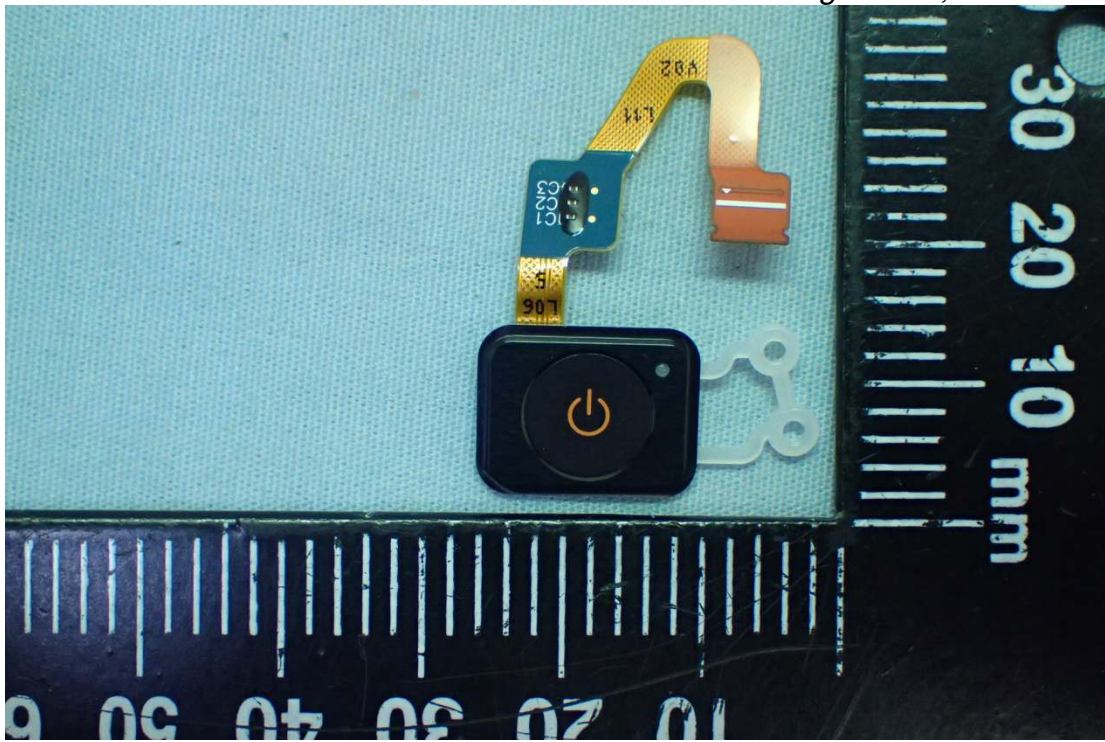
Figure 29 Finger Print, Front View
