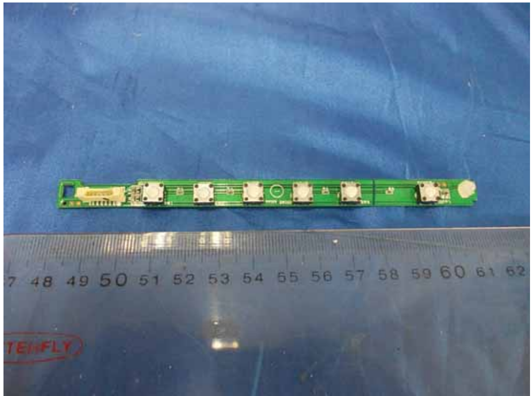
FIGURE 9 LCD MONITOR (M/N: N2311AZ) KEY BOARD (COMPONENT SIDE)
