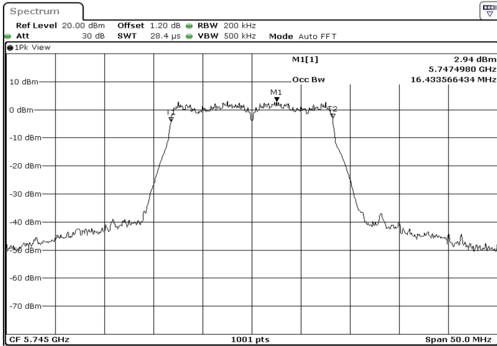
1 99% Occupied Bandwidth
