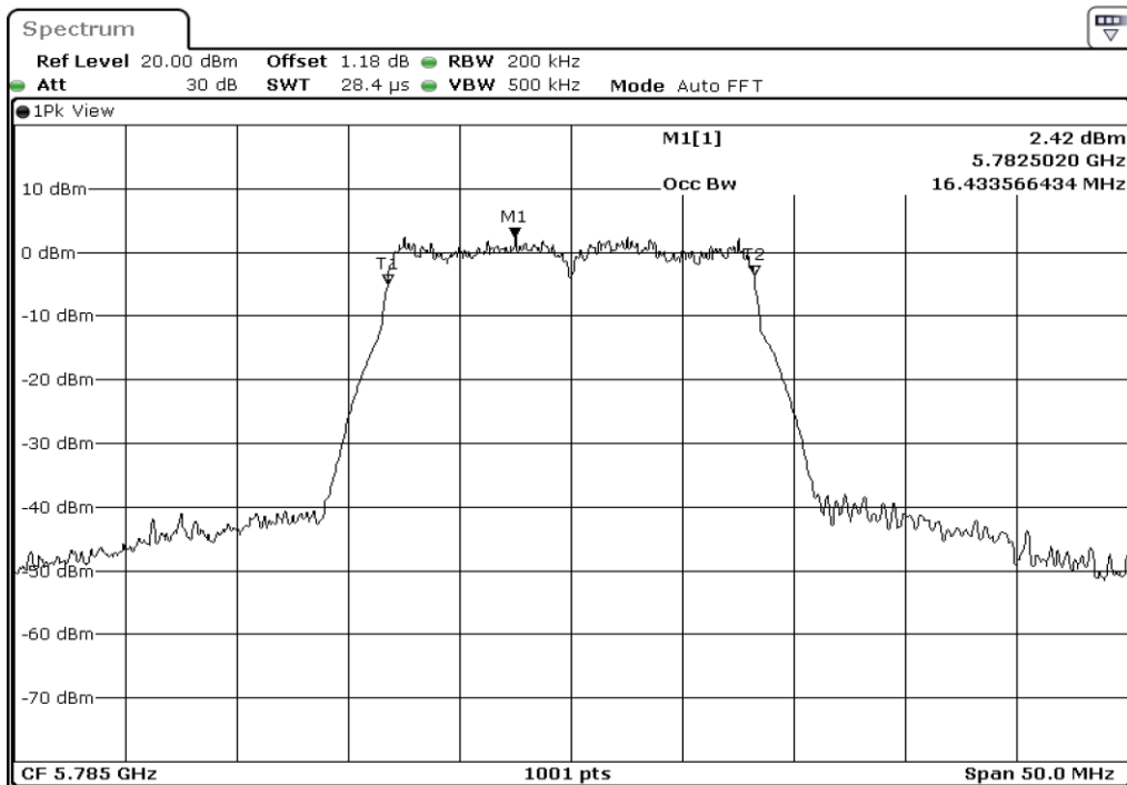
2 99% Occupied Bandwidth
