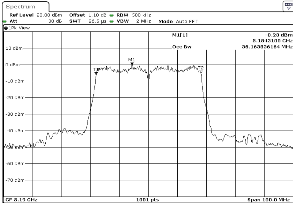
7 99% Occupied Bandwidth
