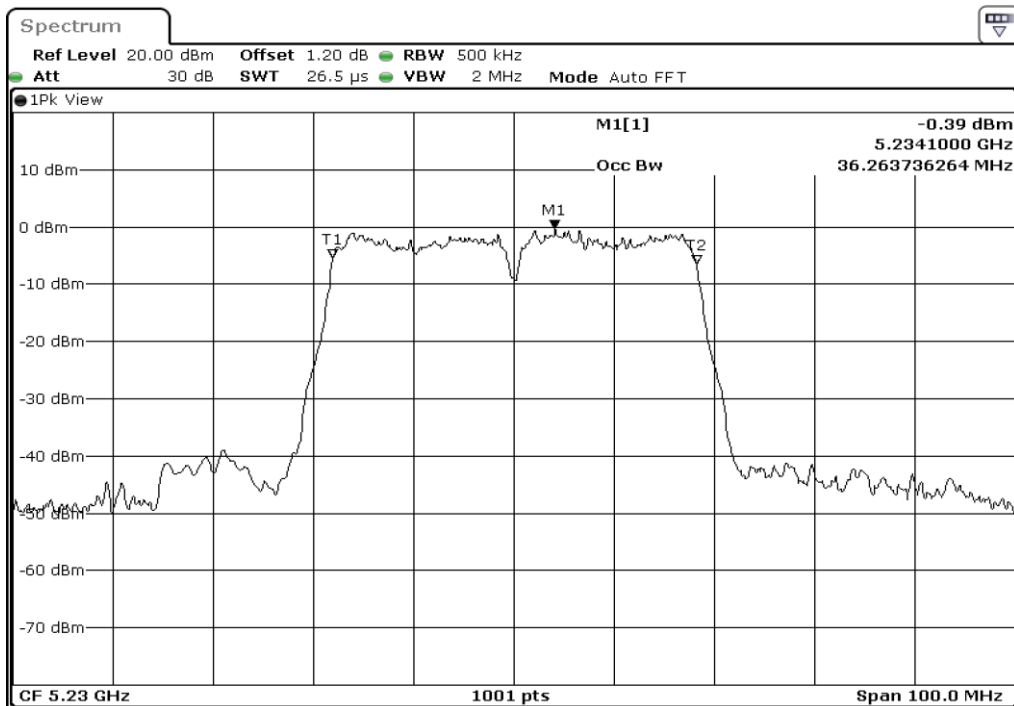
8 99% Occupied Bandwidth
