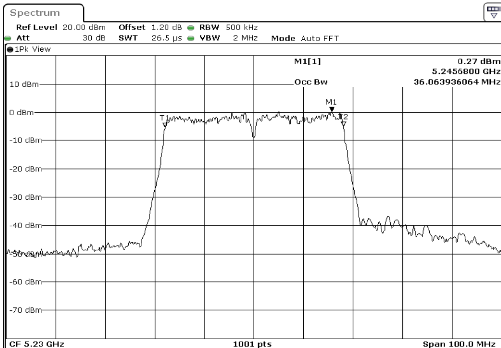
8 99% Occupied Bandwidth
