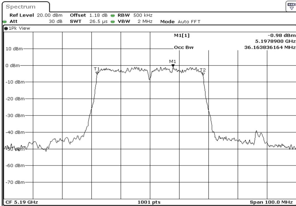
7 99% Occupied Bandwidth
