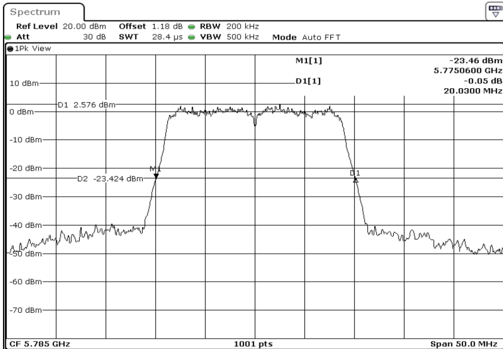
5 26dB Bandwidth
