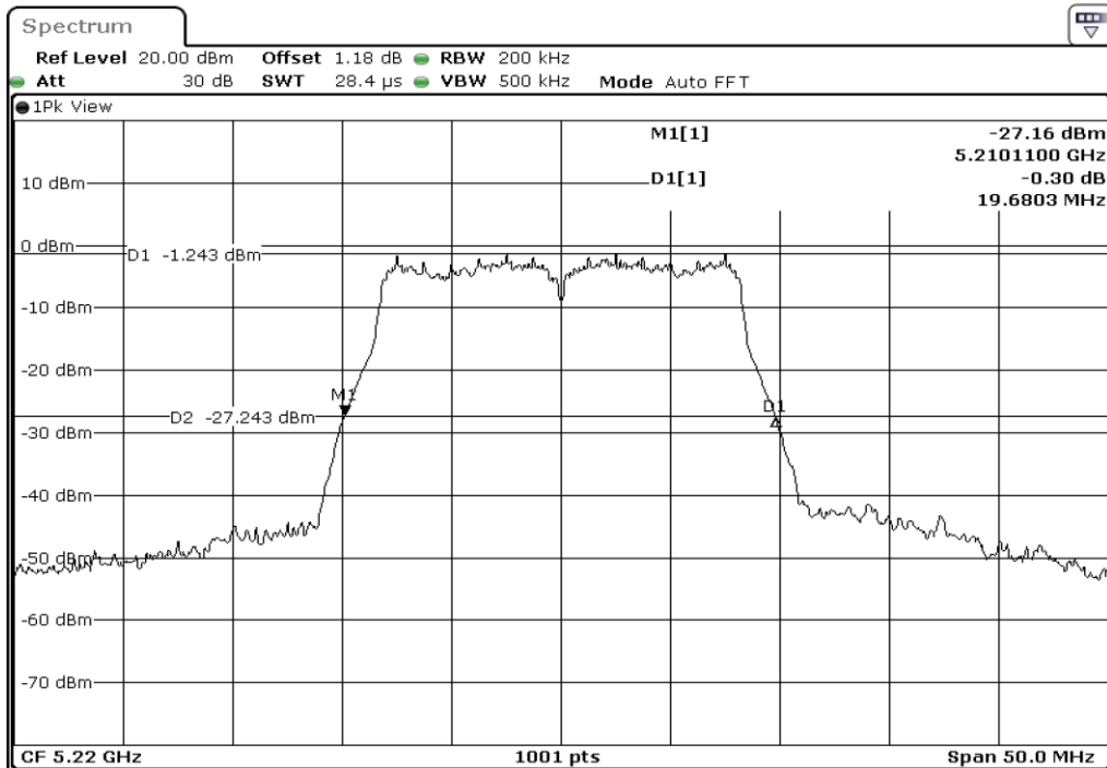
2 26dB Bandwidth
