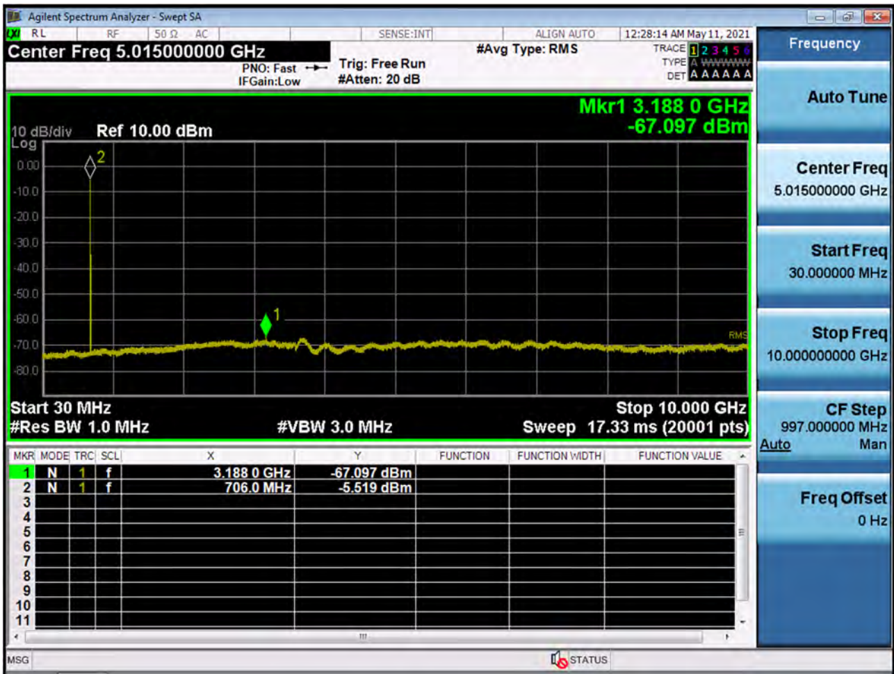
BAND 17. Conducted Spurious Plot _ (23790ch_10MHz_QPSK_RB 1_0)
