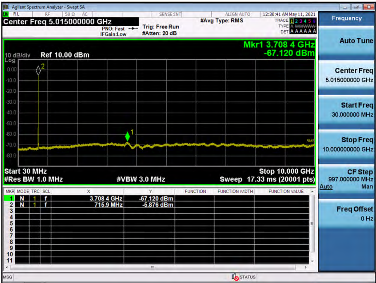
BAND 17. Conducted Spurious Plot _ (23800ch_10MHz_QPSK_RB 1_0)
