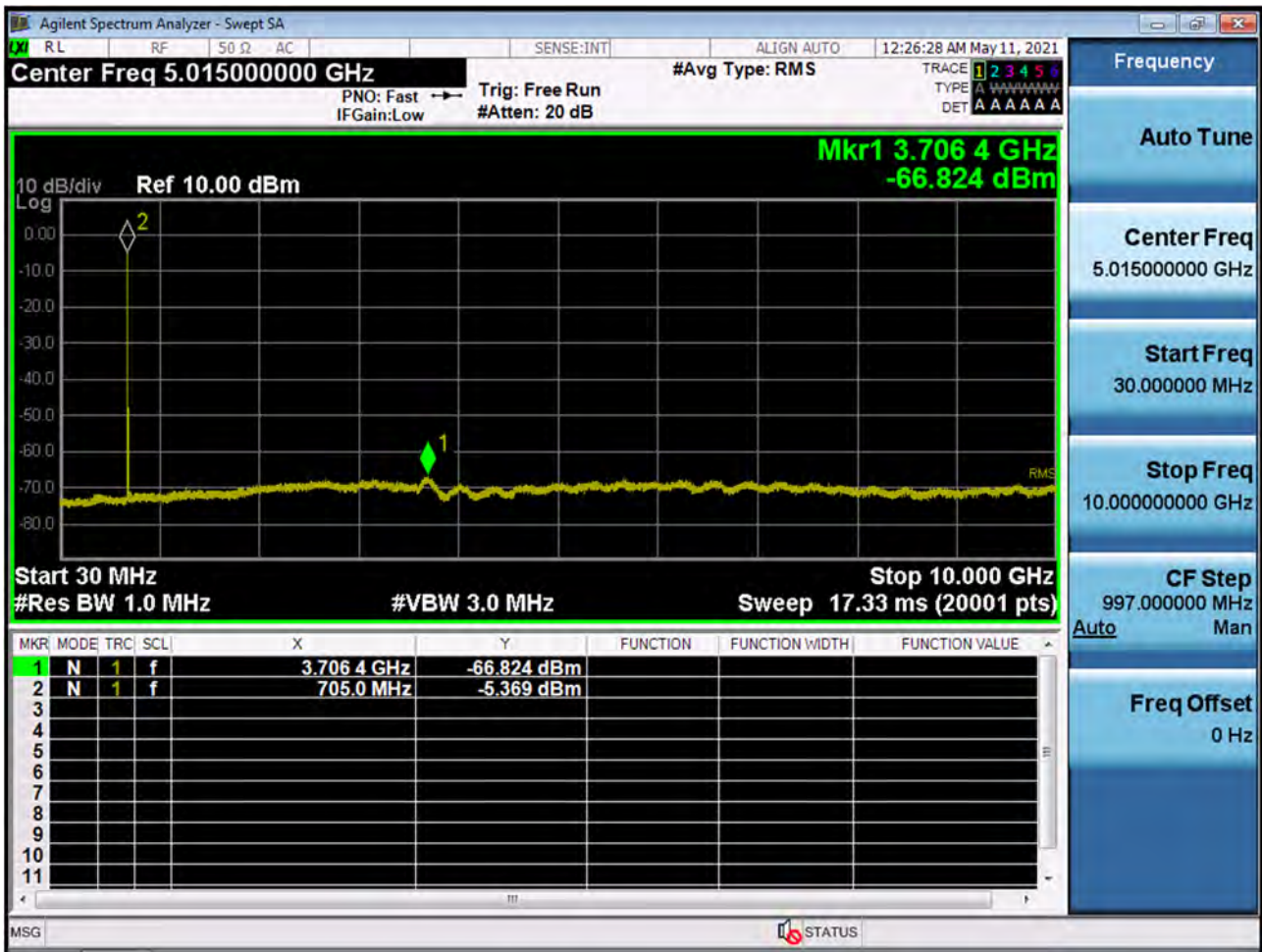
BAND 17. Conducted Spurious Plot _ (23780ch_10MHz_QPSK_RB 1_0)
