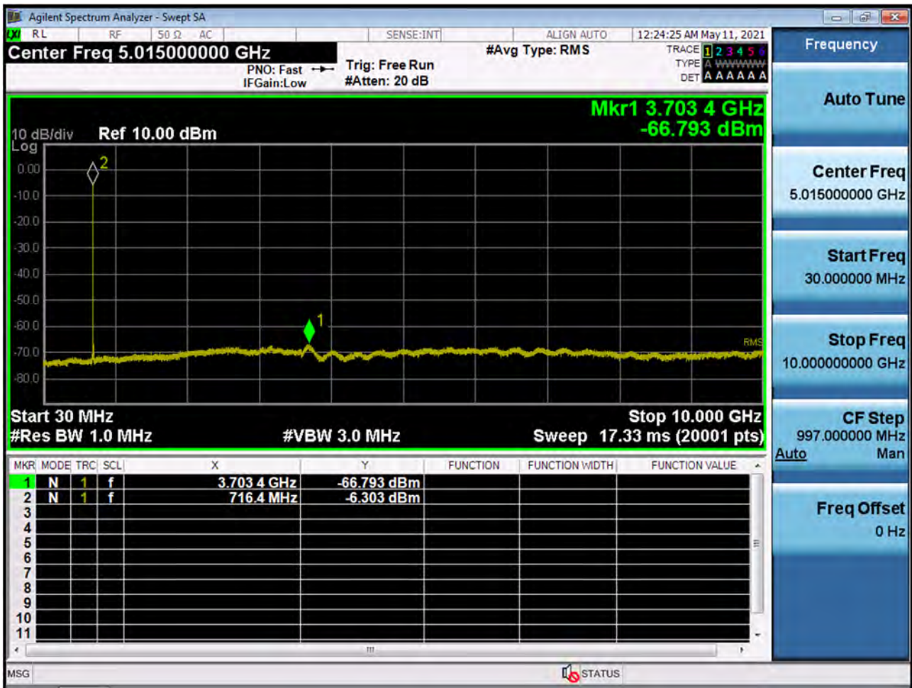
BAND 17. Conducted Spurious Plot _ (23825ch_5MHz_QPSK_RB 1_0)
