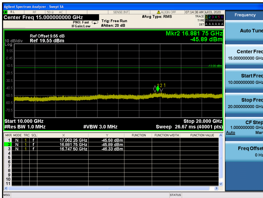
LTE Band 2 / 5MHz / 16QAM - RB Size/Offset (12/13) – Low Channel
