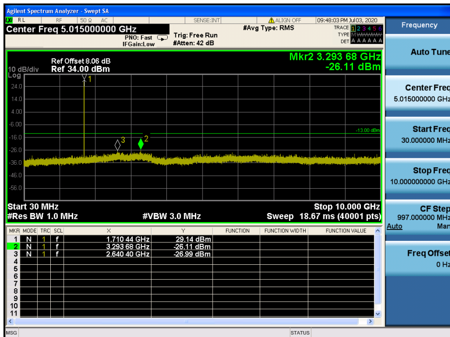
LTE Band 4 / 5MHz / 16QAM - RB Size/Offset (1/0) – Low Channel
