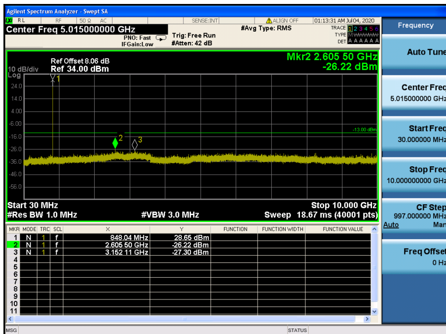
LTE Band 5 / 1.4MHz / QPSK - RB Size/Offset (1/0) – High Channel
