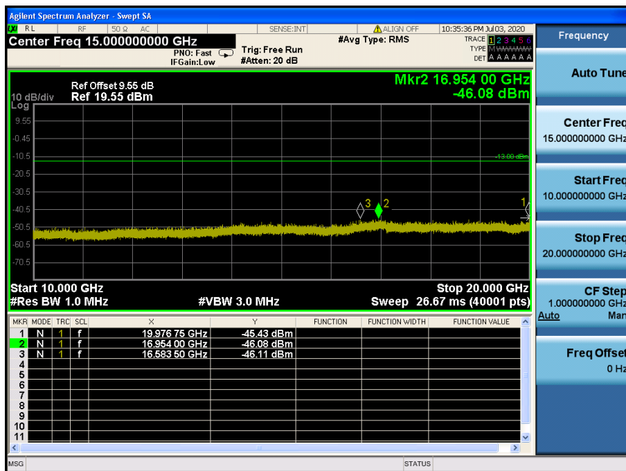
LTE Band 4 / 10MHz / 16QAM - RB Size/Offset (1/0) – Low Channel
