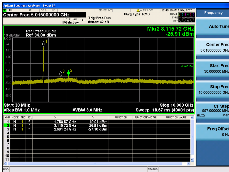
LTE Band 4 / 20MHz / 16QAM - RB Size/Offset (100/0) – High Channel
