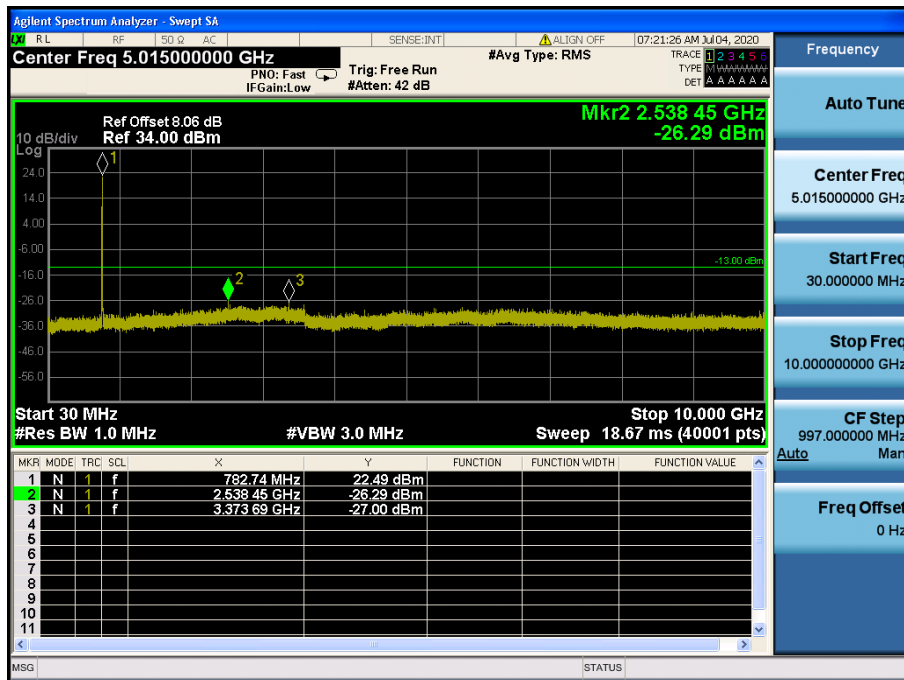
LTE Band 13 / 10MHz / QPSK - RB Size/Offset (25/25) – Low Channel
