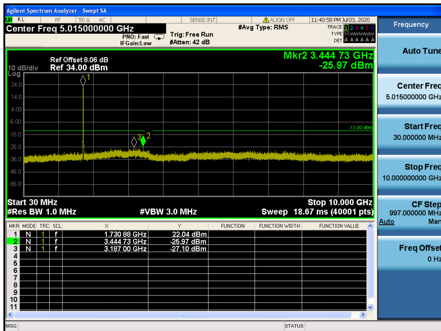
LTE Band 4 / 15MHz / 16QAM - RB Size/Offset (36/18) – Mid Channel
