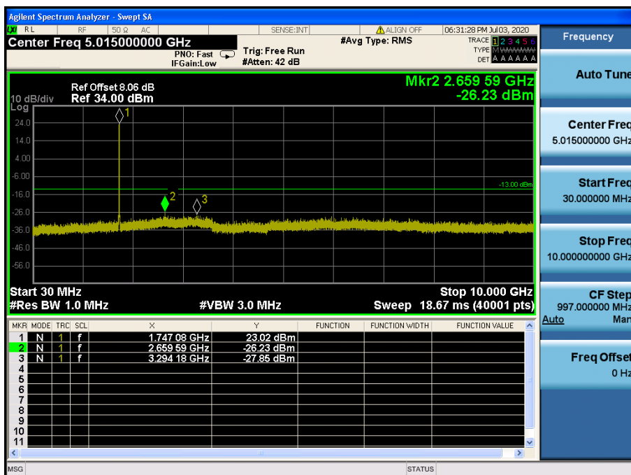
LTE Band 4 / 10MHz / QPSK - RB Size/Offset (25/0) – High Channel
