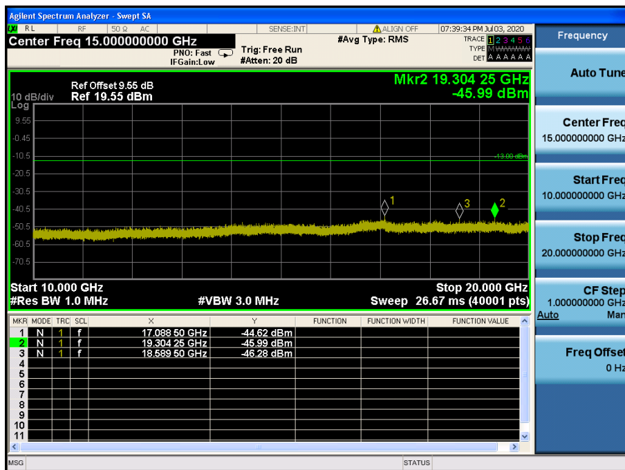
LTE Band 4 / 20MHz / QPSK - RB Size/Offset (50/25) –Low Channel
