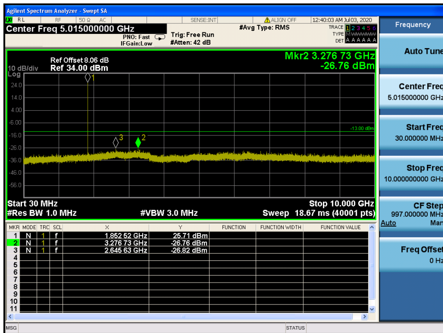
LTE Band 2 / 3MHz / QPSK - RB Size/Offset (8/7) – Low Channel
