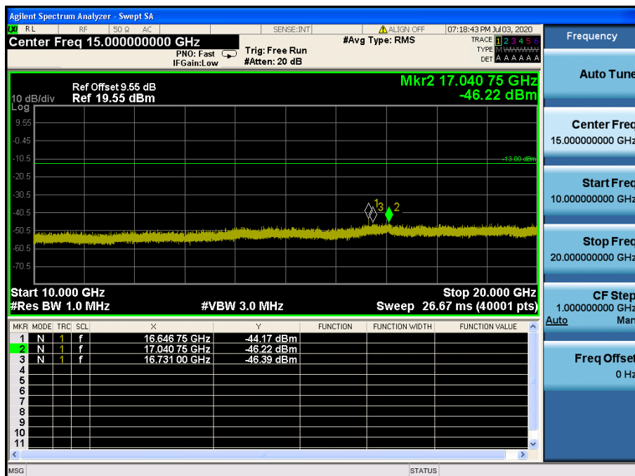
LTE Band 4 / 15MHz / QPSK - RB Size/Offset (36/18) – High Channel
