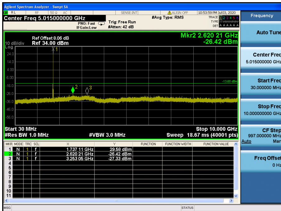
LTE Band 4 / 10MHz / 16QAM - RB Size/Offset (1/49) – Mid Channel
