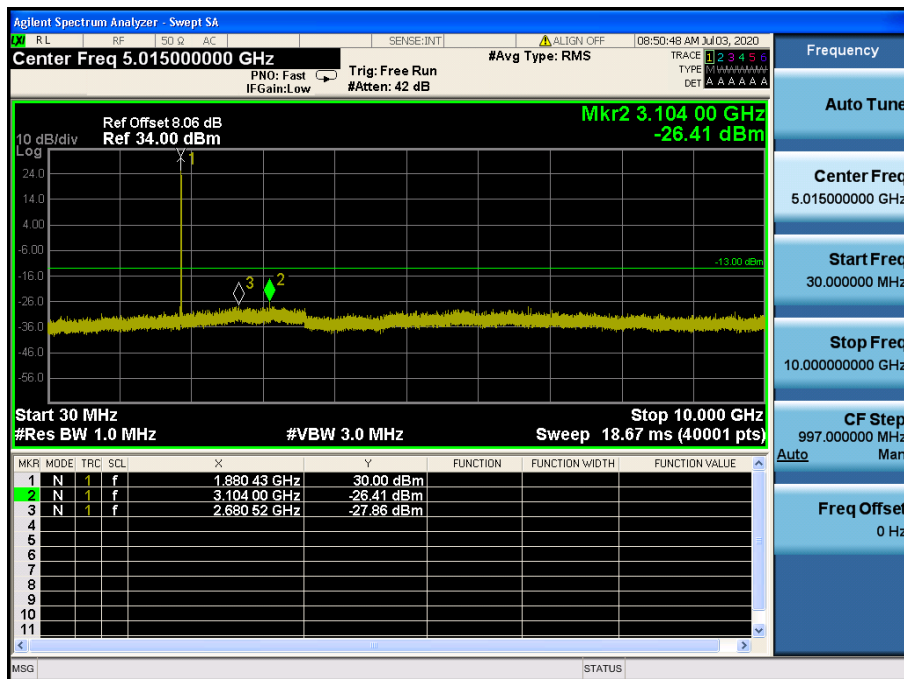
LTE Band 2 / 15MHz / 16QAM - RB Size/Offset (1/36) – Mid Channel
