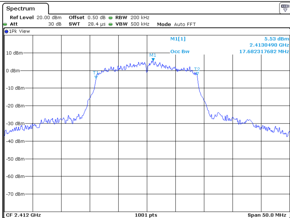
802.11 HT20_Low Channel
