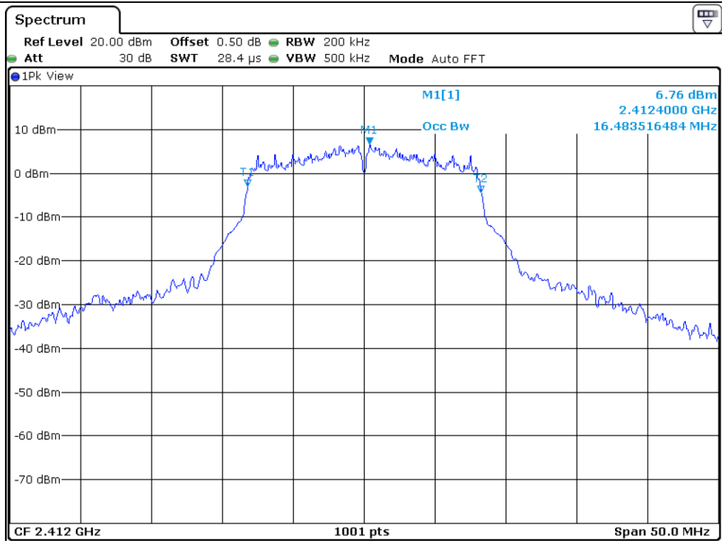
802.11 g_Low Channel
