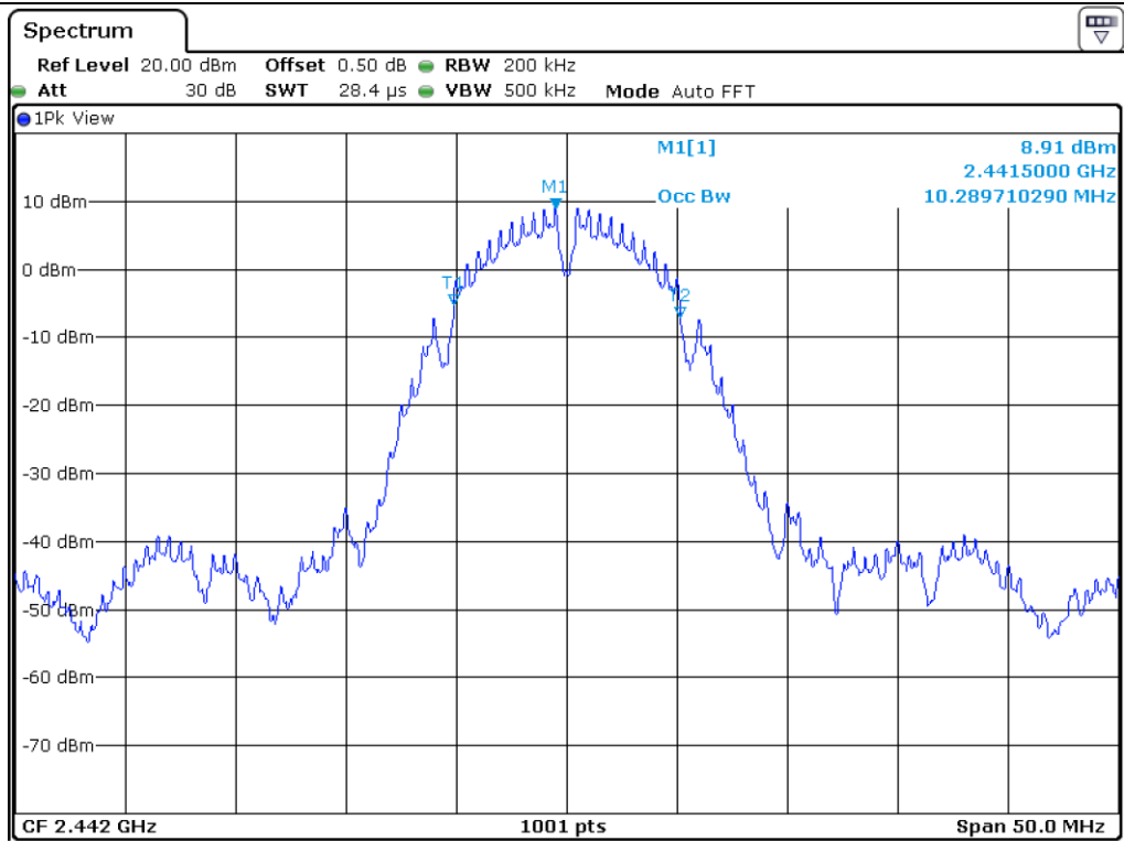
802.11 b_Middle Channel
