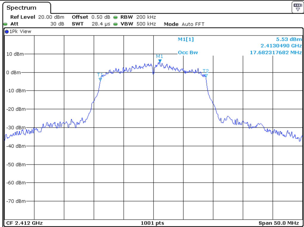
802.11 HT20_Low Channel
