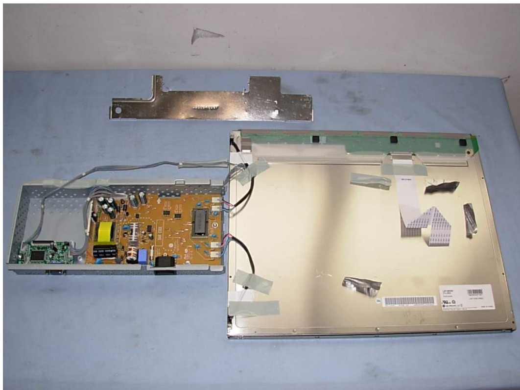
FIGURE 2 LCD MONITOR (M/N: L1919SS) SHIELDED COVER
