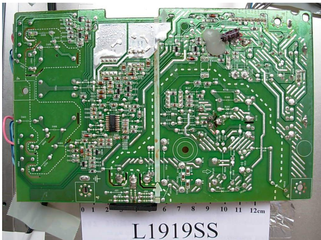
FIGURE 8 LCD MONITOR (M/N: L1919SS) POWER BOARD (SOLDERED SIDE)
