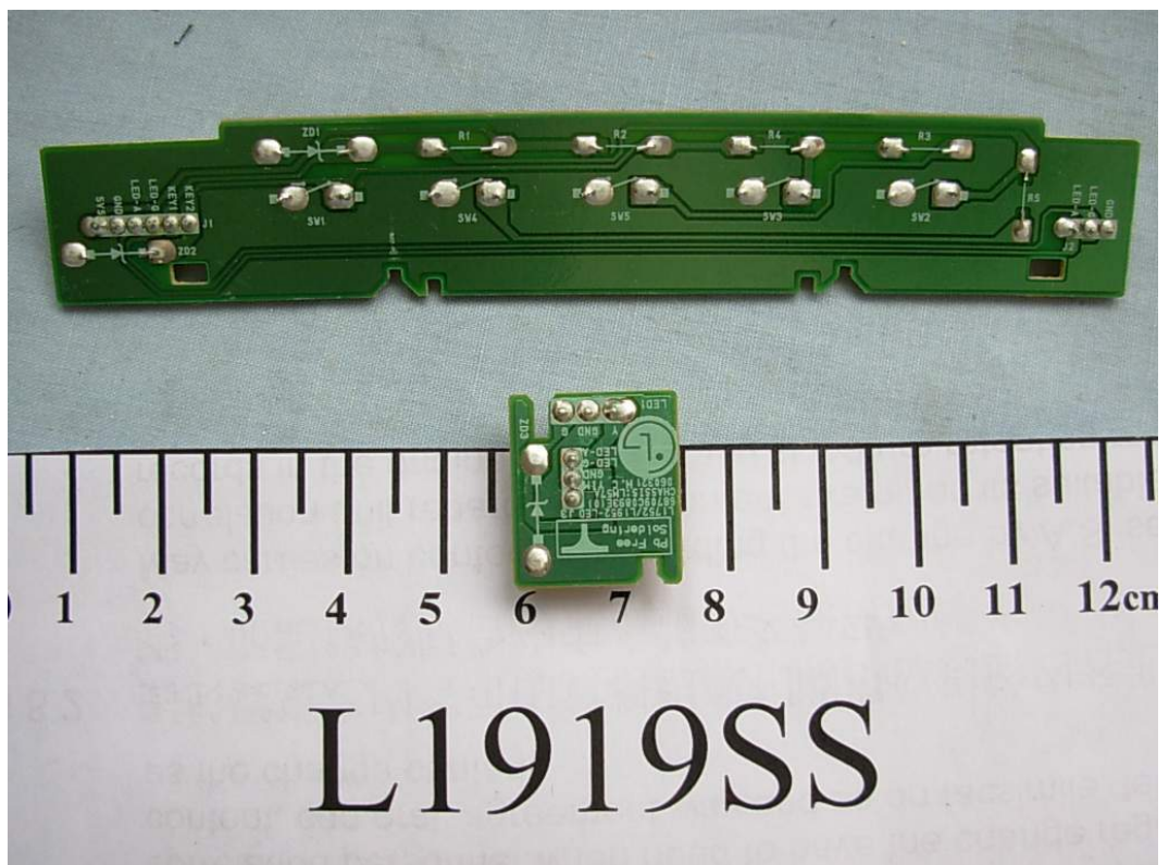
FIGURE 16 LCD MONITOR (M/N: L1919SS) SWITCH & LED BOARD (SOLDERED SIDE)
