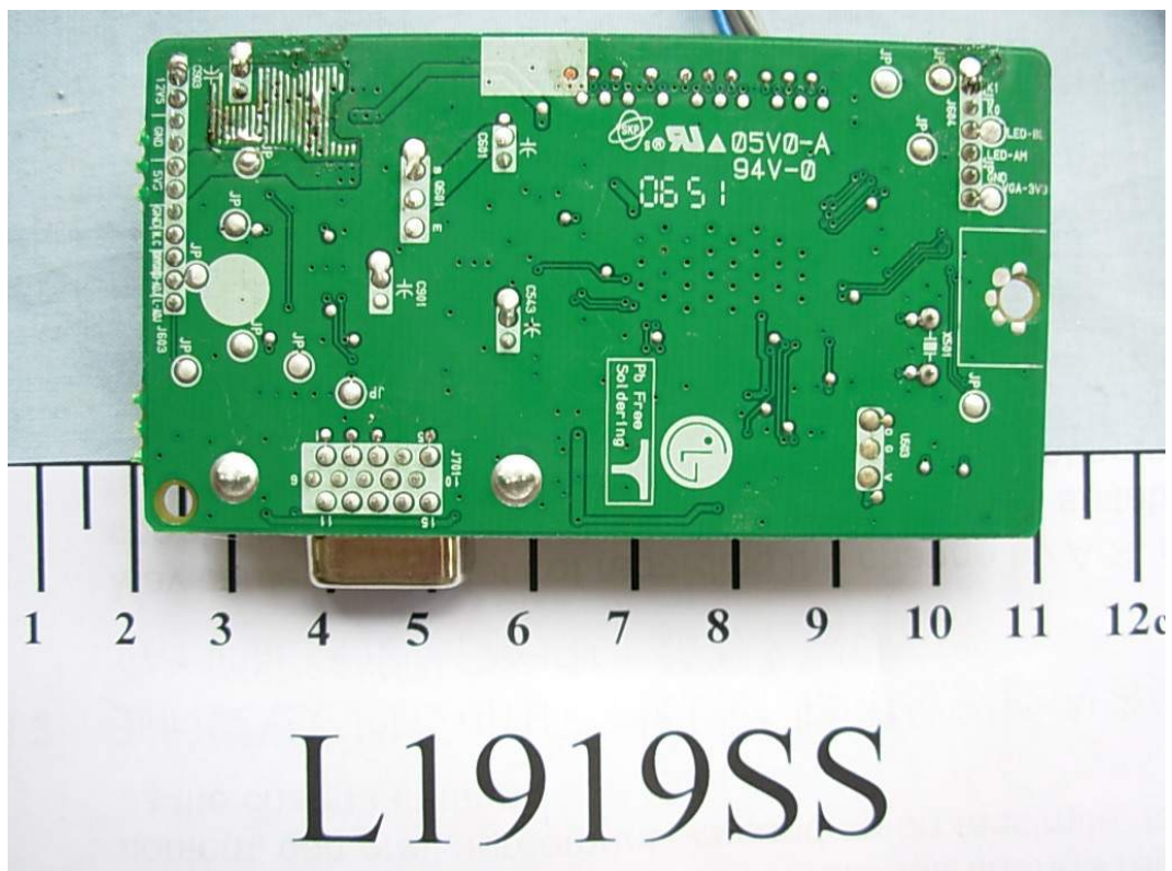
FIGURE 4 LCD MONITOR (M/N: L1953TS) MAIN BOARD (SOLDERED SIDE)
