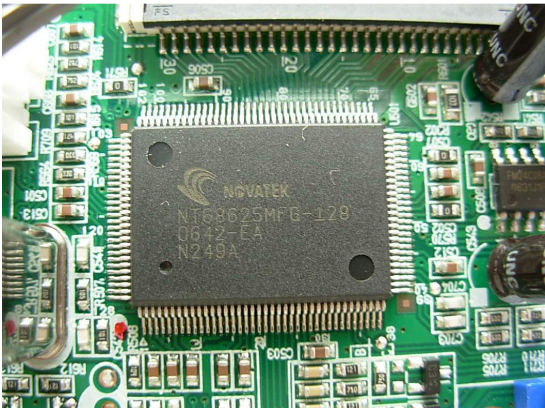
FIGURE 6 LCD MONITOR (M/N: L1919SS) CHIP ON MAIN BOARD
