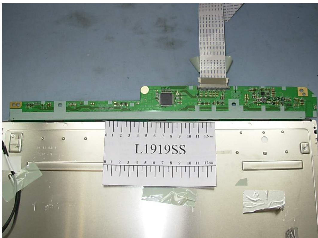
FIGURE 13 LCD MONITOR (M/N: L1919SS) LCD PANEL MAIN BOARD (BACK VIEW)
