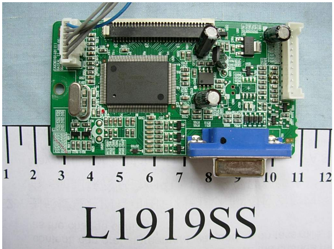
FIGURE 3 LCD MONITOR (M/N: L1919SS) MAIN BOARD (COMPONENT SIDE)
