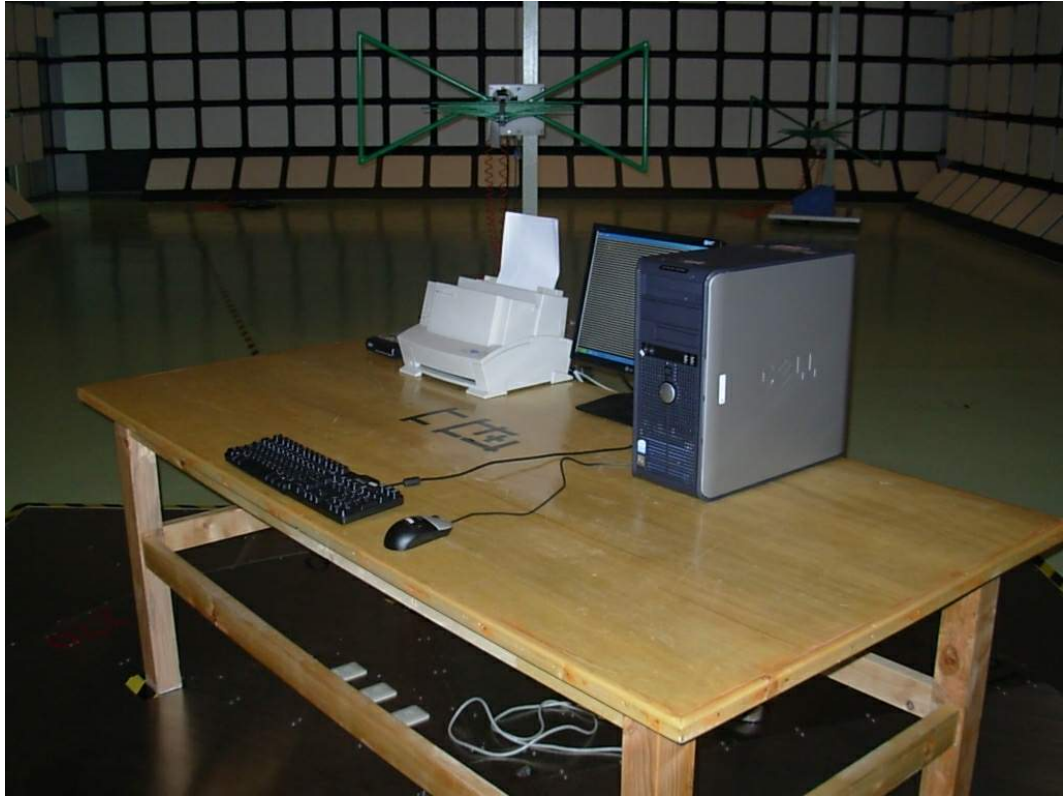
SETUP WITH MAXIMUM DETECTED EMISSION AT HORIZONTAL POLARIZATION (VGA 800*600@75Hz)
