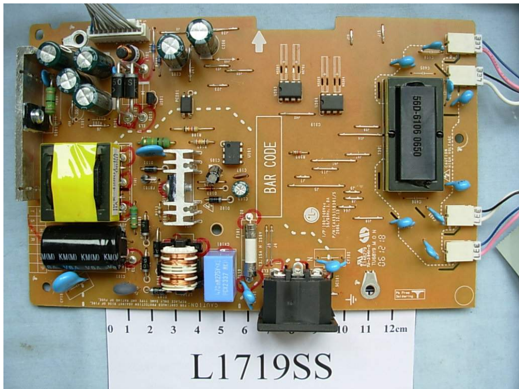
FIGURE 7 LCD MONITOR (M/N: L1719SS) POWER BOARD (COMPONENT SIDE)
