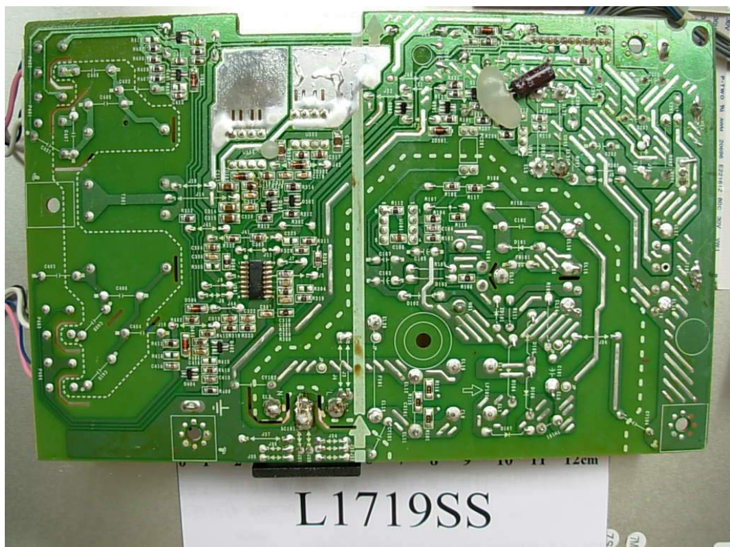
FIGURE 8 LCD MONITOR (M/N: L1719SS) POWER BOARD (SOLDERED SIDE)
