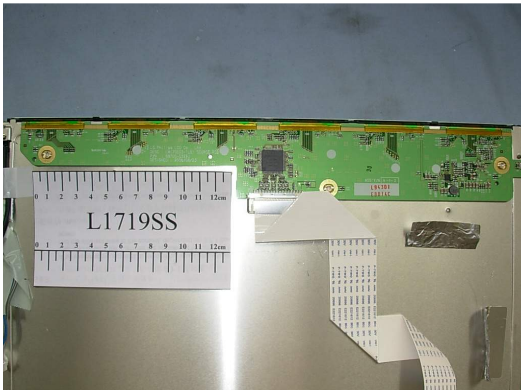
FIGURE 12 LCD MONITOR (M/N: L1719SS) LCD PANEL MAIN BOARD (FRONT VIEW)
