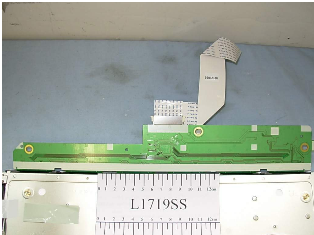
FIGURE 13 LCD MONITOR (M/N: L1719SS) LCD PANEL MAIN BOARD (BACK VIEW)
