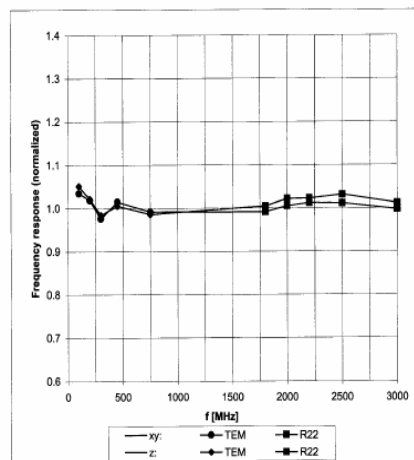
Frequency Response of H-Field (TEM-Cell: if110, Waveguide R22)
