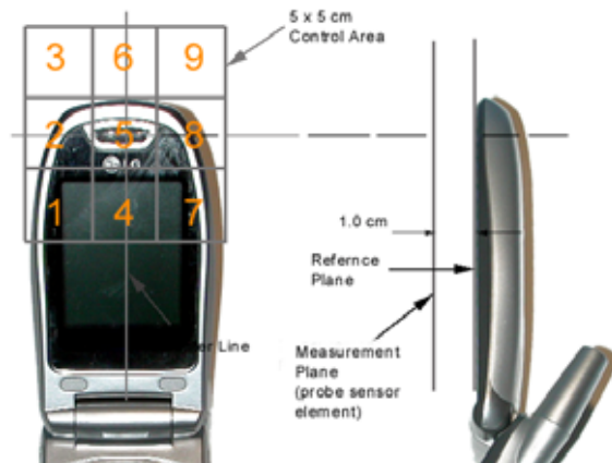
Figure 13 E/H-Field Emissions Test Setup Diagram
