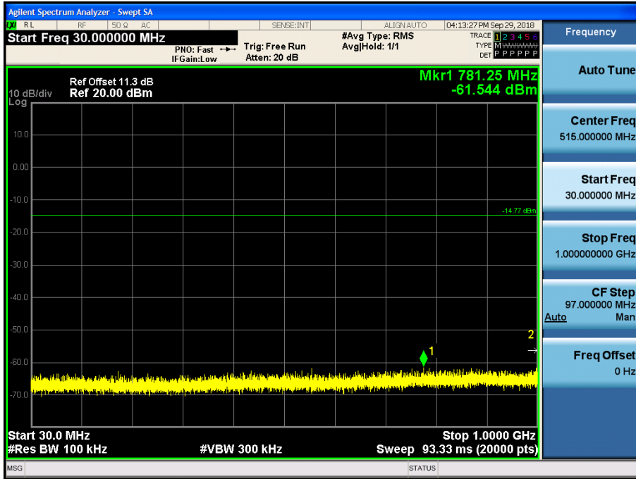
Conducted Spurious Emission (802.11n_Ch.6)
