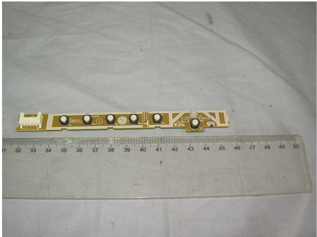
FIGURE 10 LCD MONITOR (M/N: E2241SX) KEY BOARD (COMPONENT SIDE)
