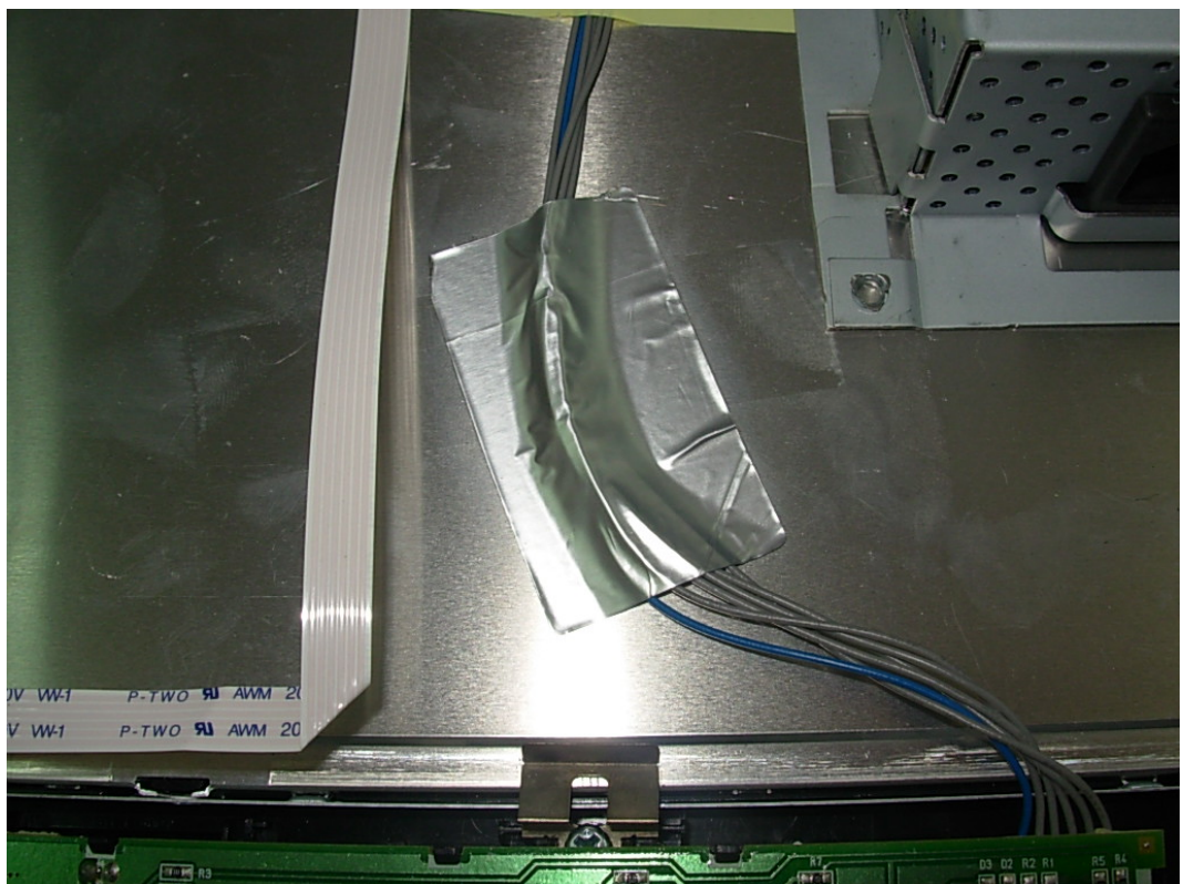
FIGURE 13 LCD MONITOR (M/N: E2241SX) DEBUG #2
