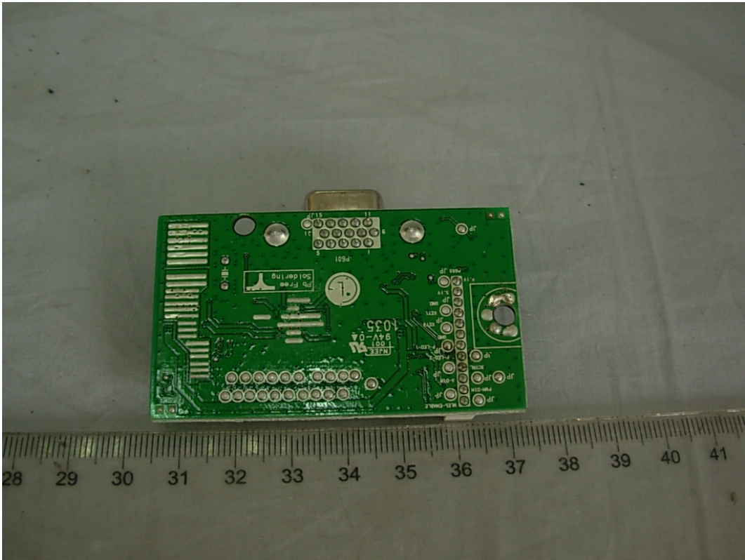
FIGURE 8 LCD MONITOR (M/N: E2241SX) MAIN BOARD (SOLDERED SIDE)
