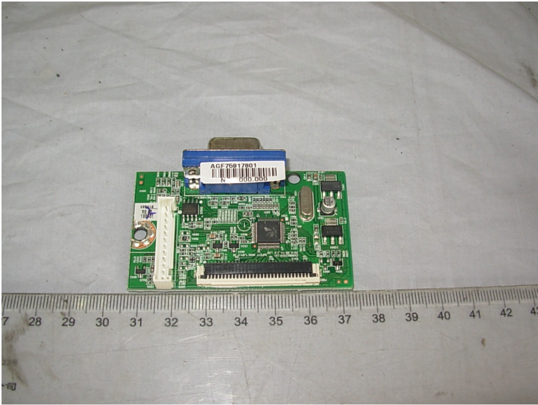
FIGURE 7 LCD MONITOR (M/N: E2241SX) MAIN BOARD (COMPONENT SIDE)
