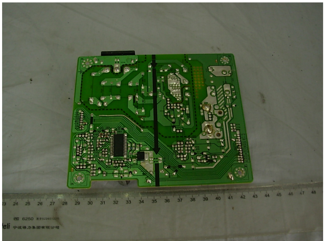
FIGURE 6 LCD MONITOR (M/N: E2241SX) POWER BOARD (SOLDERED SIDE)
