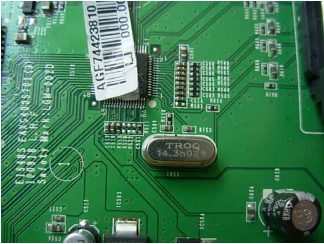
FIGURE 5 LCD MONITOR (M/N: E1948SX) CHIP & CRYSTAL ON MAIN BOARD
