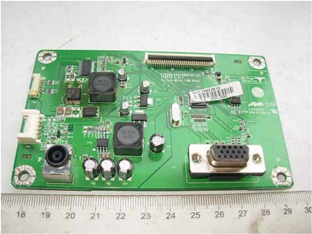
FIGURE 3 LCD MONITOR (M/N: E1948SX) MAIN BOARD (COMPONENT SIDE)
