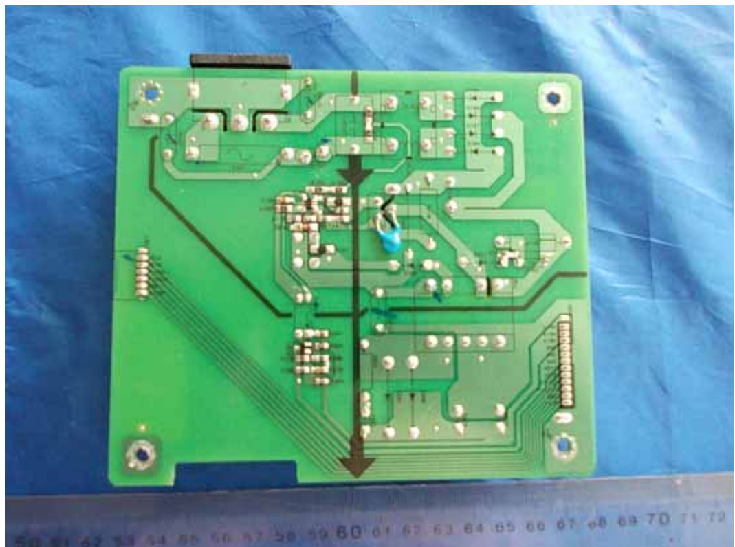
FIGURE 5 LCD MONITOR (M/N: E1641CX) POWER BOARD (COMPONENT SIDE)
