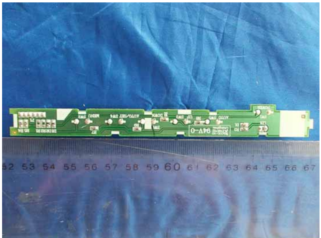
FIGURE 10 LCD MONITOR (M/N: E1641CX) KEY BOARD (SOLDERED SIDE)
