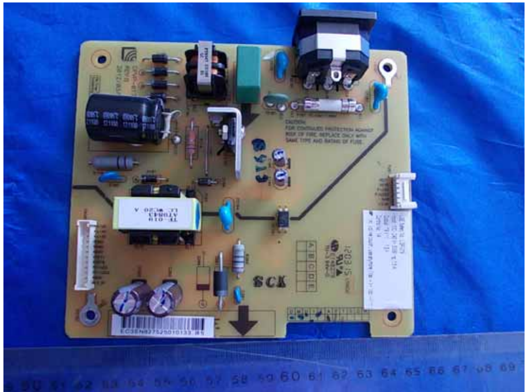
FIGURE 4 LCD MONITOR (M/N: E1641CX) POWER BOARD (COMPONENT SIDE)
