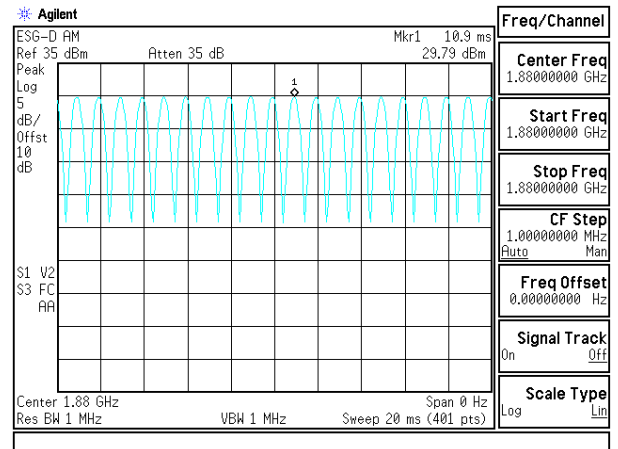
Figure 25 80% AM Signal
