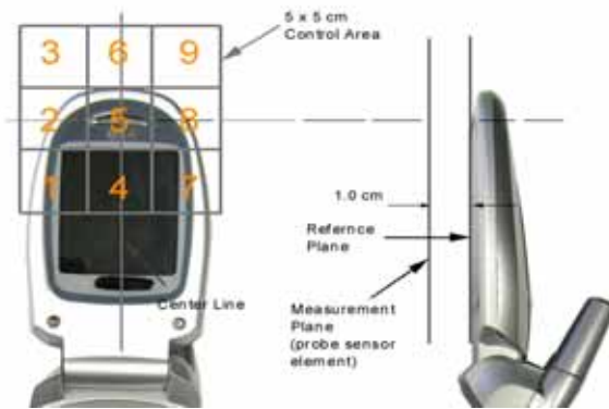
Figure 13 E/H-Field Emissions Test Setup Diagram
