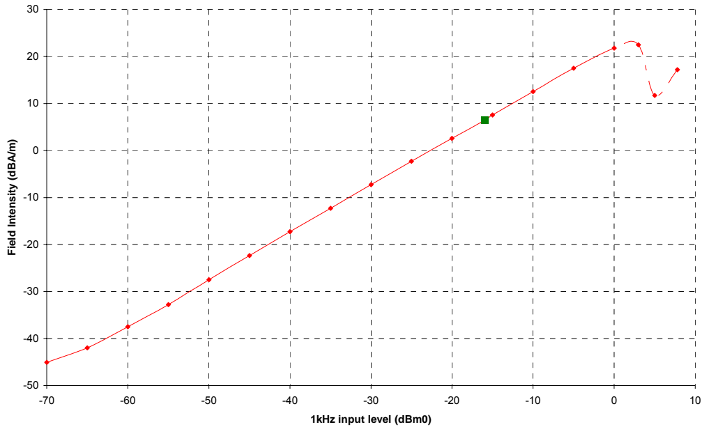
1kHz Tone Pass-through
