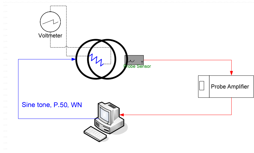
Figure 5-1 Validation Setup with Helmholtz Coil
