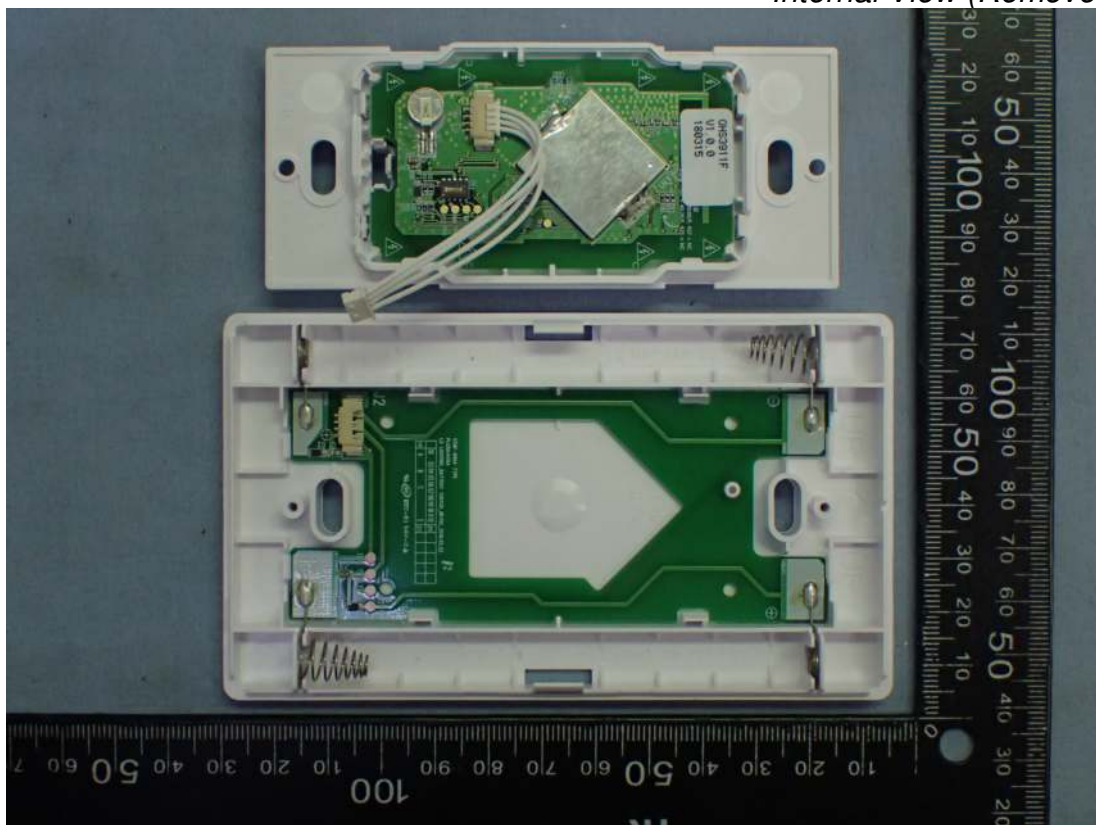
Figure 6 Internal View (Removed Cover)
