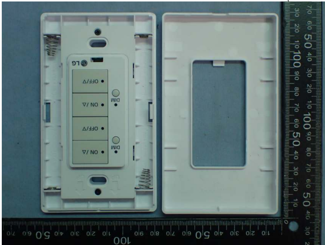
Figure 5 Internal View (Removed Cover)
