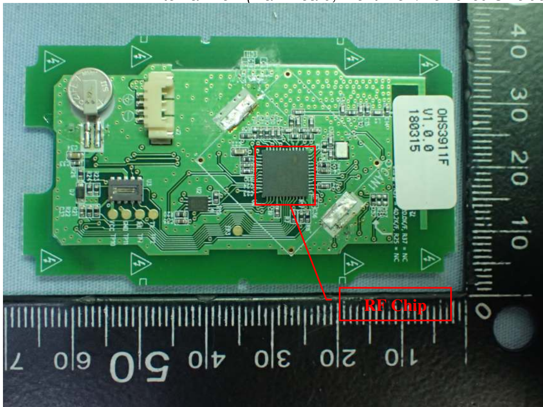
Internal View (Main Board, Front View/Removed Shielded Case)
