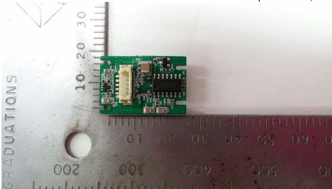
Internal View (Main Board, Front View)
