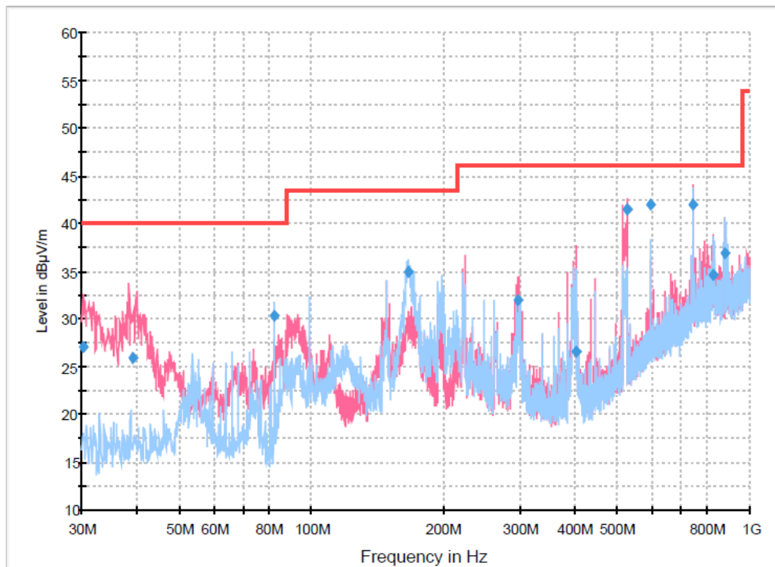
RE_below 1GHz
