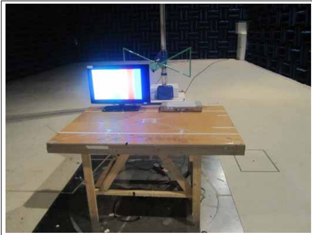
< SIDE HDMI MODE_30MHz-1GHz >
