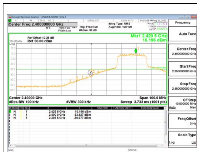
LOW CHANNEL 4 BANDEDGE ANT 4
