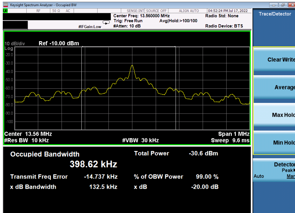
Plot 7-5. 20dB and 99% Bandwidth Plot (Reader 10% ASK 1 out of 256)
