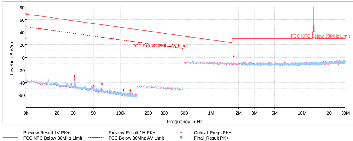
Plot 7-8. Radiated Spurious Emissions 9kHz – 30MHz (CE A 106kbps, with AC/DC Adapter and Magnetic Charger)
