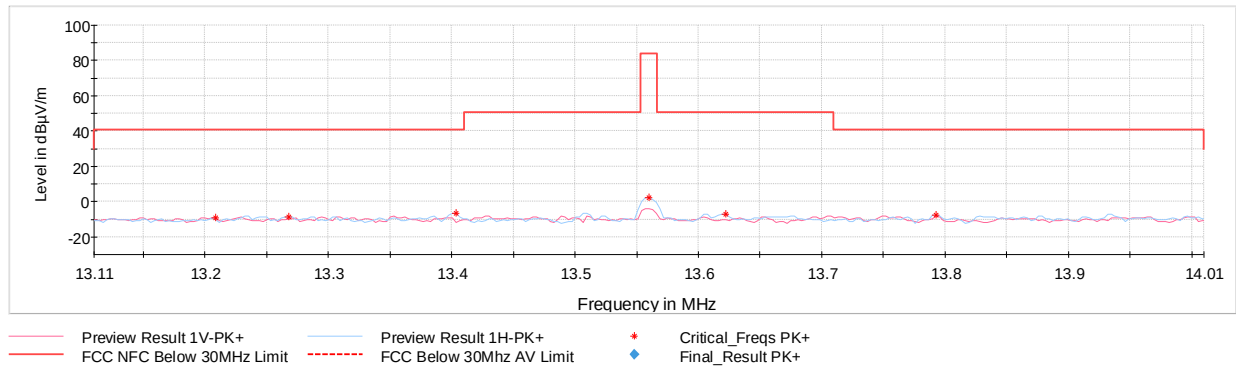
Plot 7-7. In Band Radiated Spurious Emissions (Reader A 848kbps, AC/DC Adapter and Magnetic Charger)
