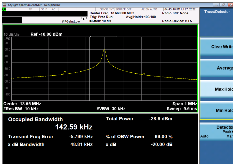
Plot 7-3. 20dB and 99% Bandwidth Plot (CE F 212kbps)
