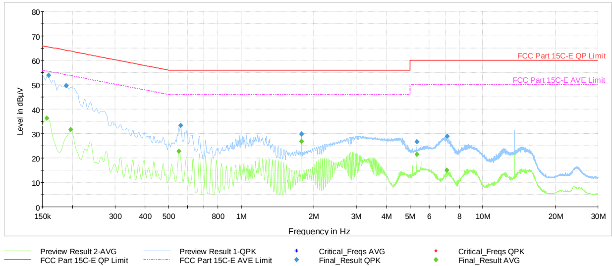
Plot 7-12. AC Line-Conducted Plot (L1, CE A 106kbps, with AC/DC Adapter and Magnetic Charger)
