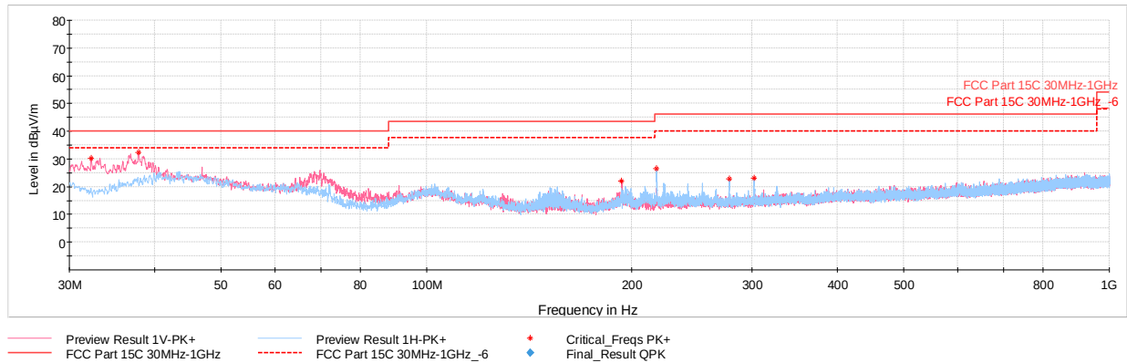
Plot 7-10. Radiated Spurious Emissions 30MHz – 1GHz (CE A 106kbps, with AC/DC Adapter and Magnetic Charger)
