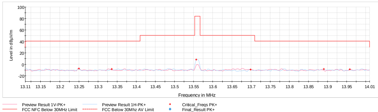
Plot 7-6. In Band Radiated Spurious Emissions (CE A 106kbps, with AC/DC Adapter and Magnetic Charger)
