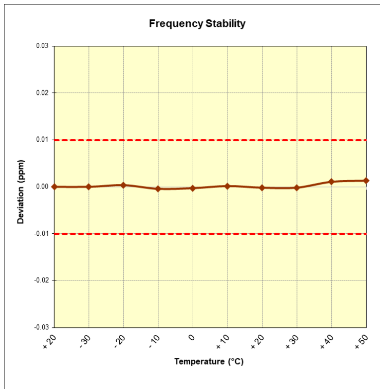
Figure 7-3. Frequency Stability Plot (CE A 106kbps)
