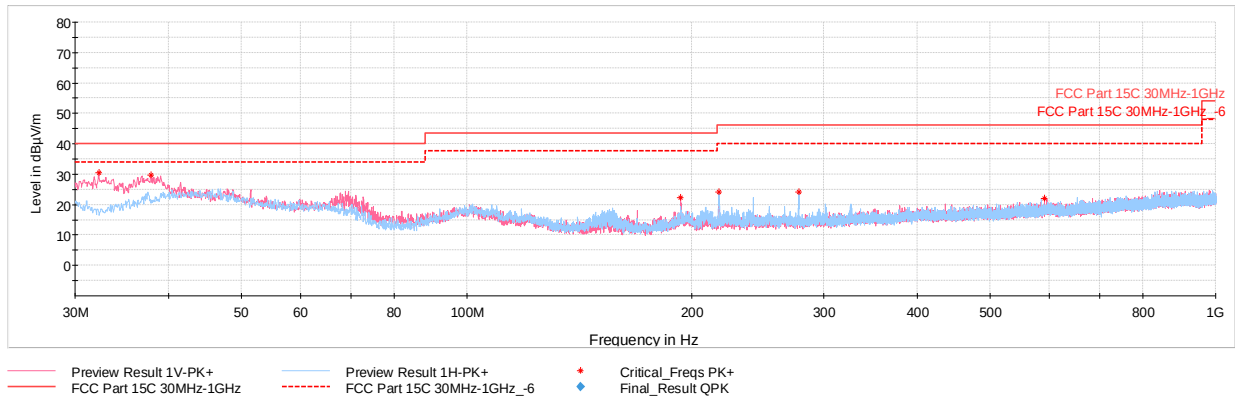
Plot 7-11. Radiated Spurious Emissions 30MHz – 1GHz (Reader A 848kbps, with AC/DC Adapter and Magnetic Charger)
