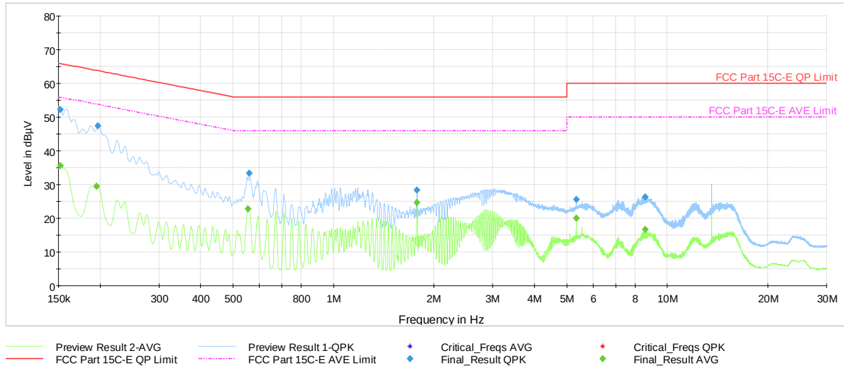
Plot 7-14. AC Line-Conducted Plot (L1, Reader A 848kbps, with Laptop and Magnetic Charger)
