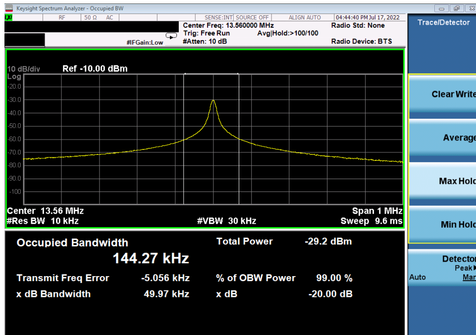
Plot 7-2. 20dB and 99% Bandwidth Plot (CE B 848kbps)
