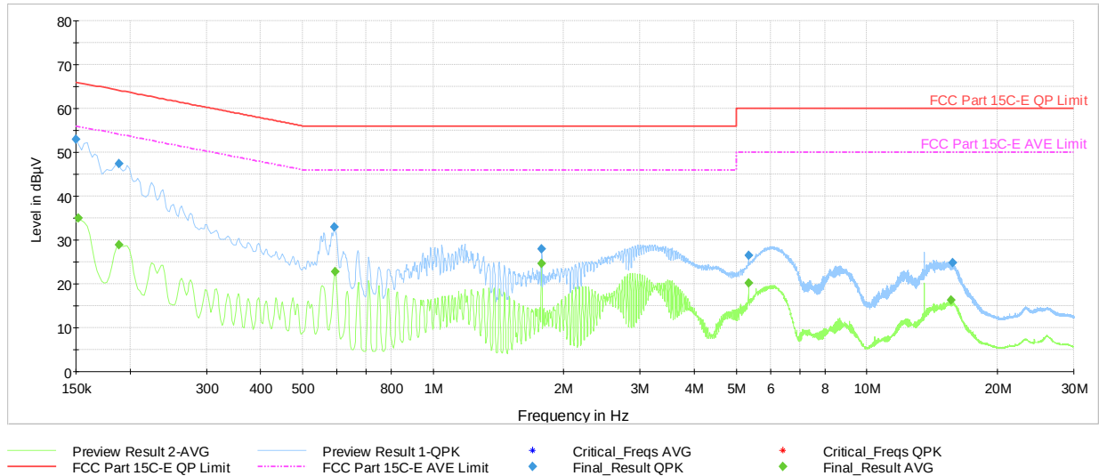
Plot 7-15. AC Line-Conducted Plot (N, Reader A 848kbps, with Laptop and Magnetic Charger)
