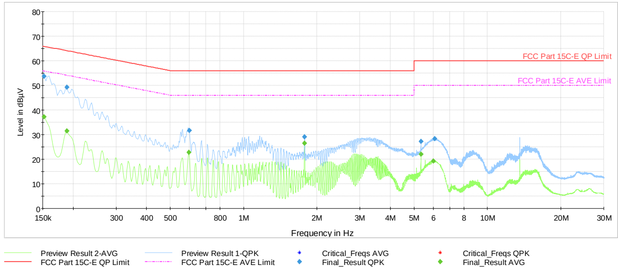
Plot 7-13. AC Line-Conducted Plot (N, CE A 106kbps, with AC/DC Adapter and Magnetic Charger)
