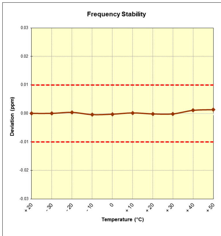
Figure 7-4. Frequency Stability Plot (Reader 100% ASK 1 out of 256)
