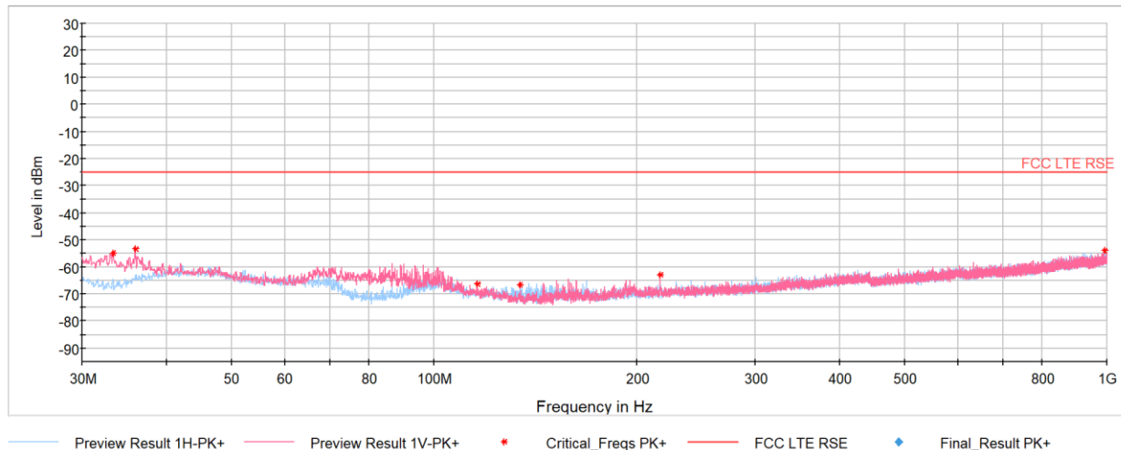
Plot 7-65. Antenna FCM Radiated Spurious Emissions -Simultaneous Transmission 30MHz – 1GHz
