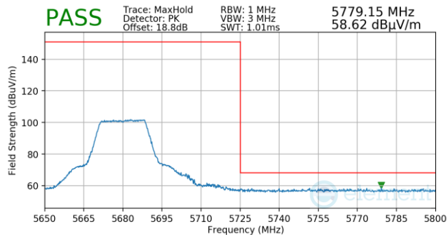
Plot 7-49. FCM (Pk, Ch.136, 802.11n, MCS0)
