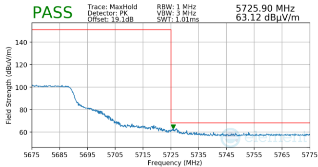
Plot 7-50. FCM (Pk, Ch.136, 802.11n, MCS7)
