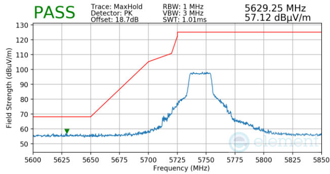
Plot 7-54. FCM (Pk, Ch.149, 802.11n, MCS7)
