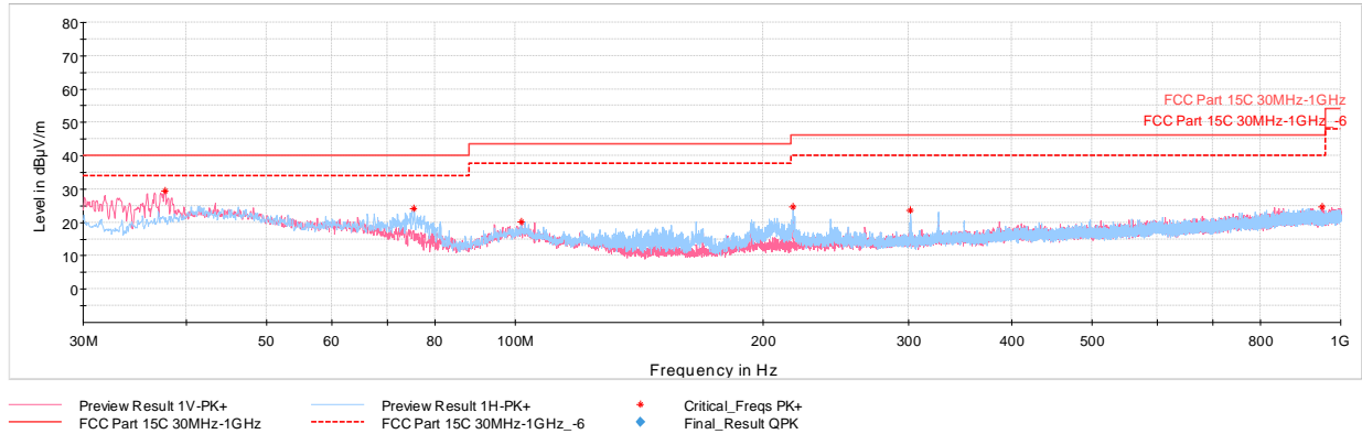
Plot 7-58. Radiated Spurious Emissions – Simultaneous Transmission 30MHz – 1GHz, with AC/DC Adapter)
