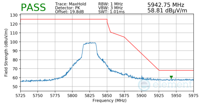
Plot 7-56. FCM (Pk, Ch.165, 802.11n, MCS7)
