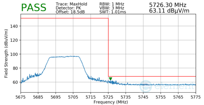
Plot 7-51. FCM (Pk, Ch.140, 802.11n, MCS0)
