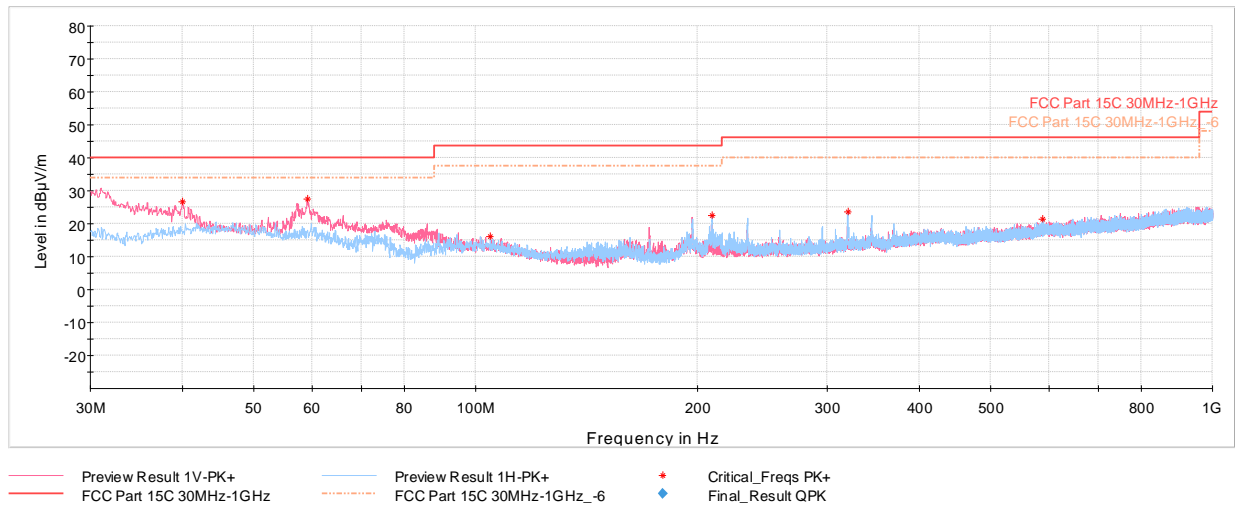
Plot 7-57. Radiated Spurious Emissions below 1GHz 802.11n, Ch.40 with AC/DC Adapter & Magnetic Charger
