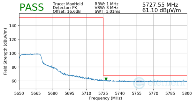
Plot 7-48. FCM (Pk & Avg, Ch.132, 802.11n, MCS7)
