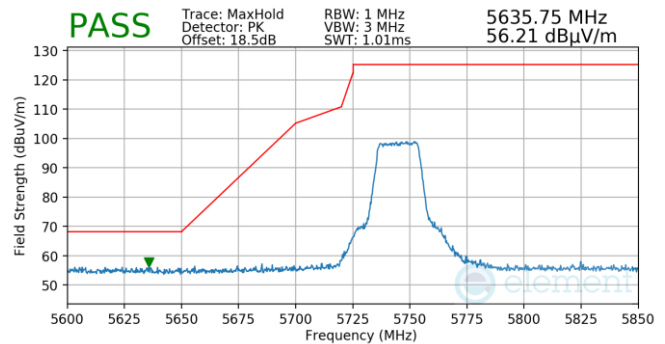
Plot 7-53. FCM (Pk, Ch.149, 802.11n, MCS0)
