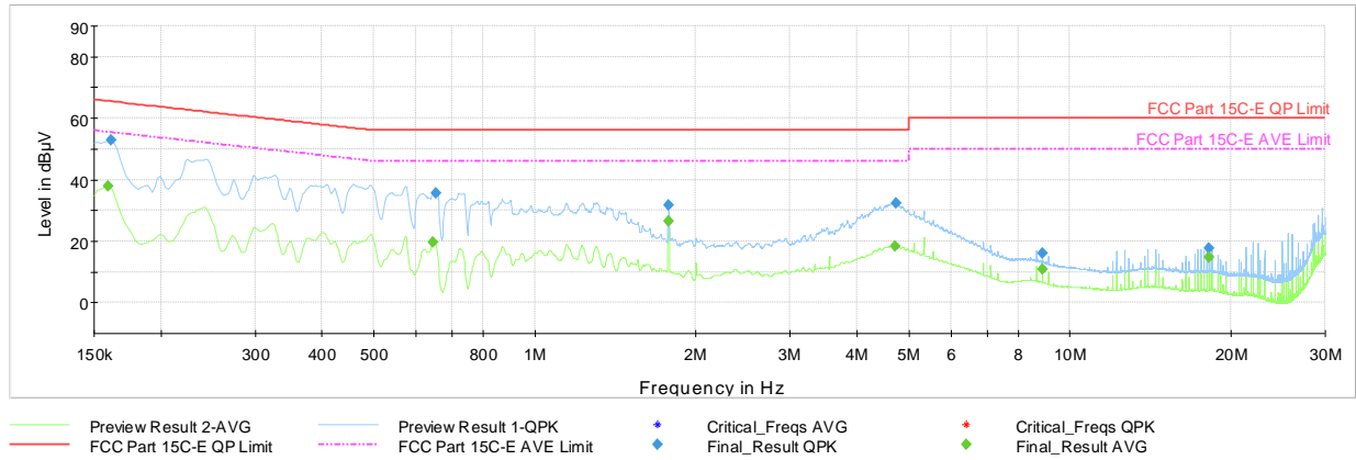
Plot 7-59. AC Line Conducted Plot with 802.11n- Ch.40 (L1), with Laptop & Magnetic Charger
