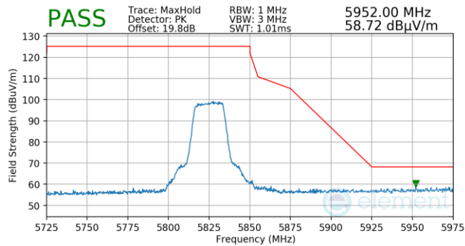
Plot 7-55. FCM (Pk, Ch.165, 802.11n, MCS0)
