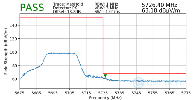
Plot 7-52. FCM (Pk, Ch.140, 802.11n, MCS7)
