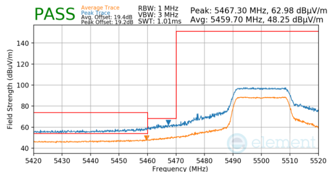
Plot 7-47. FCM (Pk & Avg, Ch.100, 802.11n, MCS7)
