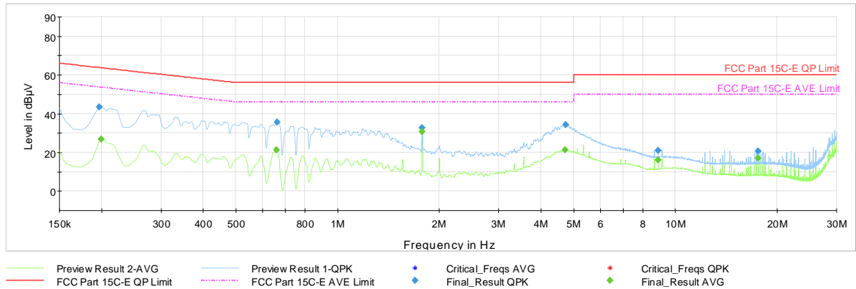
Plot 7-60. AC Line Conducted Plot with 802.11n– Ch.40 (N), with Laptop & Magnetic Charger
