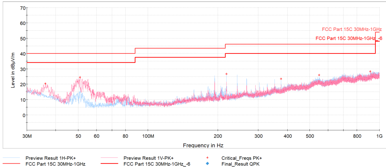
Plot 7-42. Radiated Spurious Emissions below 1GHz – Simultaneous Transmission
