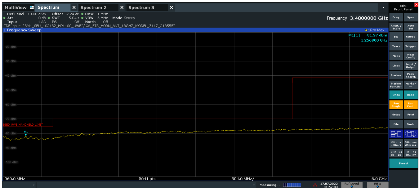
Plot 7-27. ISD Radiated Spurious Emission 960-6000MHz (Ch. 9, Config 0, Payload 125 Ant. Pol. H)
