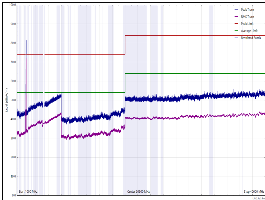
Figure 3 - 2412 MHz (CH1), HT20, Core 0 + Core 1 and U-NII-1 - 5200 MHz (CH40), HT20, Core 0 + Core 1 and 2402 MHz (CH0), DH5, iPA, Core 2, 1 GHz to 40 GHz, Horizontal
