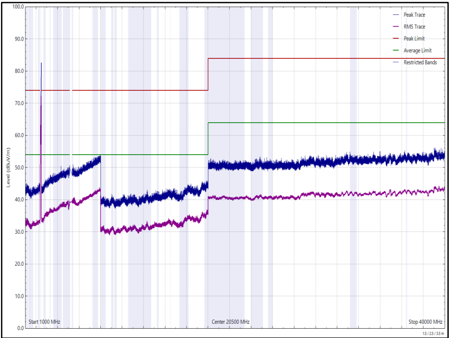
Figure 5 - 2412 MHz (CH1), HT20, Core 0 + Core 1 and U-NII-1 - 5200 MHz (CH40), HT20, Core 0 + Core 1 and 2402 MHz (CH0), DH5, iPA, Core 2, 1 GHz to 40 GHz, Vertical
