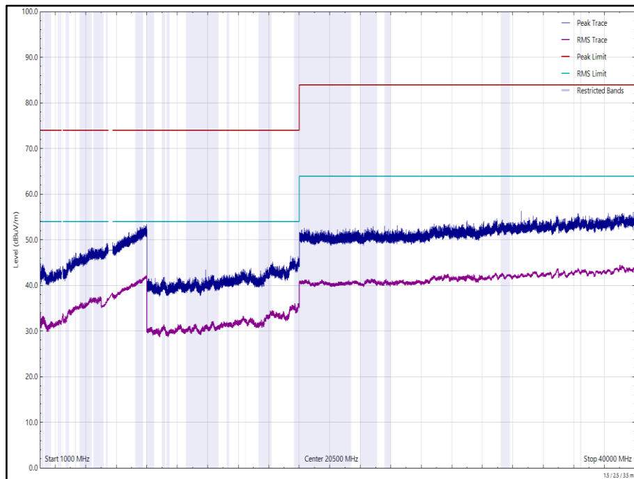
Figure 15- 2472 MHz (CH13), HT20, Core 0 + Core 1 and U-NII-2C - 5680 MHz (CH136), HT20, CDD, Core 0 + Core 1, 1 GHz to 40 GHz, Horizontal
