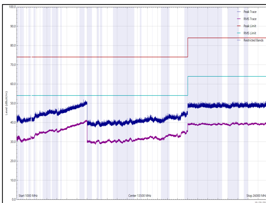
Figure 163 - 2437 MHz (CH6), 802.11b, Core 0, 1 GHz to 26 GHz, Horizontal
