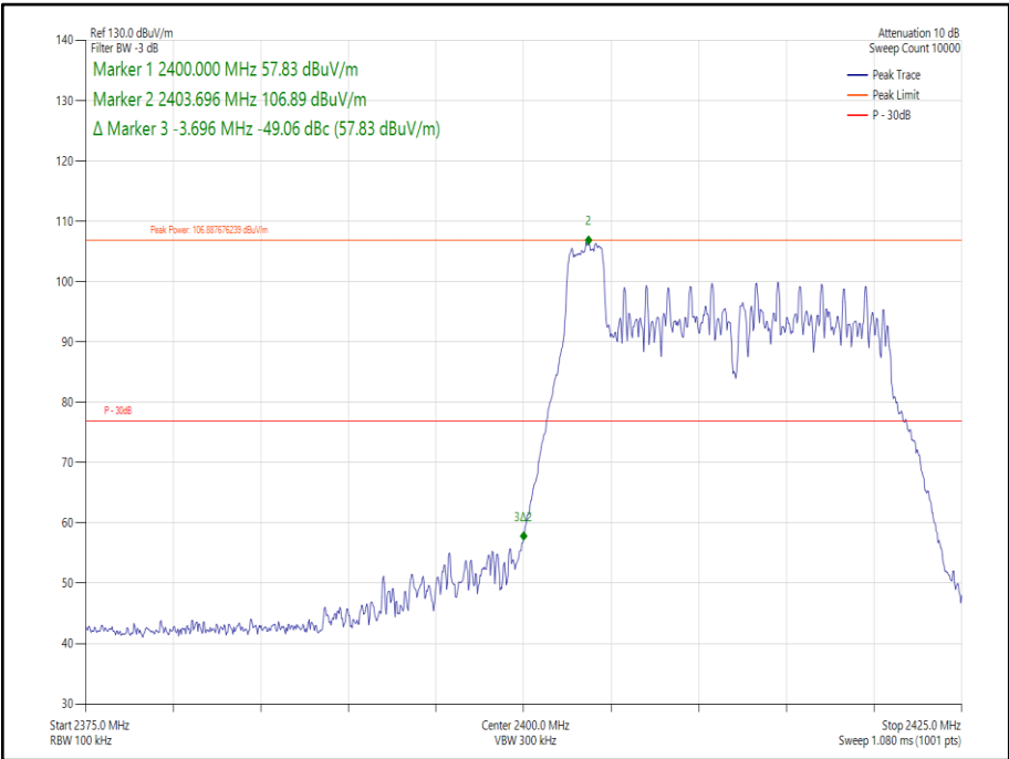
Figure 188- 802.11ax HE20, Core 0, 26-0 - 2412 MHz Band Edge Frequency 2400 MHz
