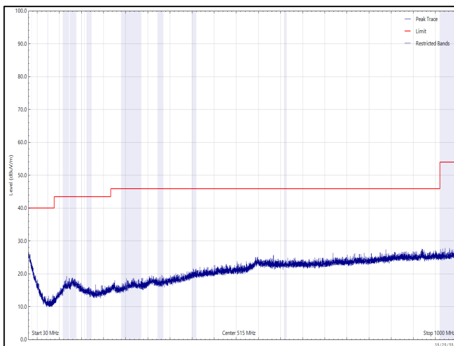
Figure 162 - 2437 MHz (CH6), 802.11b, Core 0, 30 MHz to 1 GHz, Horizontal (Peak)
