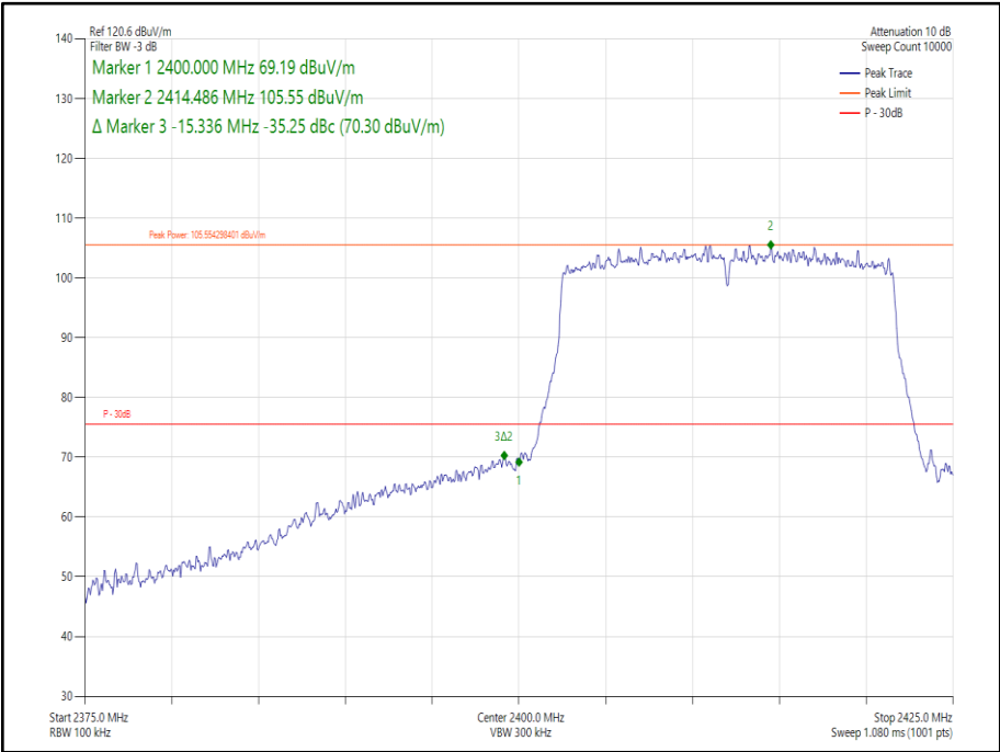
Figure 187- 802.11ax HE20, Core 0, SU - 2412 MHz Band Edge Frequency 2400 MHz
