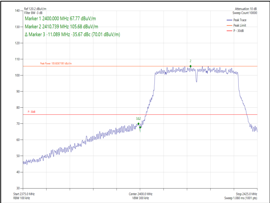
Figure 186- 802.11n HT20, Core 0 - 2412 MHz Band Edge Frequency 2400 MHz
