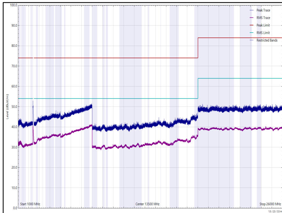
Figure 139 - 2437 MHz (CH6), HT20, CDD, Core 0 + Core 1, 1 GHz to 26 GHz, Horizontal
