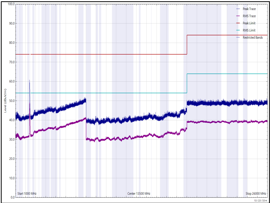
Figure 136 - 2412 MHz (CH1), HT20, CDD, Core 0 + Core 1, 1 GHz to 26 GHz, Horizontal
