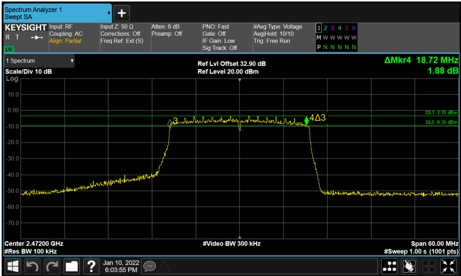
Figure 78 - Core 0 (A) 2472 MHz (CH13) 6 dB Bandwidth
