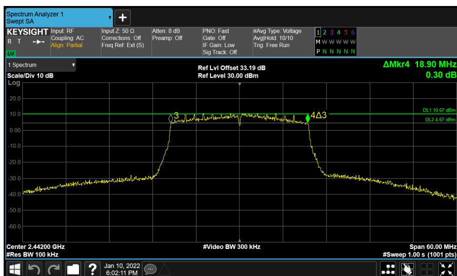
Figure 76 - Core 1 (B) 2442 MHz (CH7) 6 dB Bandwidth
