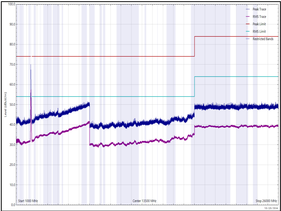
Figure 137 - 2412 MHz (CH1), HT20, CDD, Core 0 + Core 1, 1 GHz to 26 GHz, Vertical
